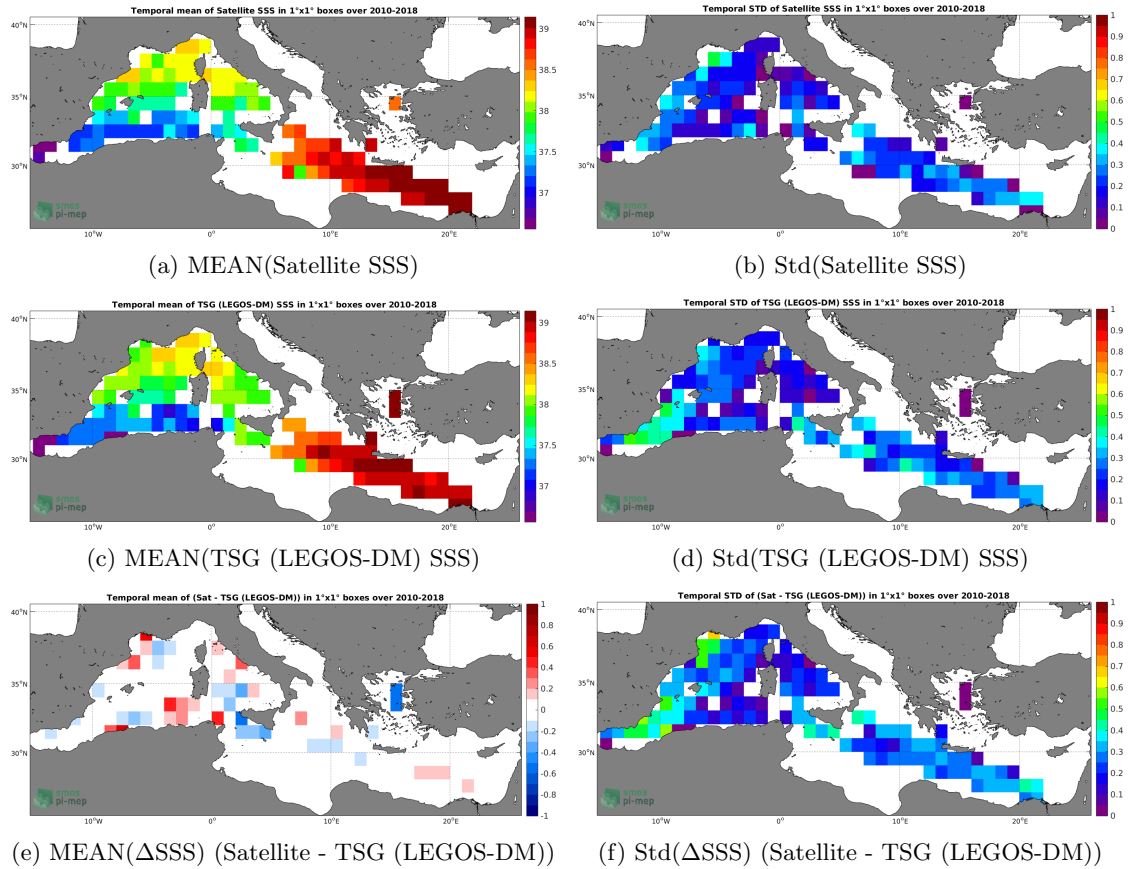
Figure 6: Temporal mean (left) and Std (right) of SSS from CCI L4 Merged-OI v2.31 - 7-day running (ESA) (top), TSG (LEGOS-DM) (middle), and of \Delta SSS (Satellite - TSG (LEGOS-DM)). Only match-up pairs are used to generate these maps.
