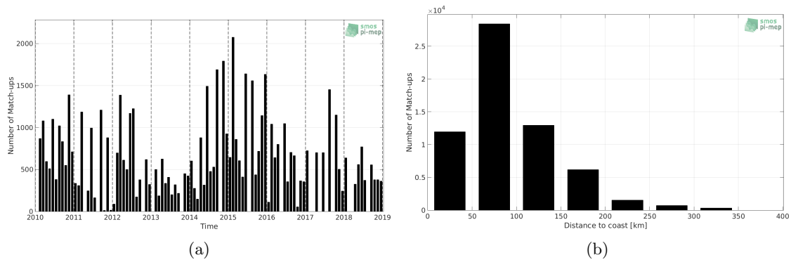
Figure 1: Number of match-ups between TSG (LEGOS-DM) and CCI L4 Merged-OI v2.31 - 7-day running (ESA) SSS as a function of time (a) and as function of the distance to coast (b) over the Mediterranean Sea Pi-MEP region and for the full satellite product period.
