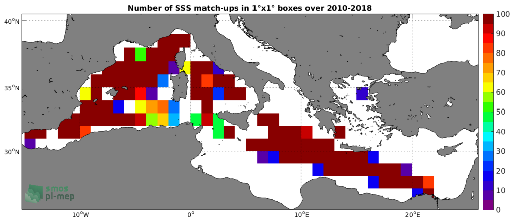
Figure 4: Number of SSS match-ups between TSG (LEGOS-DM) SSS and the CCI L4 Merged-OI v2.31 - 7-day running (ESA) SSS product for the Mediterranean Sea Pi-MEP region over 1^\circ \times 1^\circ boxes and for the full satellite product period.
