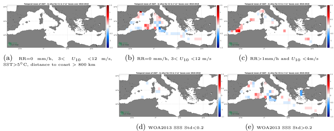
Figure 12: Temporal mean gridded over spatial boxes of size 1^\circ \times 1^\circ of \Delta SSS (CCI L4 Merged-OI v2.31 - 7-day running (ESA) - TSG (LEGOS-DM)) for 5 different subdatasets corresponding to:RR=0 mm/h, 3 < U_{10} < 12 m/s, SST >5^\circ C, distance to coast > 800 km (a), RR=0 mm/h, 3 < U_{10} < 12 m/s (b), RR >1 mm/h and U_{10} < 4 m/s (c), WOA2013 SSS Std <0.2 (d), WOA2013 SSS Std >0.2 (e).
