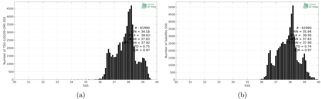
Figure 2: Histograms of SSS from TSG (LEGOS-DM) (a) and CCI L4 Merged-OI v2.31 - 7-day running (ESA) (b) considering all match-up pairs per bins of 0.1 over the Mediterranean Sea Pi-MEP region and for the full satellite product period.
