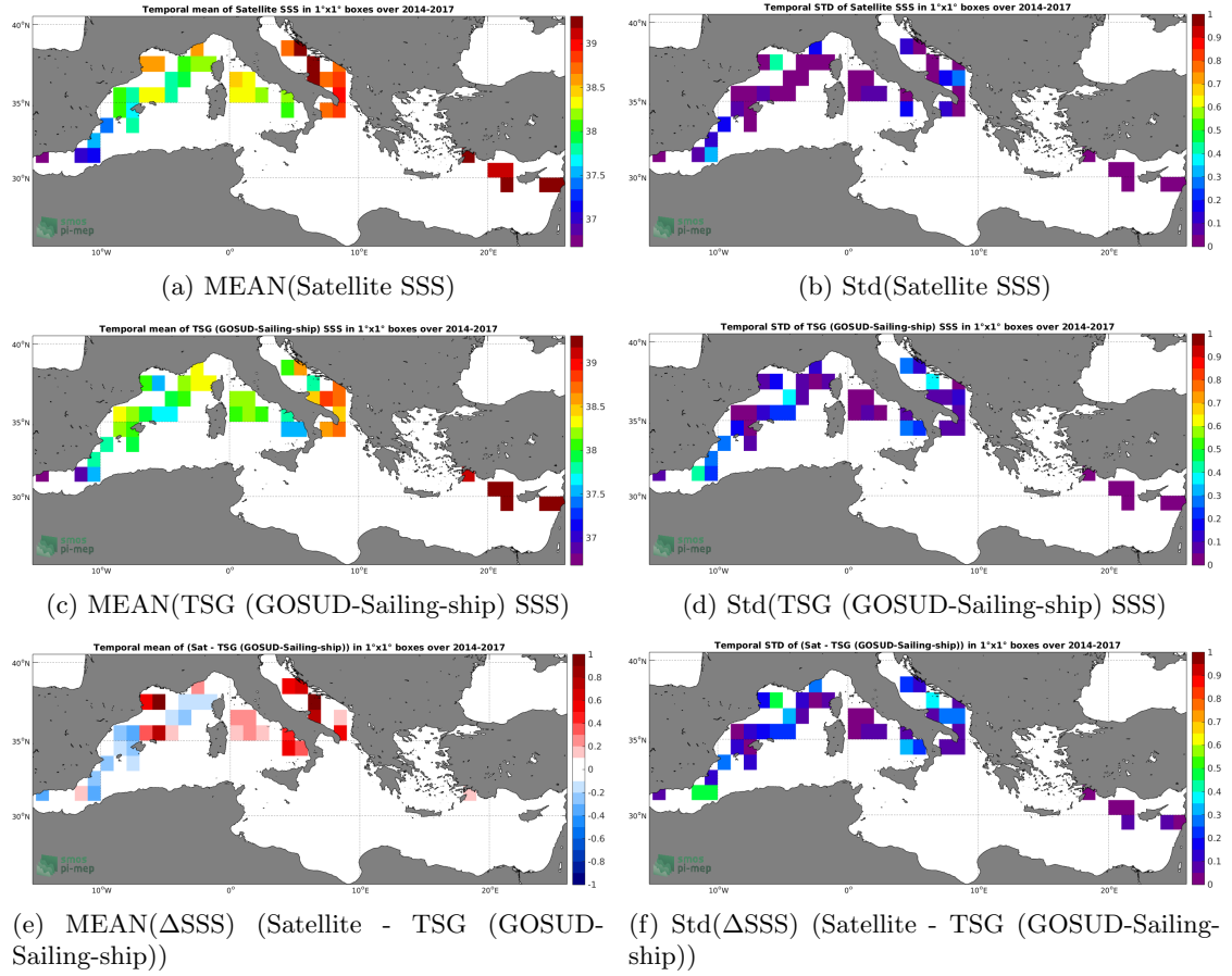
Figure 6: Temporal mean (left) and Std (right) of SSS from CCI L4 Merged-OI v2.31 - 7-day running (ESA) (top), TSG (GOSUD-Sailing-ship) (middle), and of \Delta SSS (Satellite - TSG (GOSUD-Sailing-ship)). Only match-up pairs are used to generate these maps.
