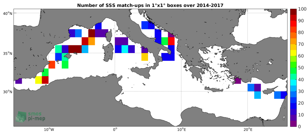
Figure 4: Number of SSS match-ups between TSG (GOSUD-Sailing-ship) SSS and the CCI L4 Merged-OI v2.31 - 7-day running (ESA) SSS product for the Mediterranean Sea Pi-MEP region over 1°x1° boxes and for the full satellite product period.
