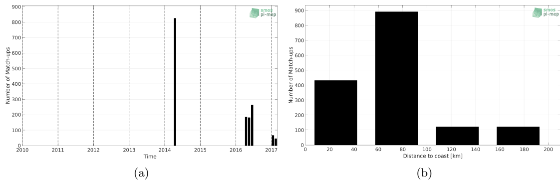
Figure 1: Number of match-ups between TSG (GOSUD-Sailing-ship) and CCI L4 Merged-OI v2.31 - 7-day running (ESA) SSS as a function of time (a) and as function of the distance to coast (b) over the Mediterranean Sea Pi-MEP region and for the full satellite product period.
