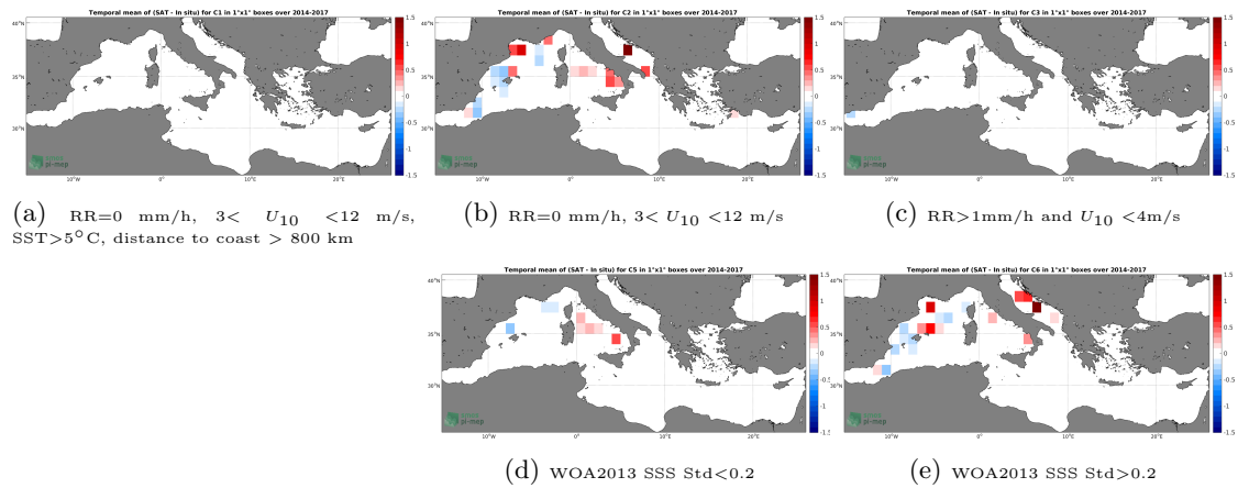
Figure 12: Temporal mean gridded over spatial boxes of size 1^\circ \times 1^\circ of \Delta SSS (CCI L4 Merged-OI v2.31 - 7-day running (ESA) - TSG (GOSUD-Sailing-ship)) for 5 different subdatasets corresponding to:RR=0 mm/h, 3 < U_{10} < 12 m/s, SST >5^\circ\text{C} , distance to coast > 800 km (a), RR=0 mm/h, 3 < U_{10} < 12 m/s (b), RR >1 mm/h and U_{10} < 4 m/s (c), WOA2013 SSS Std <0.2 (d), WOA2013 SSS Std >0.2 (e).
