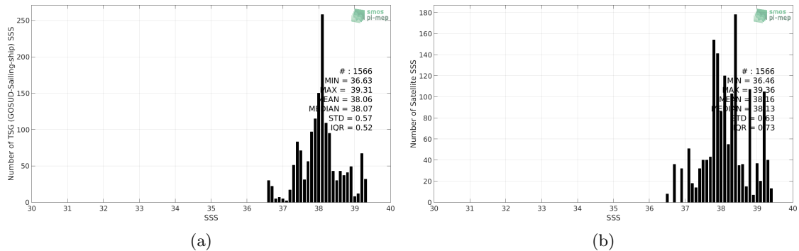
Figure 2: Histograms of SSS from TSG (GOSUD-Sailing-ship) (a) and CCI L4 Merged-OI v2.31 - 7-day running (ESA) (b) considering all match-up pairs per bins of 0.1 over the Mediterranean Sea Pi-MEP region and for the full satellite product period.
