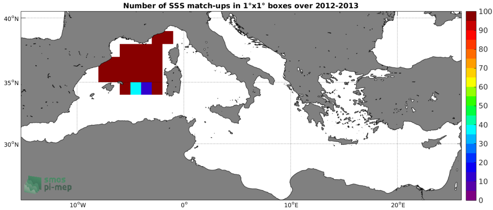
Figure 3: Number of SSS match-ups between Surface drifters SSS and the CCI L4 Merged-OI v2.31 - 7-day running (ESA) SSS product for the Mediterranean Sea Pi-MEP region over 1°x1° boxes and for the full satellite product period.
