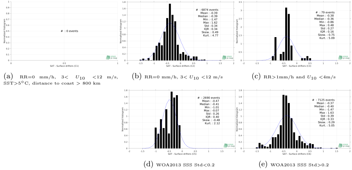
Figure 12: Normalized histogram of \Delta\text{SSS} (CCI L4 Merged-OI v2.31 - 7-day running (ESA) - Surface drifters) for 5 different subdatasets corresponding to: RR=0 mm/h, 3 < U_{10} < 12 m/s, SST > 5^\circ\text{C} , distance to coast > 800 km (a), RR=0 mm/h, 3 < U_{10} < 12 m/s (b), RR > 1\text{mm/h} and U_{10} < 4\text{m/s} (c), WOA2013 SSS Std < 0.2 (d), WOA2013 SSS Std > 0.2 (e).
