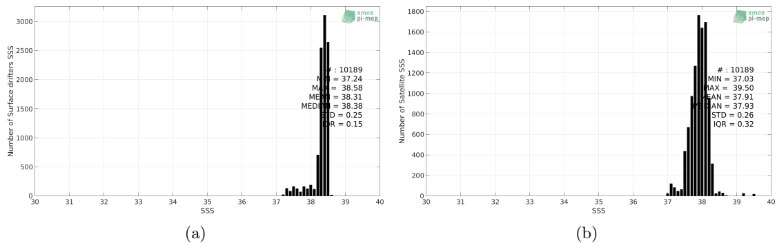
Figure 2: Histograms of SSS from Surface drifters (a) and CCI L4 Merged-OI v2.31 - 7-day running (ESA) (b) considering all match-up pairs per bins of 0.1 over the Mediterranean Sea Pi-MEP region and for the full satellite product period.
