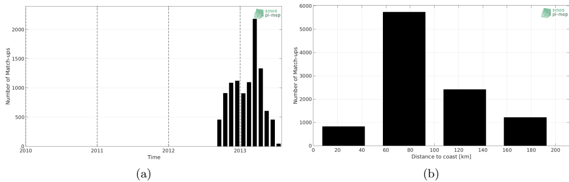
Figure 1: Number of match-ups between Surface drifters and CCI L4 Merged-OI v2.31 - 7-day running (ESA) SSS as a function of time (a) and as function of the distance to coast (b) over the Mediterranean Sea Pi-MEP region and for the full satellite product period.
