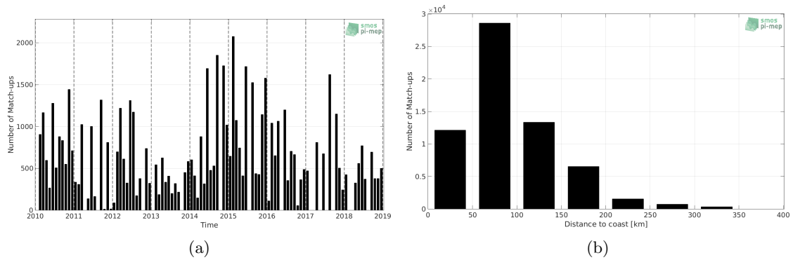
Figure 1: Number of match-ups between TSG (LEGOS-DM) and CCI L4 Merged-OI v2.31 - 30-day running (ESA) SSS as a function of time (a) and as function of the distance to coast (b) over the Mediterranean Sea Pi-MEP region and for the full satellite product period.
