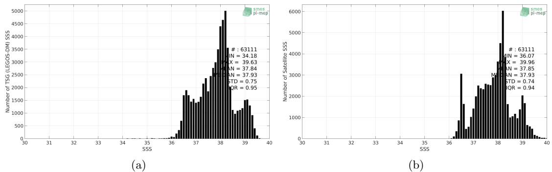
Figure 2: Histograms of SSS from TSG (LEGOS-DM) (a) and CCI L4 Merged-OI v2.31 - 30-day running (ESA) (b) considering all match-up pairs per bins of 0.1 over the Mediterranean Sea Pi-MEP region and for the full satellite product period.
