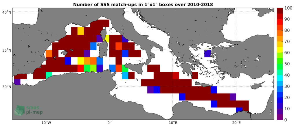
Figure 4: Number of SSS match-ups between TSG (LEGOS-DM) SSS and the CCI L4 Merged-OI v2.31 - 30-day running (ESA) SSS product for the Mediterranean Sea Pi-MEP region over 1^\circ \times 1^\circ boxes and for the full satellite product period.
