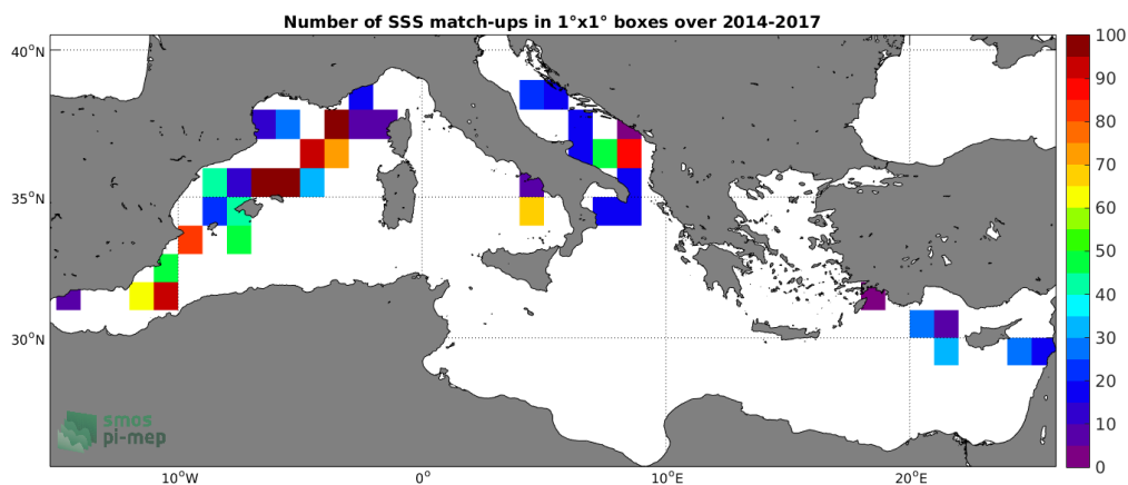
Figure 4: Number of SSS match-ups between TSG (GOSUD-Sailing-ship) SSS and the CCI SSS L4 Merged-OI v2.31 - 30-day running (ESA) SSS product for the Mediterranean Sea Pi-MEP region over 1°x1° boxes and for the full satellite product period.
