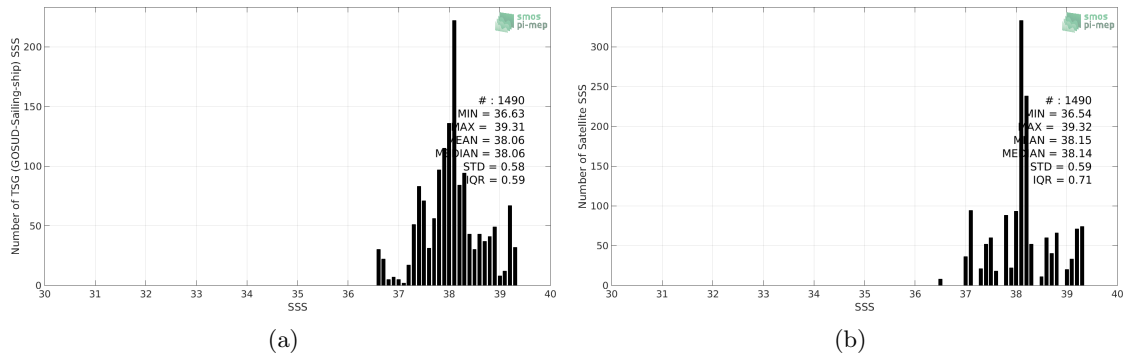
Figure 2: Histograms of SSS from TSG (GOSUD-Sailing-ship) (a) and CCI SSS L4 Merged-OI v2.31 - 30-day running (ESA) (b) considering all match-up pairs per bins of 0.1 over the Mediterranean Sea Pi-MEP region and for the full satellite product period.
