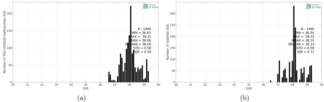
Figure 2: Histograms of SSS from TSG (GOSUD-Sailing-ship) (a) and CCI L4 Merged-OI v2.31 - 30-day running (ESA) (b) considering all match-up pairs per bins of 0.1 over the Mediterranean Sea Pi-MEP region and for the full satellite product period.
