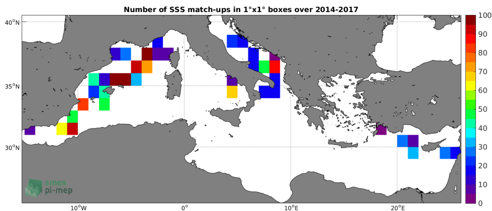
Figure 4: Number of SSS match-ups between TSG (GOSUD-Sailing-ship) SSS and the CCI L4 Merged-OI v2.31 - 30-day running (ESA) SSS product for the Mediterranean Sea Pi-MEP region over 1°x1° boxes and for the full satellite product period.
