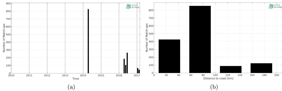
Figure 1: Number of match-ups between TSG (GOSUD-Sailing-ship) and CCI L4 Merged-OI v2.31 - 30-day running (ESA) SSS as a function of time (a) and as function of the distance to coast (b) over the Mediterranean Sea Pi-MEP region and for the full satellite product period.
