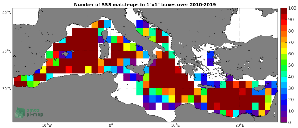
Figure 4: Number of SSS match-ups between Argon SSS and the CCI L4 Merged-OI v2.31 - 30-day running (ESA) SSS product for the Mediterranean Sea Pi-MEP region over 1°x1° boxes and for the full satellite product period.
