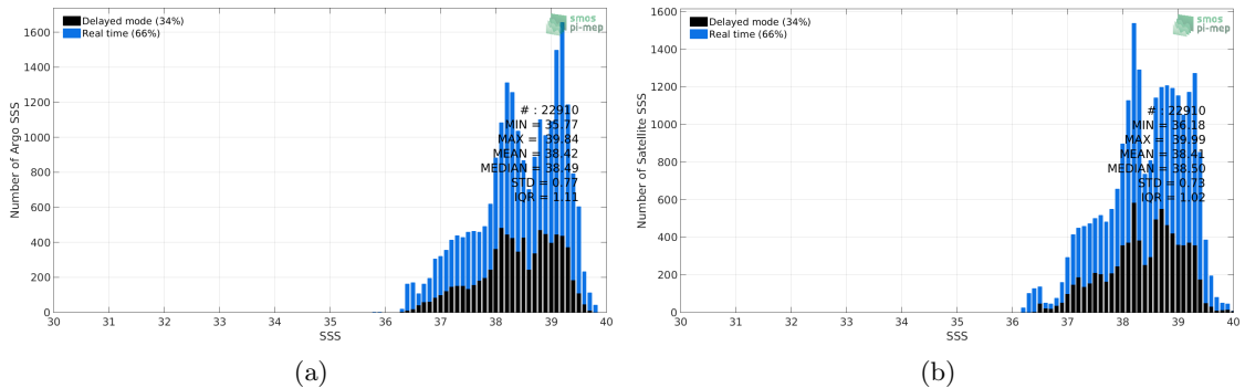
Figure 2: Histograms of SSS from Argo (a) and CCI L4 Merged-OI v2.31 - 30-day running (ESA) (b) considering all match-up pairs per bins of 0.1 over the Mediterranean Sea Pi-MEP region and for the full satellite product period.
