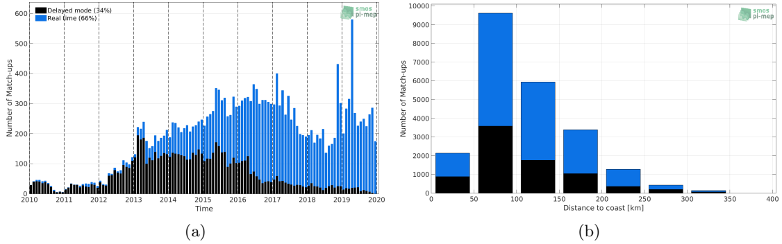
Figure 1: Number of match-ups between Argo and CCI L4 Merged-OI v2.31 - 30-day running (ESA) SSS as a function of time (a) and as function of the distance to coast (b) over the Mediterranean Sea Pi-MEP region and for the full satellite product period.
