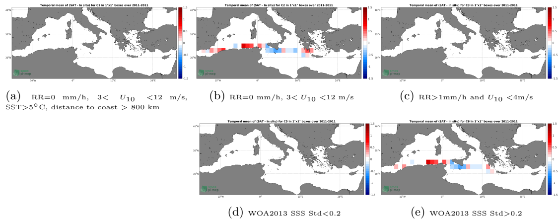
Figure 12: Temporal mean gridded over spatial boxes of size 1^{\circ}\times 1^{\circ} of \Delta\text{SSS} (CCI L4 Merged-OI v1.8 - 7-day running (ESA) - TSG-SAMOS) for 5 different subdatasets corresponding to:RR=0 mm/h, 3 < U_{10} < 12 m/s, SST > 5^{\circ}\text{C} , distance to coast > 800 km (a), RR=0 mm/h, 3 < U_{10} < 12 m/s (b), RR > 1 mm/h and U_{10} < 4 m/s (c), WOA2013 SSS Std < 0.2 (d), WOA2013 SSS Std > 0.2 (e).
