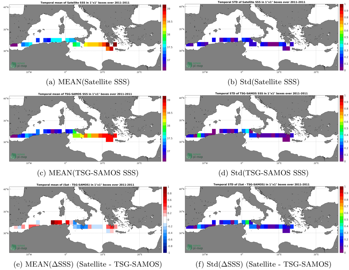
Figure 6: Temporal mean (left) and Std (right) of SSS from CCI L4 Merged-OI v1.8 - 7-day running (ESA) (top), TSG-SAMOS (middle), and of \Delta SSS (Satellite - TSG-SAMOS). Only match-up pairs are used to generate these maps.
