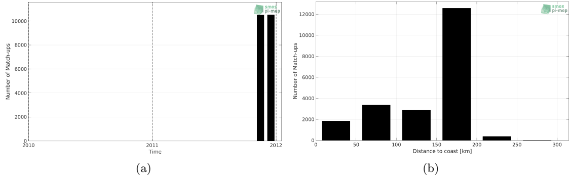
Figure 1: Number of match-ups between TSG-SAMOS and CCI L4 Merged-OI v1.8 - 7-day running (ESA) SSS as a function of time (a) and as function of the distance to coast (b) over the Mediterranean Sea Pi-MEP region and for the full satellite product period.
