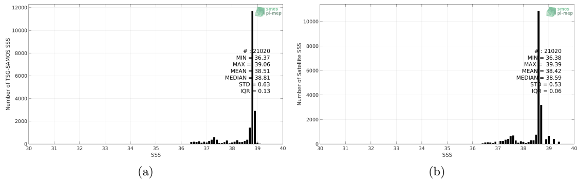
Figure 2: Histograms of SSS from TSG-SAMOS (a) and CCI L4 Merged-OI v1.8 - 7-day running (ESA) (b) considering all match-up pairs per bins of 0.1 over the Mediterranean Sea Pi-MEP region and for the full satellite product period.
