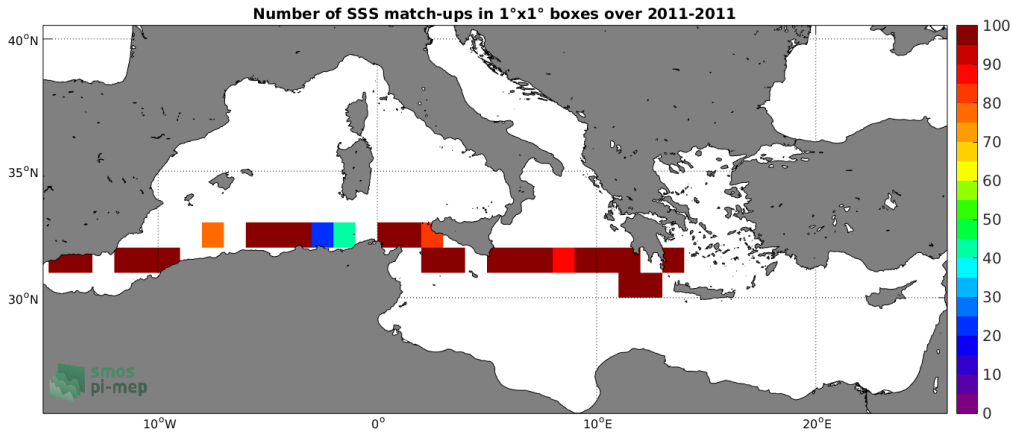
Figure 4: Number of SSS match-ups between TSG-SAMOS SSS and the CCI L4 Merged-OI v1.8 - 7-day running (ESA) SSS product for the Mediterranean Sea Pi-MEP region over 1°x1° boxes and for the full satellite product period.
