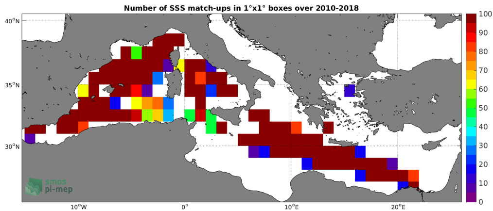
Figure 4: Number of SSS match-ups between TSG-LEGOS-DM SSS and the CCI-L4-ESA-MERGED-OI-V1.8-7DAY-RUNNING SSS product for the Mediterranean Sea Pi-MEP region over 1^\circ \times 1^\circ boxes and for the full satellite product period.
