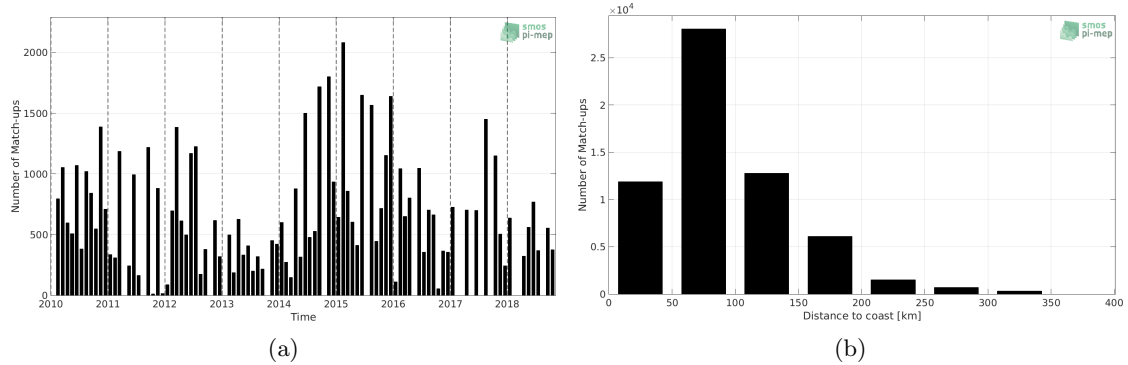
Figure 1: Number of match-ups between TSG-LEGOS-DM and CCI-L4-ESA-MERGED-OI-V1.8-7DAY-RUNNING SSS as a function of time (a) and as function of the distance to coast (b) over the Mediterranean Sea Pi-MEP region and for the full satellite product period.
