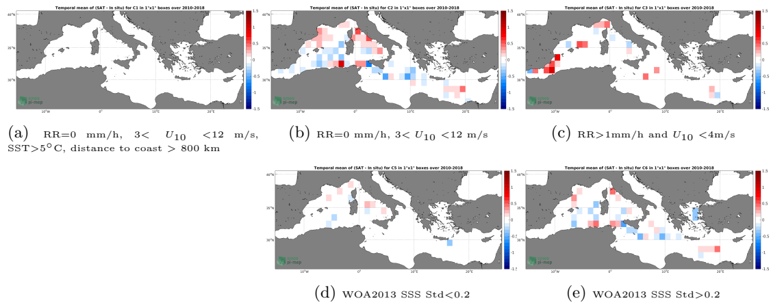
Figure 12: Temporal mean gridded over spatial boxes of size 1^\circ \times 1^\circ of \Delta SSS (CCI-L4-ESAMERGED-OI-V1.8-7DAY-RUNNING - TSG-LEGOS-DM) for 5 different subdatasets corresponding to:RR=0 mm/h, 3 < U_{10} < 12 m/s, SST >5^\circ\text{C} , distance to coast > 800 km (a), RR=0 mm/h, 3 < U_{10} < 12 m/s (b), RR >1 mm/h and U_{10} < 4 m/s (c), WOA2013 SSS Std <0.2 (d), WOA2013 SSS Std >0.2 (e).
