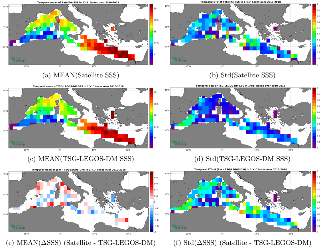
Figure 6: Temporal mean (left) and Std (right) of SSS from CCI-L4-ESA-MERGED-OI-V1.8-7DAY-RUNNING (top), TSG-LEGOS-DM (middle), and of \Delta SSS (Satellite - TSG-LEGOS-DM). Only match-up pairs are used to generate these maps.
