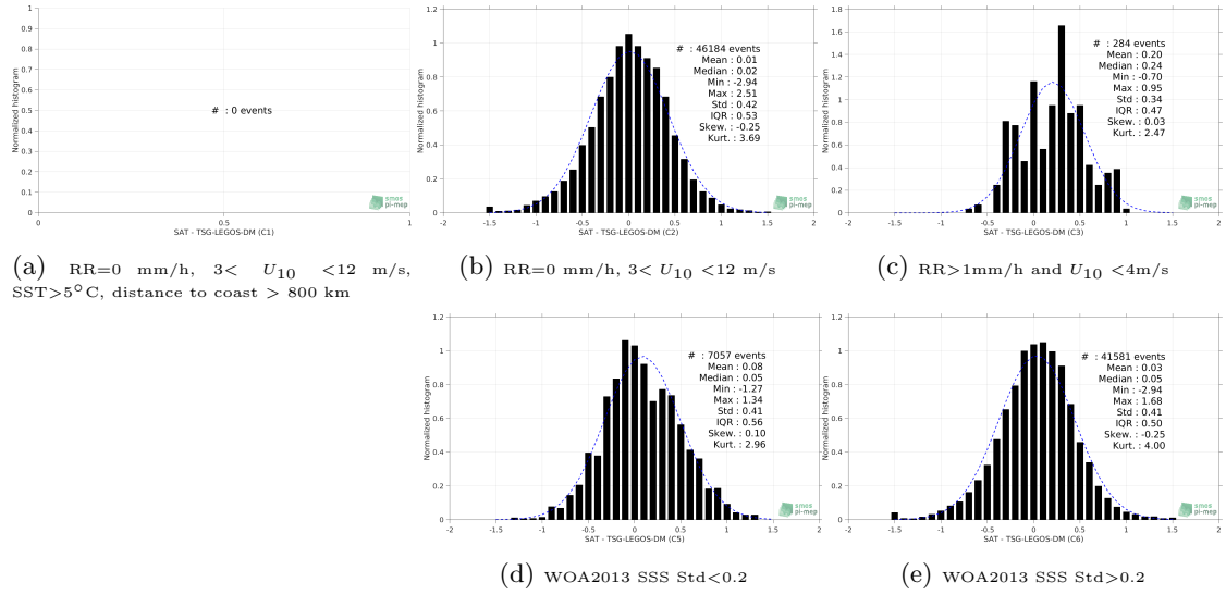
Figure 13: Normalized histogram of \Delta SSS (CCI-L4-ESA-MERGED-OI-V1.8-7DAY-RUNNING - TSG-LEGOS-DM) for 5 different subdatasets corresponding to: RR=0 mm/h, 3 < U_{10} < 12 m/s, SST > 5°C, distance to coast > 800 km (a), RR=0 mm/h, 3 < U_{10} < 12 m/s (b), RR > 1mm/h and U_{10} < 4 m/s (c), WOA2013 SSS Std < 0.2 (d), WOA2013 SSS Std > 0.2 (e).
