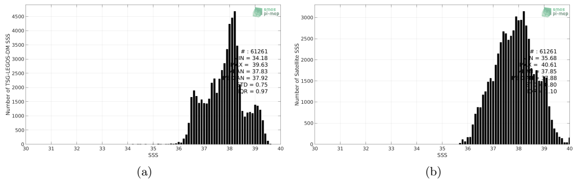
Figure 2: Histograms of SSS from TSG-LEGOS-DM (a) and CCI-L4-ESA-MERGED-OI-V1.8-7DAY-RUNNING (b) considering all match-up pairs per bins of 0.1 over the Mediterranean Sea Pi-MEP region and for the full satellite product period.
