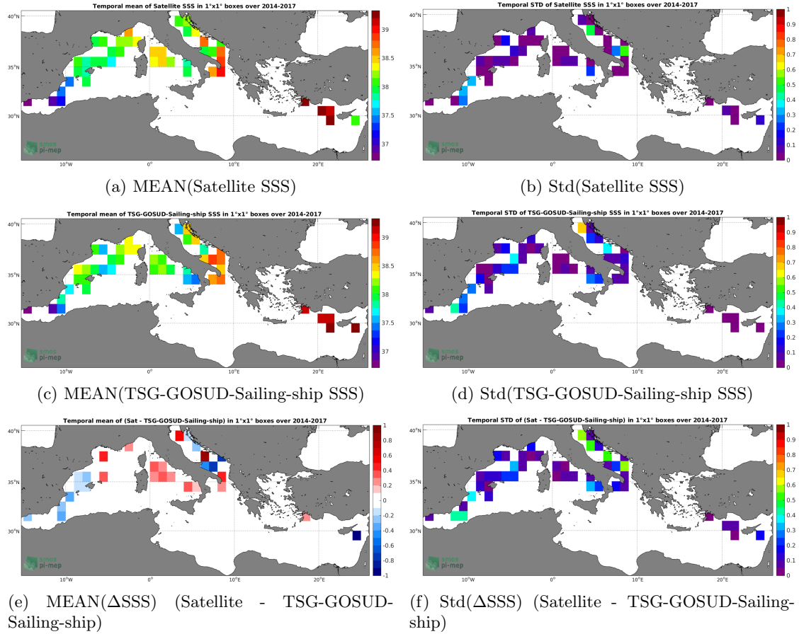
Figure 6: Temporal mean (left) and Std (right) of SSS from CCI L4 Merged-OI v1.8 - 7-day running (ESA) (top), TSG-GOSUD-Sailing-ship (middle), and of \Delta SSS (Satellite - TSG-GOSUD-Sailing-ship). Only match-up pairs are used to generate these maps.
