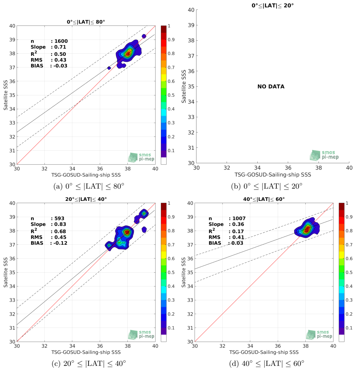
Figure 9: Contour maps of the concentration of CCI L4 Merged-OI v1.8 - 7-day running (ESA) SSS (y-axis) versus TSG-GOSUD-Sailing-ship SSS (x-axis) at match-up pairs for different latitude bands. For each plot, the red line shows x=y . The black thin and dashed lines indicate a linear fit through the data cloud and the \pm 95\% confidence levels, respectively. The number match-up pairs n , the slope and R^2 coefficient of the linear fit, the root mean square (RMS) and the mean bias between satellite and in situ data are indicated for each latitude band in each plots.
