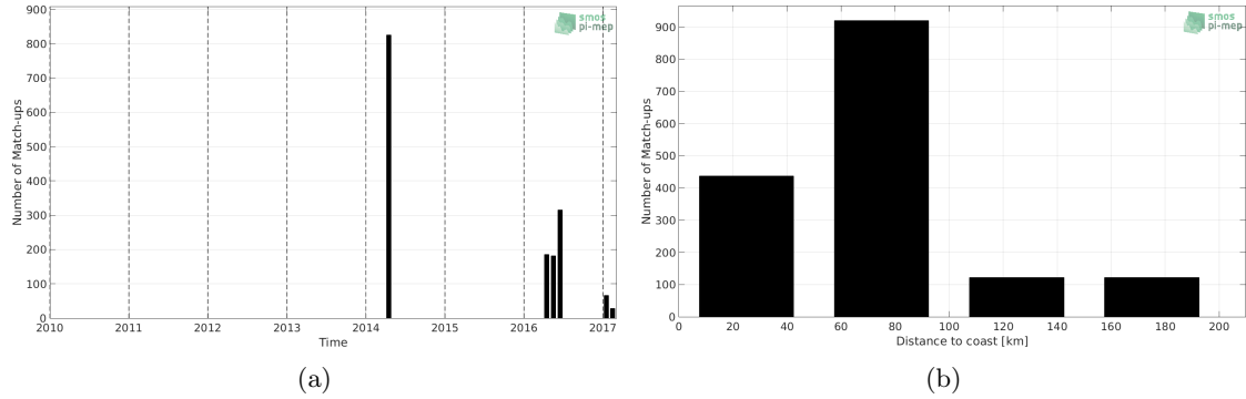
Figure 1: Number of match-ups between TSG-GOSUD-Sailing-ship and CCI L4 Merged-OI v1.8 - 7-day running (ESA) SSS as a function of time (a) and as function of the distance to coast (b) over the Mediterranean Sea Pi-MEP region and for the full satellite product period.
