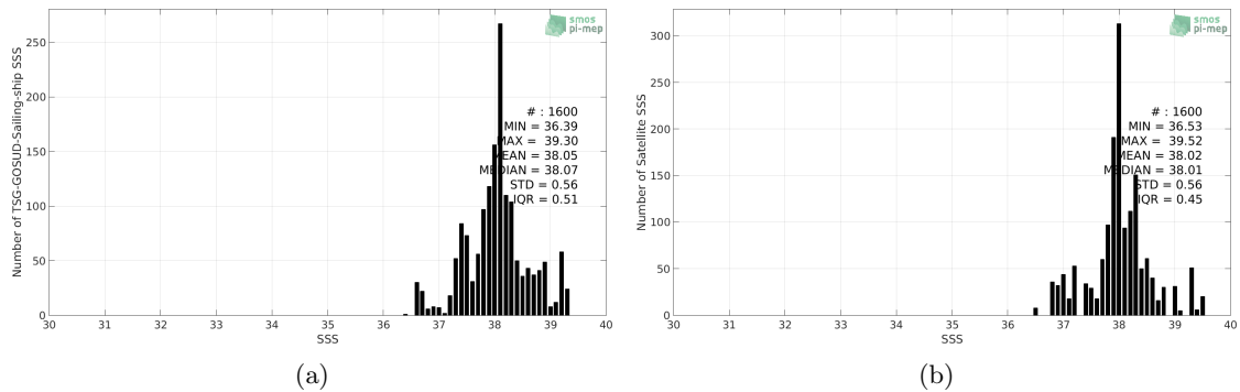
Figure 2: Histograms of SSS from TSG-GOSUD-Sailing-ship (a) and CCI-L4-ESA-MERGED-OI-V1.8-7DAY-RUNNING (b) considering all match-up pairs per bins of 0.1 over the Mediterranean Sea Pi-MEP region and for the full satellite product period.
