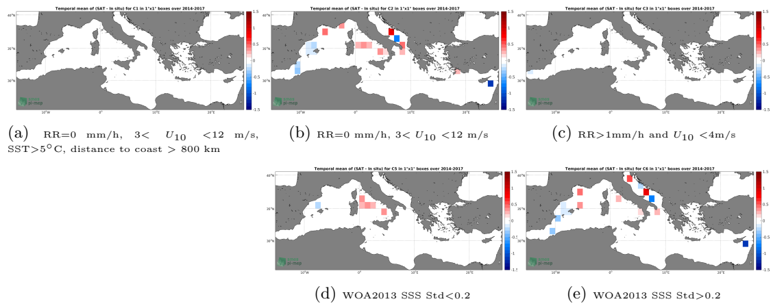
Figure 12: Temporal mean gridded over spatial boxes of size 1^\circ \times 1^\circ of \Delta SSS (CCI-L4-ESA-MERGED-OI-V1.8-7DAY-RUNNING - TSG-GOSUD-Sailing-ship) for 5 different subdatasets corresponding to:RR=0 mm/h, 3 < U_{10} < 12 m/s, SST>5°C, distance to coast > 800 km (a), RR=0 mm/h, 3 < U_{10} < 12 m/s (b), RR>1mm/h and U_{10} < 4 m/s (c), WOA2013 SSS Std<0.2 (d), WOA2013 SSS Std>0.2 (e).
