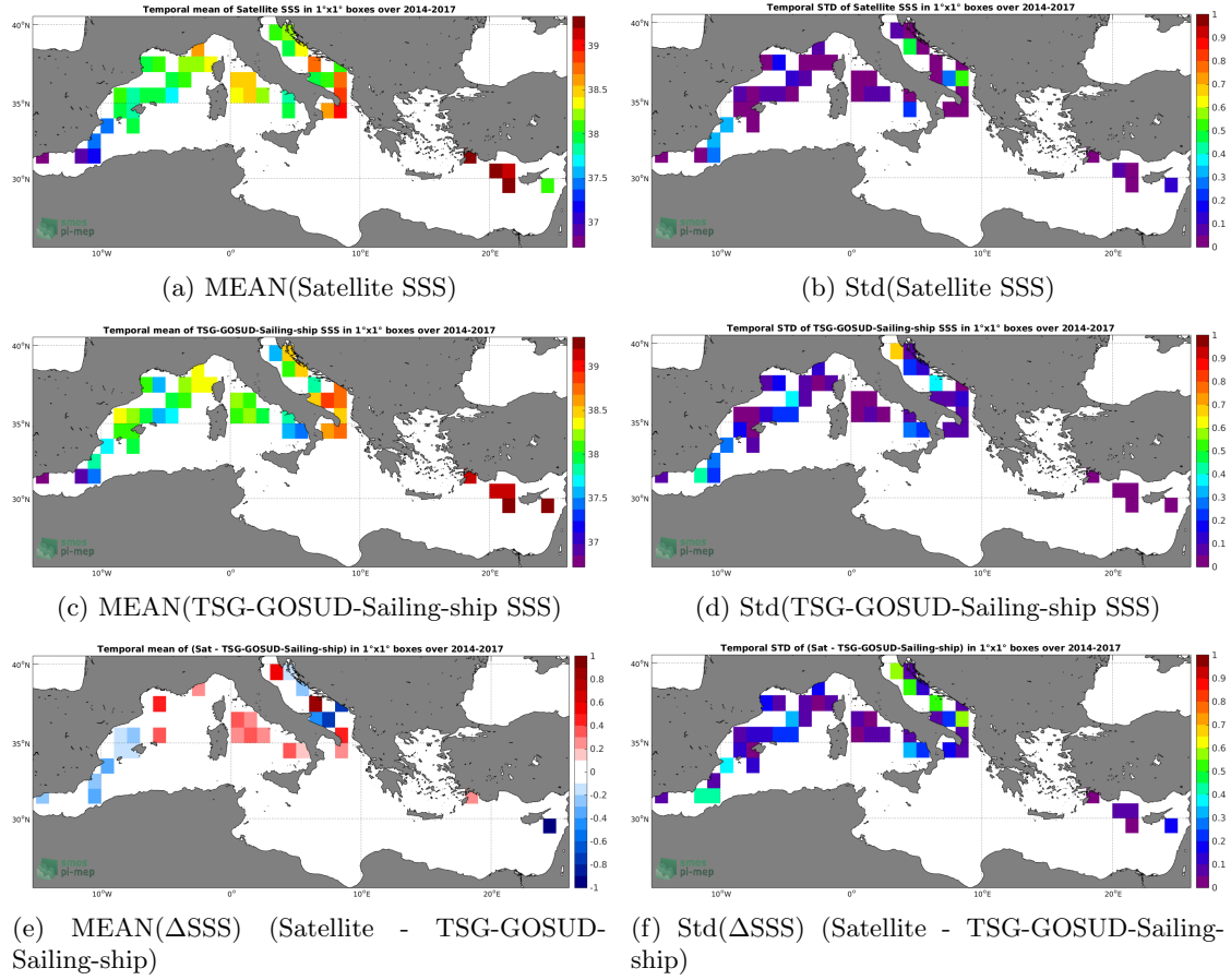
Figure 6: Temporal mean (left) and Std (right) of SSS from CCI-L4-ESA-MERGED-OI-V1.8-7DAY-RUNNING (top), TSG-GOSUD-Sailing-ship (middle), and of \Delta SSS (Satellite - TSG-GOSUD-Sailing-ship). Only match-up pairs are used to generate these maps.
