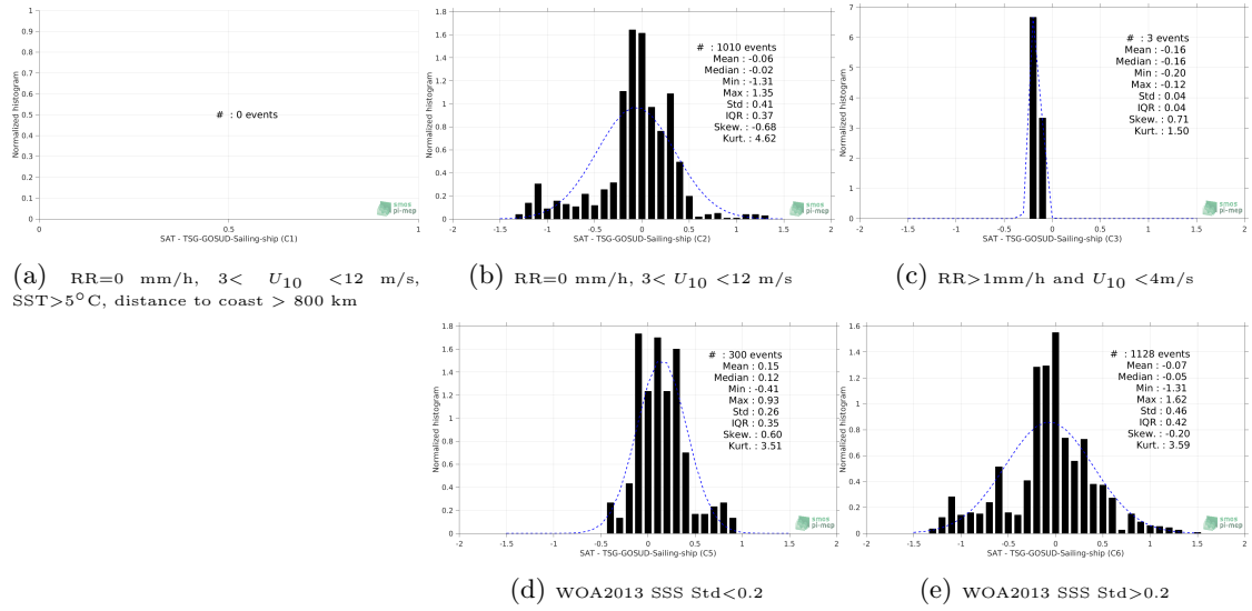
Figure 13: Normalized histogram of \Delta SSS (CCI-L4-ESA-MERGED-OI-V1.8-7DAY-RUNNING - TSG-GOSUD-Sailing-ship) for 5 different subdatasets corresponding to: RR=0 mm/h, 3 < U_{10} < 12 m/s, SST>5°C, distance to coast > 800 km (a), RR=0 mm/h, 3 < U_{10} < 12 m/s (b), RR>1mm/h and U_{10} < 4 m/s (c), WOA2013 SSS Std<0.2 (d), WOA2013 SSS Std>0.2 (e).
