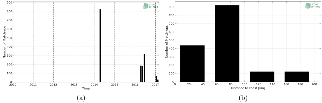
Figure 1: Number of match-ups between TSG-GOSUD-Sailing-ship and CCI-L4-ESA-MERGED-OI-V1.8-7DAY-RUNNING SSS as a function of time (a) and as function of the distance to coast (b) over the Mediterranean Sea Pi-MEP region and for the full satellite product period.
