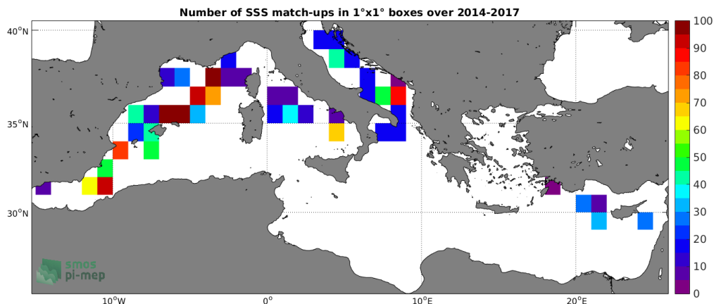
Figure 4: Number of SSS match-ups between TSG-GOSUD-Sailing-ship SSS and the CCI-L4-ESA-MERGED-OI-V1.8-7DAY-RUNNING SSS product for the Mediterranean Sea Pi-MEP region over 1^\circ \times 1^\circ boxes and for the full satellite product period.
