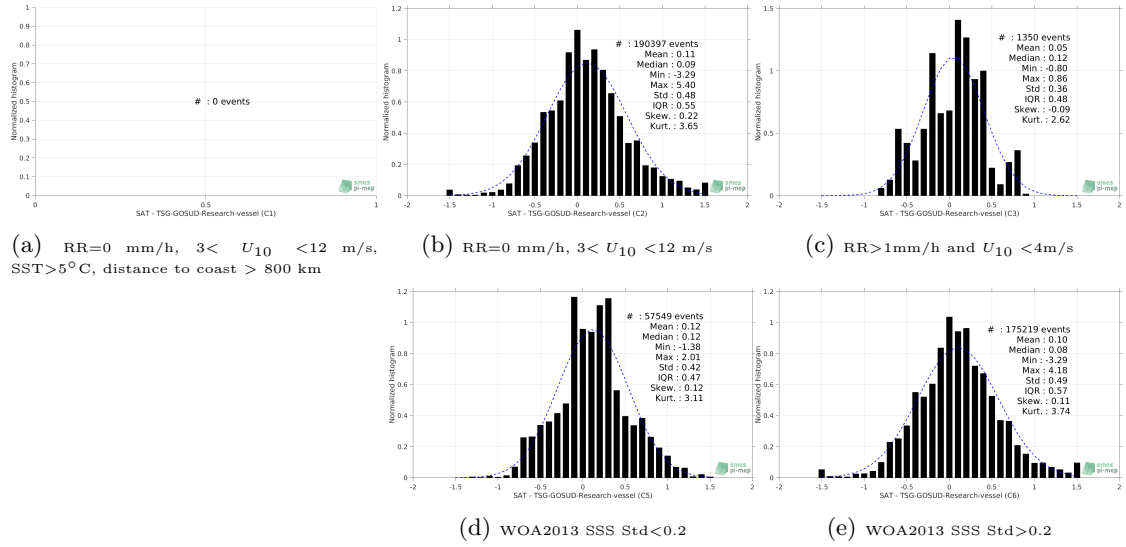
Figure 13: Normalized histogram of \Delta SSS (CCI-L4-ESA-MERGED-OI-V1.8-7DAY-RUNNING - TSG-GOSUD-Research-vessel) for 5 different subdatasets corresponding to: RR=0 mm/h, 3 < U_{10} < 12 m/s, SST > 5°C, distance to coast > 800 km (a), RR=0 mm/h, 3 < U_{10} < 12 m/s (b), RR > 1mm/h and U_{10} < 4 m/s (c), WOA2013 SSS Std < 0.2 (d), WOA2013 SSS Std > 0.2 (e).
