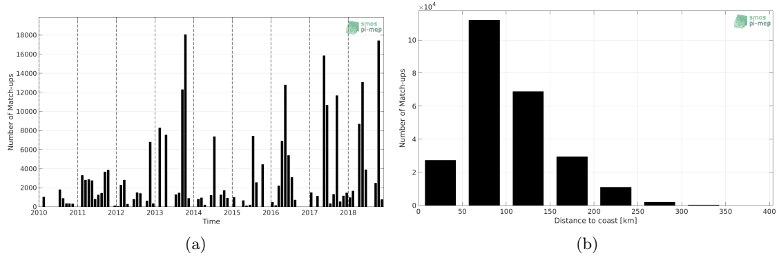
Figure 1: Number of match-ups between TSG-GOSUD-Research-vessel and CCI-L4-ESAMERGED-OI-V1.8-7DAY-RUNNING SSS as a function of time (a) and as function of the distance to coast (b) over the Mediterranean Sea Pi-MEP region and for the full satellite product period.
