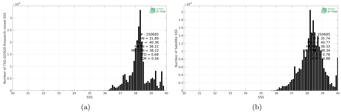
Figure 2: Histograms of SSS from TSG-GOSUD-Research-vessel (a) and CCI-L4-ESAMERGED-OI-V1.8-7DAY-RUNNING (b) considering all match-up pairs per bins of 0.1 over the Mediterranean Sea Pi-MEP region and for the full satellite product period.
