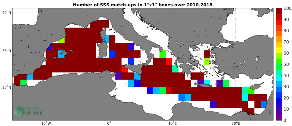
Figure 4: Number of SSS match-ups between TSG-GOSUD-Research-vessel SSS and the CCI-L4-ESA-MERGED-OI-V1.8-7DAY-RUNNING SSS product for the Mediterranean Sea Pi-MEP region over 1^\circ \times 1^\circ boxes and for the full satellite product period.
