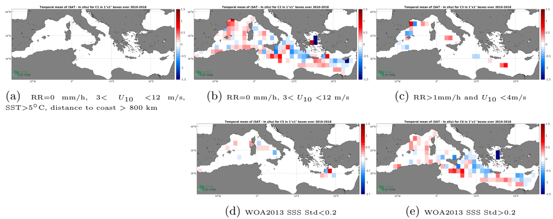
Figure 12: Temporal mean gridded over spatial boxes of size 1^\circ \times 1^\circ of \Delta SSS (CCI-L4-ESA-MERGED-OI-V1.8-7DAY-RUNNING - TSG-GOSUD-Research-vessel) for 5 different sub-datasets corresponding to: RR=0 mm/h, 3 < U_{10} < 12 m/s, SST>5°C, distance to coast > 800 km (a), RR=0 mm/h, 3 < U_{10} < 12 m/s (b), RR>1mm/h and U_{10} < 4 m/s (c), WOA2013 SSS Std<0.2 (d), WOA2013 SSS Std>0.2 (e).
