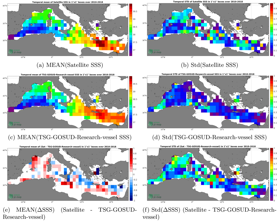
Figure 6: Temporal mean (left) and Std (right) of SSS from CCI-L4-ESA-MERGED-OI-V1.8-7DAY-RUNNING (top), TSG-GOSUD-Research-vessel (middle), and of \Delta SSS (Satellite - TSG-GOSUD-Research-vessel). Only match-up pairs are used to generate these maps.
