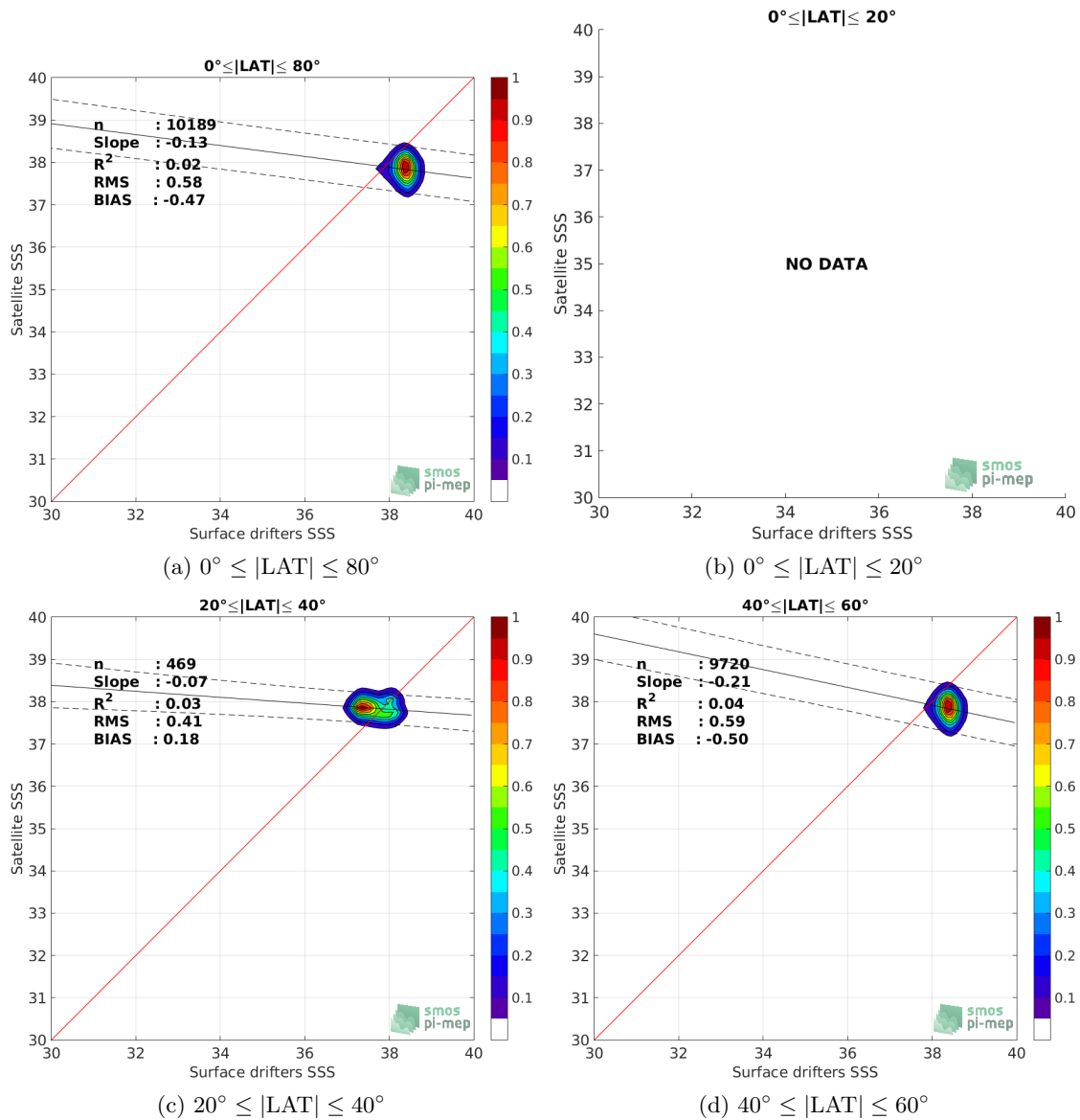
Figure 8: Contour maps of the concentration of CCI L4 Merged-OI v1.8 - 7-day running (ESA) SSS (y-axis) versus Surface drifters SSS (x-axis) at match-up pairs for different latitude bands. For each plot, the red line shows x=y . The black thin and dashed lines indicate a linear fit through the data cloud and the \pm 95\% confidence levels, respectively. The number match-up pairs n , the slope and R^2 coefficient of the linear fit, the root mean square (RMS) and the mean bias between satellite and in situ data are indicated for each latitude band in each plots.
