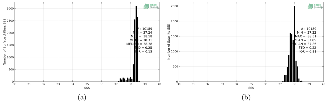
Figure 2: Histograms of SSS from Surface drifters (a) and CCI L4 Merged-OI v1.8 - 7-day running (ESA) (b) considering all match-up pairs per bins of 0.1 over the Mediterranean Sea Pi-MEP region and for the full satellite product period.
