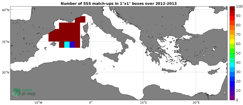
Figure 3: Number of SSS match-ups between Surface drifters SSS and the CCI L4 Merged-OI v1.8 - 7-day running (ESA) SSS product for the Mediterranean Sea Pi-MEP region over 1^\circ \times 1^\circ boxes and for the full satellite product period.
