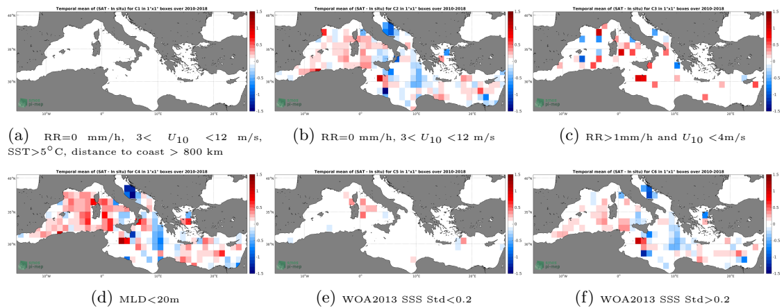
Figure 12: Temporal mean gridded over spatial boxes of size 1^\circ \times 1^\circ of \Delta SSS (CCI L4 Merged-OI v1.8 - 7-day running (ESA) - Argo) for 6 different subdatasets corresponding to:RR=0 mm/h, 3 < U_{10} < 12 m/s, SST > 5^\circ C , distance to coast > 800 km (a), RR=0 mm/h, 3 < U_{10} < 12 m/s (b), RR > 1 mm/h and U_{10} < 4 m/s (c),MLD < 20 m (d),WOA2013 SSS Std < 0.2 (e),WOA2013 SSS Std > 0.2 (f).
