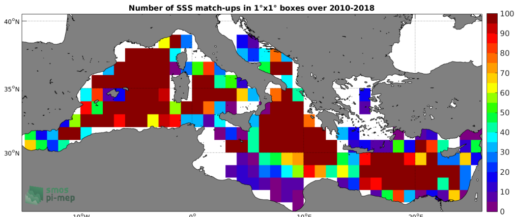
Figure 4: Number of SSS match-ups between Argo SSS and the CCI L4 Merged-OI v1.8 - 7-day running (ESA) SSS product for the Mediterranean Sea Pi-MEP region over 1°x1° boxes and for the full satellite product period.
