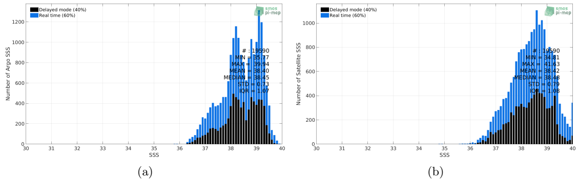
Figure 2: Histograms of SSS from Argo (a) and CCI L4 Merged-OI v1.8 - 7-day running (ESA) (b) considering all match-up pairs per bins of 0.1 over the Mediterranean Sea Pi-MEP region and for the full satellite product period.
