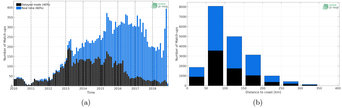
Figure 1: Number of match-ups between Argo and CCI L4 Merged-OI v1.8 - 7-day running (ESA) SSS as a function of time (a) and as function of the distance to coast (b) over the Mediterranean Sea Pi-MEP region and for the full satellite product period.
