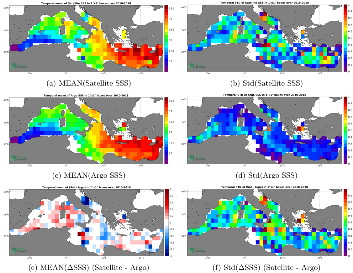
Figure 6: Temporal mean (left) and Std (right) of SSS from CCI L4 Merged-OI v1.8 - 7-day running (ESA) (top), Argo (middle), and of \Delta SSS (Satellite - Argo). Only match-up pairs are used to generate these maps.
