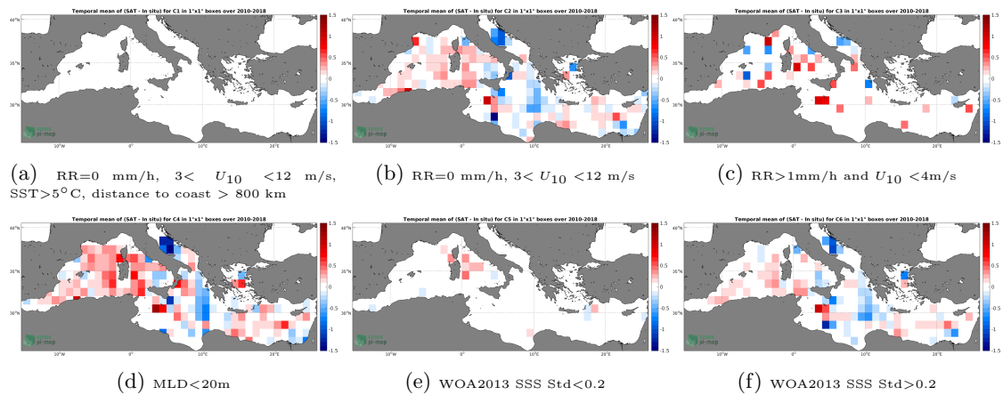
Figure 12: Temporal mean gridded over spatial boxes of size 1^\circ \times 1^\circ of \Delta SSS (CCI-L4-ESA-MERGED-OI-V1.8-7DAY-RUNNING - Argo) for 6 different subdatasets corresponding to:RR=0 mm/h, 3 < U_{10} < 12 m/s, SST >5^\circ C, distance to coast > 800 km (a), RR=0 mm/h, 3 < U_{10} < 12 m/s (b), RR >1 mm/h and U_{10} < 4 m/s (c),MLD <20 m (d),WOA2013 SSS Std <0.2 (e),WOA2013 SSS Std >0.2 (f).
