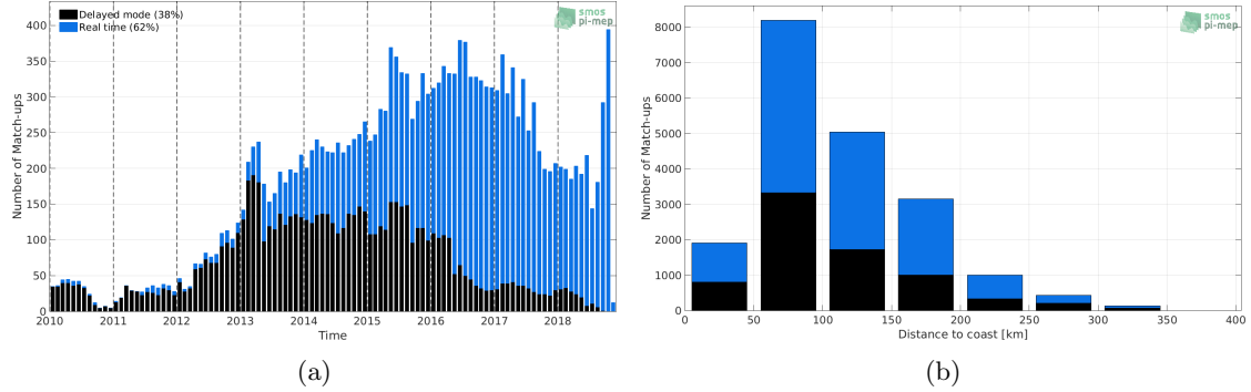
Figure 1: Number of match-ups between Argo and CCI-L4-ESA-MERGED-OI-V1.8-7DAY-RUNNING SSS as a function of time (a) and as function of the distance to coast (b) over the Mediterranean Sea Pi-MEP region and for the full satellite product period.
