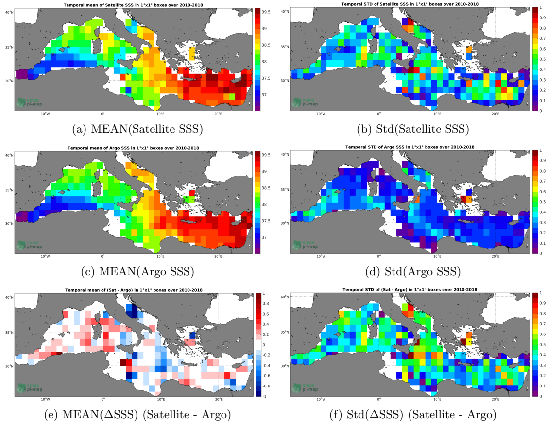
Figure 6: Temporal mean (left) and Std (right) of SSS from CCI-L4-ESA-MERGED-OI-V1.8-7DAY-RUNNING (top), Argo (middle), and of \Delta SSS (Satellite - Argo). Only match-up pairs are used to generate these maps.
