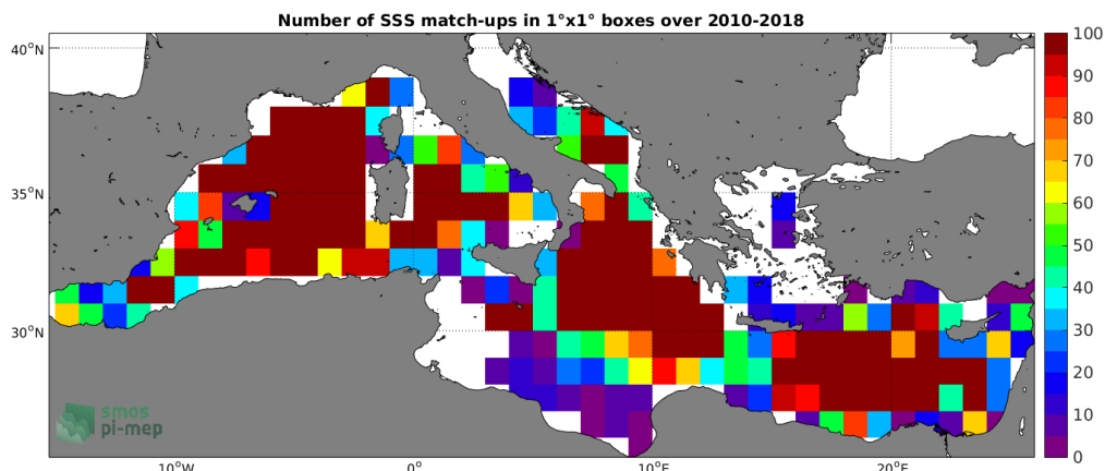
Figure 4: Number of SSS match-ups between Argo SSS and the CCI-L4-ESA-MERGED-OI-V1.8-7DAY-RUNNING SSS product for the Mediterranean Sea Pi-MEP region over 1°x1° boxes and for the full satellite product period.
