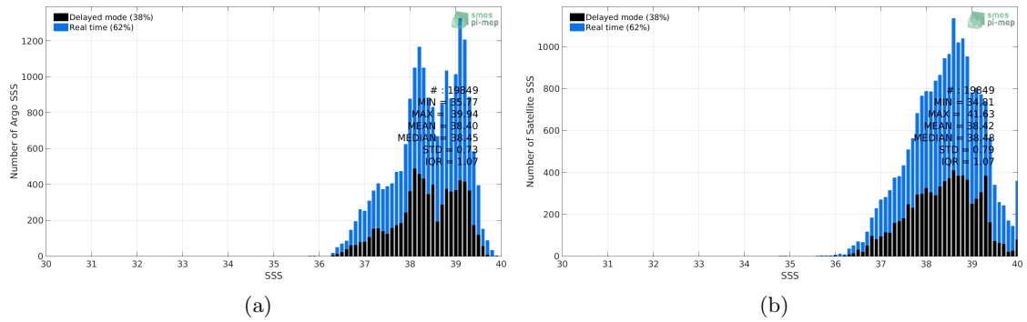
Figure 2: Histograms of SSS from Argo (a) and CCI-L4-ESA-MERGED-OI-V1.8-7DAY-RUNNING (b) considering all match-up pairs per bins of 0.1 over the Mediterranean Sea Pi-MEP region and for the full satellite product period.
