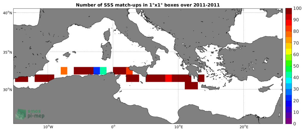
Figure 4: Number of SSS match-ups between TSG-SAMOS SSS and the CCI L4 Merged-OI v1.8 - 30-day running (ESA) SSS product for the Mediterranean Sea Pi-MEP region over 1^\circ \times 1^\circ boxes and for the full satellite product period.
