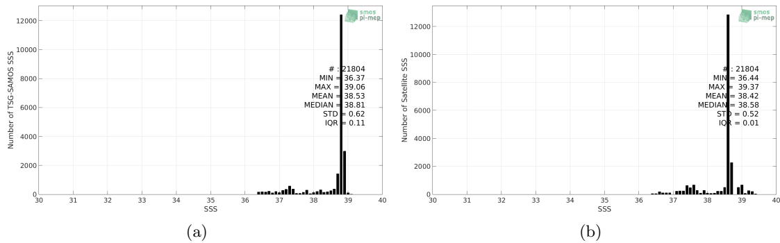
Figure 2: Histograms of SSS from TSG-SAMOS (a) and CCI L4 Merged-OI v1.8 - 30-day running (ESA) (b) considering all match-up pairs per bins of 0.1 over the Mediterranean Sea Pi-MEP region and for the full satellite product period.
