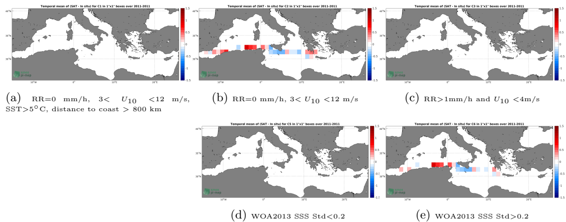
Figure 12: Temporal mean gridded over spatial boxes of size 1^{\circ}\times 1^{\circ} of \Delta\text{SSS} (CCI L4 Merged-OI v1.8 - 30-day running (ESA) - TSG-SAMOS) for 5 different subdatasets corresponding to:RR=0 mm/h, 3 < U_{10} < 12 m/s, SST > 5^{\circ}\text{C} , distance to coast > 800 km (a), RR=0 mm/h, 3 < U_{10} < 12 m/s (b), RR > 1 mm/h and U_{10} < 4 m/s (c), WOA2013 SSS Std < 0.2 (d), WOA2013 SSS Std > 0.2 (e).
