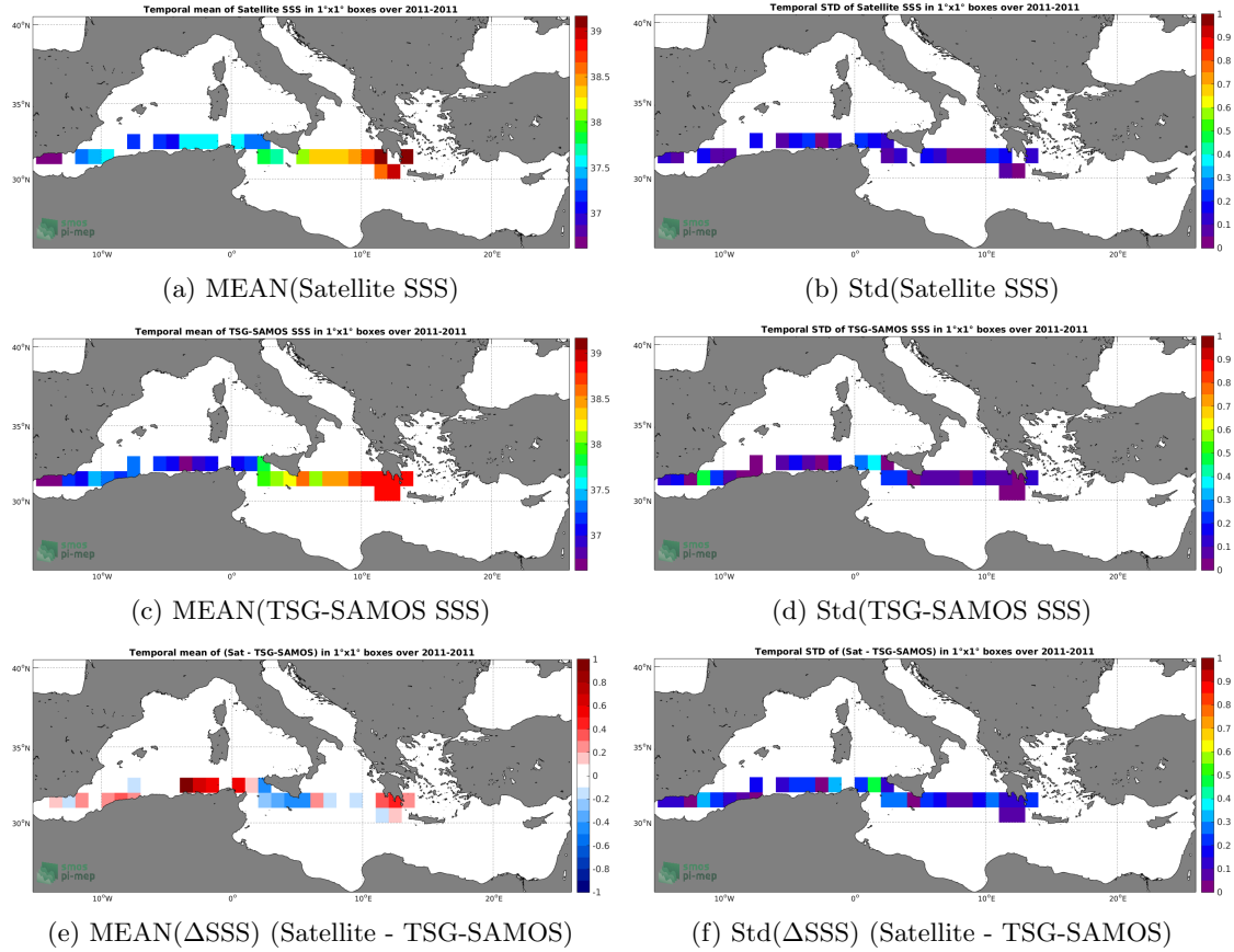
Figure 6: Temporal mean (left) and Std (right) of SSS from CCI L4 Merged-OI v1.8 - 30-day running (ESA) (top), TSG-SAMOS (middle), and of \Delta SSS (Satellite - TSG-SAMOS). Only match-up pairs are used to generate these maps.
