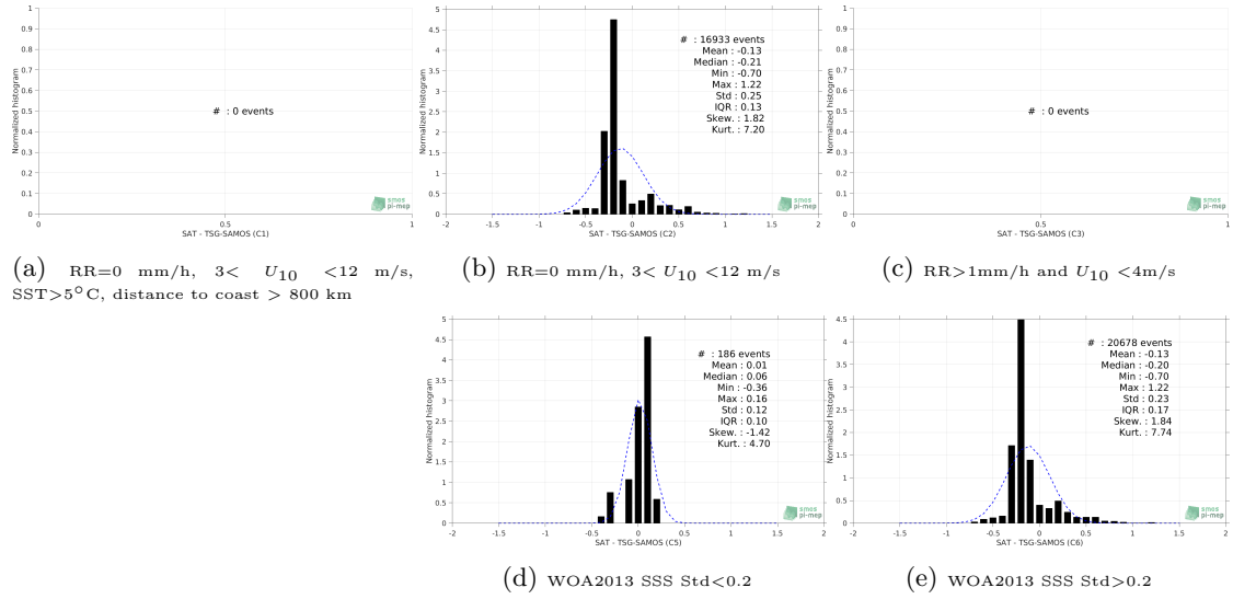
Figure 13: Normalized histogram of \Delta SSS (CCI L4 Merged-OI v1.8 - 30-day running (ESA) - TSG-SAMOS) for 5 different subdatasets corresponding to: RR=0 mm/h, 3 < U_{10} < 12 m/s, SST > 5°C, distance to coast > 800 km (a), RR=0 mm/h, 3 < U_{10} < 12 m/s (b), RR > 1mm/h and U_{10} < 4 m/s (c), WOA2013 SSS Std < 0.2 (d), WOA2013 SSS Std > 0.2 (e).
