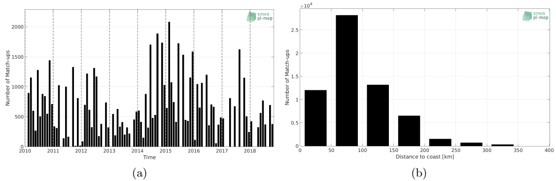
Figure 1: Number of match-ups between TSG-LEGOS-DM and CCI L4 Merged-OI v1.8 - 30-day running (ESA) SSS as a function of time (a) and as function of the distance to coast (b) over the Mediterranean Sea Pi-MEP region and for the full satellite product period.
