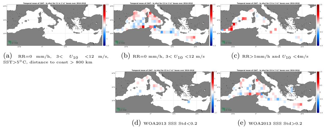
Figure 12: Temporal mean gridded over spatial boxes of size 1^\circ \times 1^\circ of \Delta SSS (CCI L4 Merged-OI v1.8 - 30-day running (ESA) - TSG-LEGOS-DM) for 5 different subdatasets corresponding to:RR=0 mm/h, 3 < U_{10} < 12 m/s, SST >5^\circ\text{C} , distance to coast > 800 km (a), RR=0 mm/h, 3 < U_{10} < 12 m/s (b), RR >1 mm/h and U_{10} < 4 m/s (c), WOA2013 SSS Std <0.2 (d), WOA2013 SSS Std >0.2 (e).
