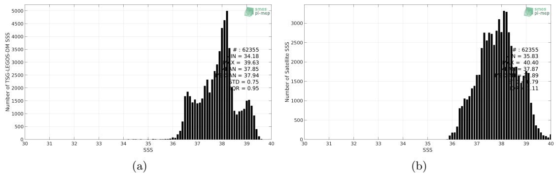
Figure 2: Histograms of SSS from TSG-LEGOS-DM (a) and CCI L4 Merged-OI v1.8 - 30-day running (ESA) (b) considering all match-up pairs per bins of 0.1 over the Mediterranean Sea Pi-MEP region and for the full satellite product period.
