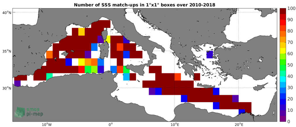
Figure 4: Number of SSS match-ups between TSG-LEGOS-DM SSS and the CCI L4 Merged-OI v1.8 - 30-day running (ESA) SSS product for the Mediterranean Sea Pi-MEP region over 1^\circ \times 1^\circ boxes and for the full satellite product period.
