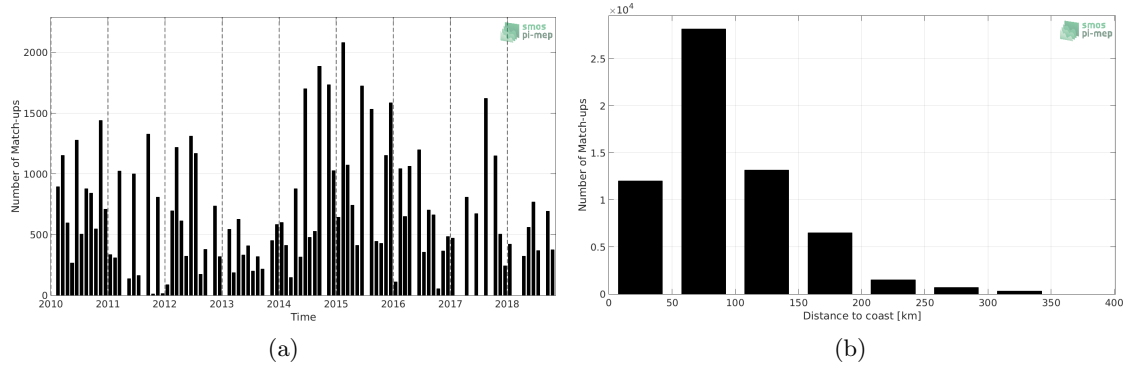
Figure 1: Number of match-ups between TSG-LEGOS-DM and CCI-L4-ESA-MERGED-OI-V1.8-30DAY-RUNNING SSS as a function of time (a) and as function of the distance to coast (b) over the Mediterranean Sea Pi-MEP region and for the full satellite product period.
