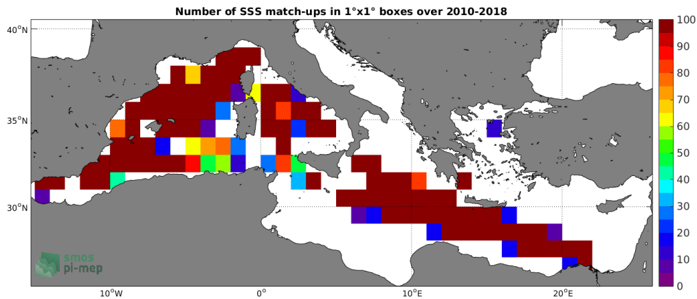
Figure 4: Number of SSS match-ups between TSG-LEGOS-DM SSS and the CCI-L4-ESA-MERGED-OI-V1.8-30DAY-RUNNING SSS product for the Mediterranean Sea Pi-MEP region over 1^\circ \times 1^\circ boxes and for the full satellite product period.
