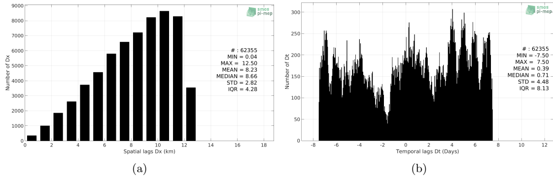
Figure 5: Histograms of the spatial (a) and temporal (b) lags between the time of the TSG-LEGOS-DM measurements and the date of the corresponding CCI-L4-ESA-MERGED-OI-V1.8-30DAY-RUNNING SSS product.
