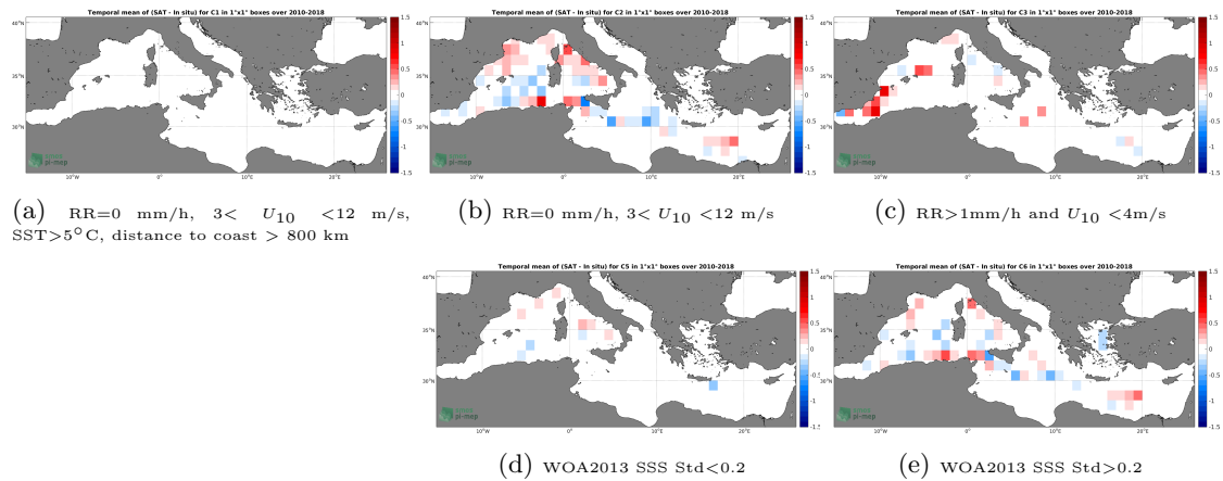
Figure 12: Temporal mean gridded over spatial boxes of size 1^\circ \times 1^\circ of \Delta SSS (CCI-L4-ESAMERGED-OI-V1.8-30DAY-RUNNING - TSG-LEGOS-DM) for 5 different subdatasets corresponding to:RR=0 mm/h, 3 < U_{10} < 12 m/s, SST >5^\circ\text{C} , distance to coast > 800 km (a), RR=0 mm/h, 3 < U_{10} < 12 m/s (b), RR >1 mm/h and U_{10} < 4 m/s (c), WOA2013 SSS Std <0.2 (d), WOA2013 SSS Std >0.2 (e).
