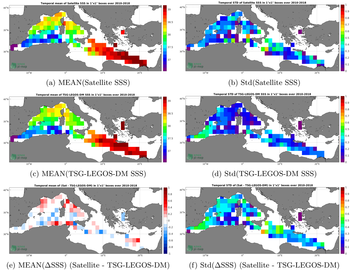
Figure 6: Temporal mean (left) and Std (right) of SSS from CCI-L4-ESA-MERGED-OI-V1.8-30DAY-RUNNING (top), TSG-LEGOS-DM (middle), and of \Delta SSS (Satellite - TSG-LEGOS-DM). Only match-up pairs are used to generate these maps.
