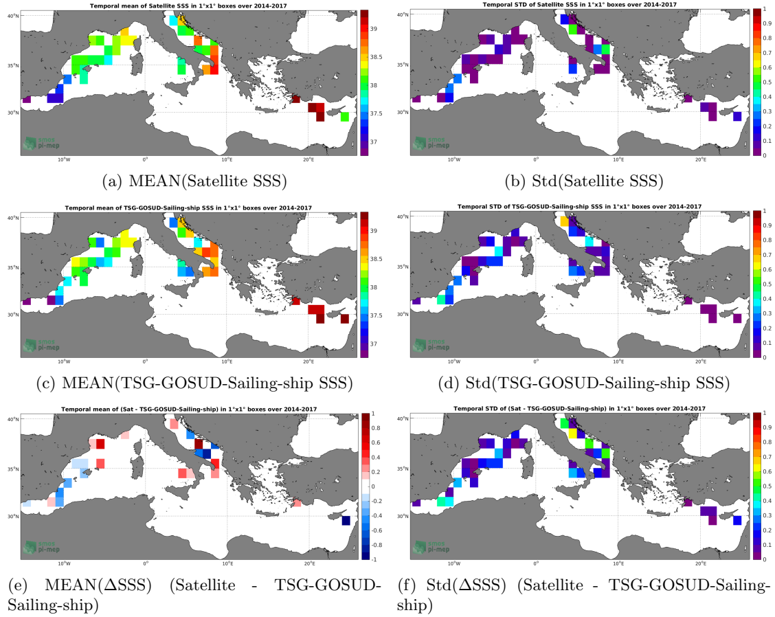
Figure 6: Temporal mean (left) and Std (right) of SSS from CCI L4 Merged-OI v1.8 - 30-day running (ESA) (top), TSG-GOSUD-Sailing-ship (middle), and of \Delta SSS (Satellite - TSG-GOSUD-Sailing-ship). Only match-up pairs are used to generate these maps.
