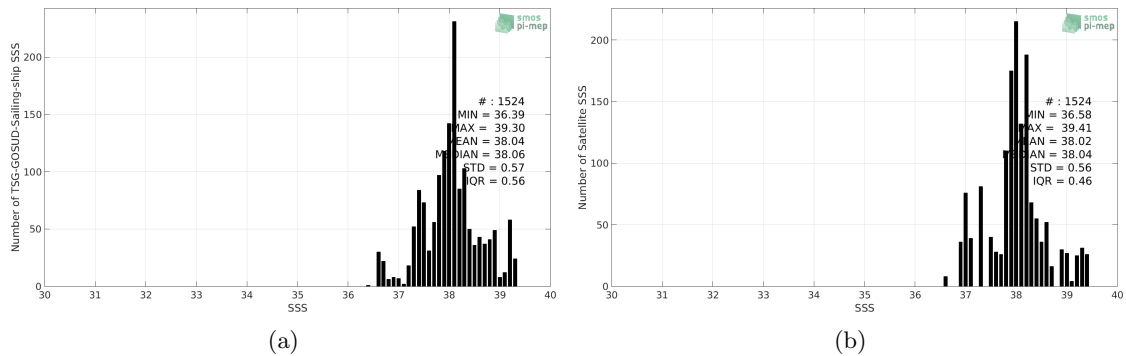
Figure 2: Histograms of SSS from TSG-GOSUD-Sailing-ship (a) and CCI L4 Merged-OI v1.8 - 30-day running (ESA) (b) considering all match-up pairs per bins of 0.1 over the Mediterranean Sea Pi-MEP region and for the full satellite product period.
