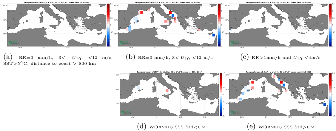
Figure 12: Temporal mean gridded over spatial boxes of size 1^{\circ}\times 1^{\circ} of \Delta SSS (CCI L4 Merged-OI v1.8 - 30-day running (ESA) - TSG-GOSUD-Sailing-ship) for 5 different subdatasets corresponding to:RR=0 mm/h, 3 < U_{10} < 12 m/s, SST >5^{\circ}\text{C} , distance to coast > 800 km (a), RR=0 mm/h, 3 < U_{10} < 12 m/s (b), RR >1 mm/h and U_{10} < 4 m/s (c), WOA2013 SSS Std <0.2 (d), WOA2013 SSS Std >0.2 (e).
