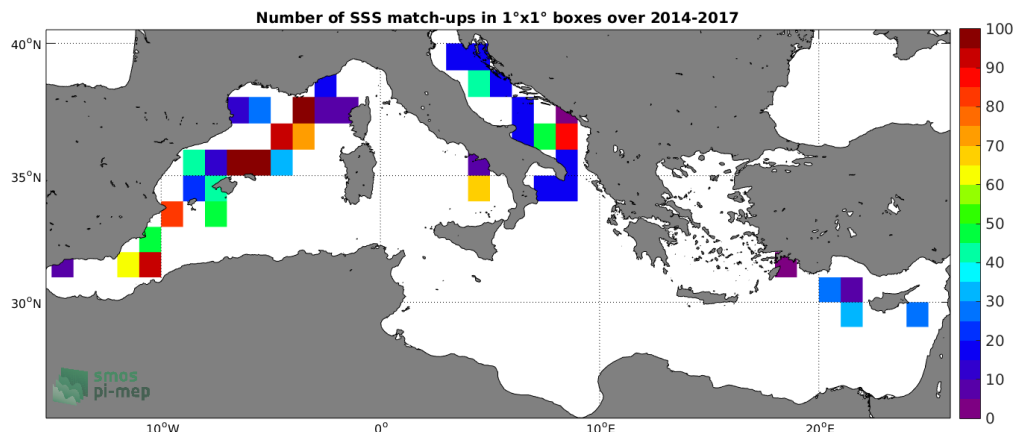
Figure 4: Number of SSS match-ups between TSG-GOSUD-Sailing-ship SSS and the CCI L4 Merged-OI v1.8 - 30-day running (ESA) SSS product for the Mediterranean Sea Pi-MEP region over 1°x1° boxes and for the full satellite product period.
