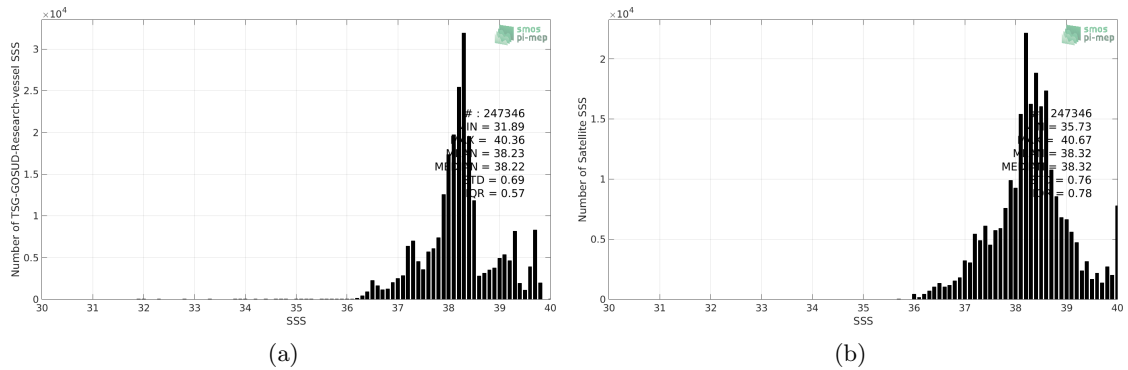
Figure 2: Histograms of SSS from TSG-GOSUD-Research-vessel (a) and CCI-L4-ESAMERGED-OI-V1.8-30DAY-RUNNING (b) considering all match-up pairs per bins of 0.1 over the Mediterranean Sea Pi-MEP region and for the full satellite product period.
