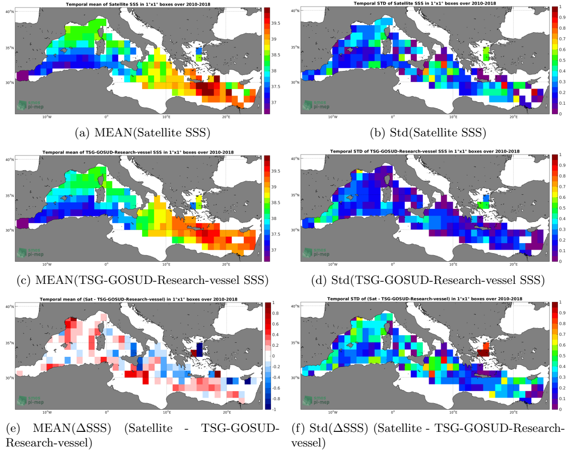
Figure 6: Temporal mean (left) and Std (right) of SSS from CCI-L4-ESA-MERGED-OI-V1.8-30DAY-RUNNING (top), TSG-GOSUD-Research-vessel (middle), and of \Delta SSS (Satellite - TSG-GOSUD-Research-vessel). Only match-up pairs are used to generate these maps.
