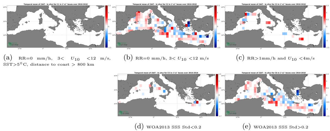
Figure 12: Temporal mean gridded over spatial boxes of size 1^\circ \times 1^\circ of \Delta SSS (CCI-L4-ESA-MERGED-OI-V1.8-30DAY-RUNNING - TSG-GOSUD-Research-vessel) for 5 different sub-datasets corresponding to:RR=0 mm/h, 3 < U_{10} < 12 m/s, SST >5^\circ\text{C} , distance to coast > 800 km (a), RR=0 mm/h, 3 < U_{10} < 12 m/s (b), RR >1 mm/h and U_{10} < 4 m/s (c), WOA2013 SSS Std <0.2 (d), WOA2013 SSS Std >0.2 (e).
