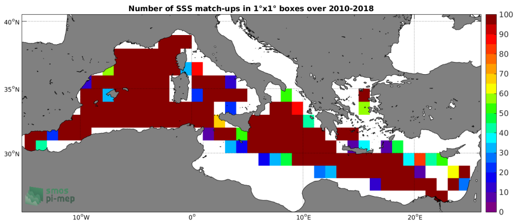
Figure 4: Number of SSS match-ups between TSG-GOSUD-Research-vessel SSS and the CCI-L4-ESA-MERGED-OI-V1.8-30DAY-RUNNING SSS product for the Mediterranean Sea Pi-MEP region over 1^\circ \times 1^\circ boxes and for the full satellite product period.
