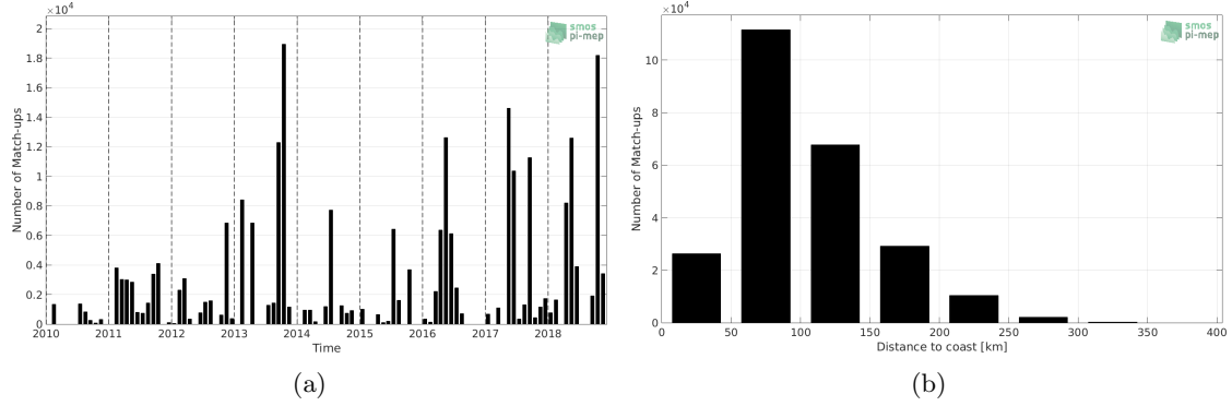
Figure 1: Number of match-ups between TSG-GOSUD-Research-vessel and CCI-L4-ESAMERGED-OI-V1.8-30DAY-RUNNING SSS as a function of time (a) and as function of the distance to coast (b) over the Mediterranean Sea Pi-MEP region and for the full satellite product period.
