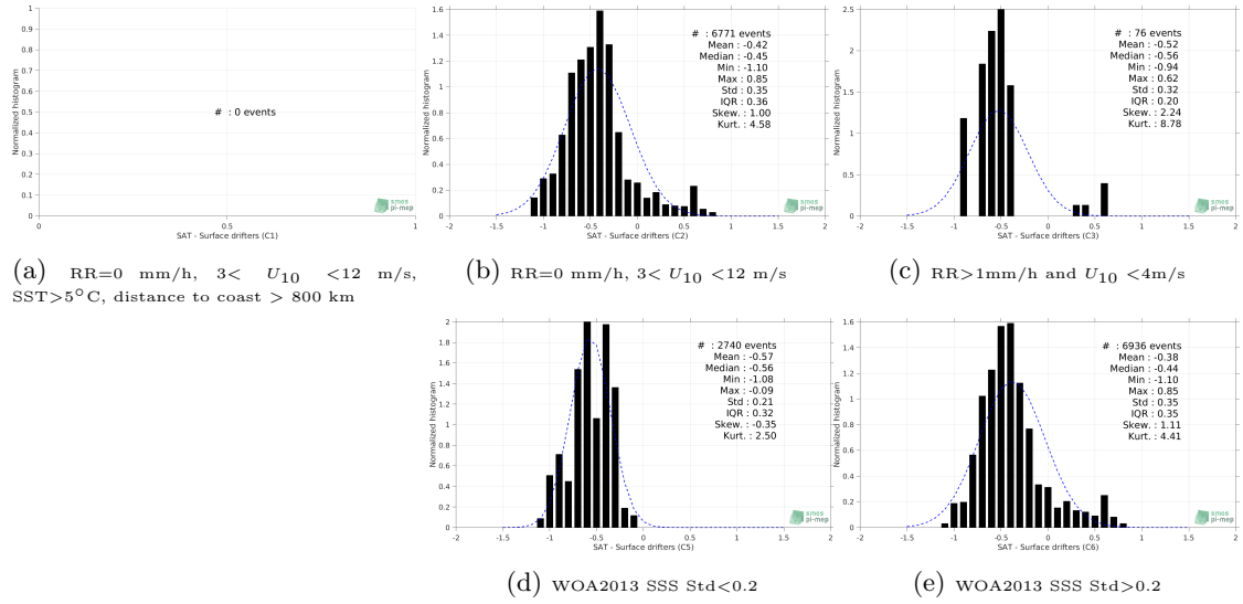
Figure 12: Normalized histogram of \Delta SSS (CCI L4 Merged-OI v1.8 - 30-day running (ESA) - Surface drifters) for 5 different subdatasets corresponding to: RR=0 mm/h, 3 < U_{10} < 12 m/s, SST > 5°C, distance to coast > 800 km (a), RR=0 mm/h, 3 < U_{10} < 12 m/s (b), RR > 1mm/h and U_{10} < 4 m/s (c), WOA2013 SSS Std < 0.2 (d), WOA2013 SSS Std > 0.2 (e).
