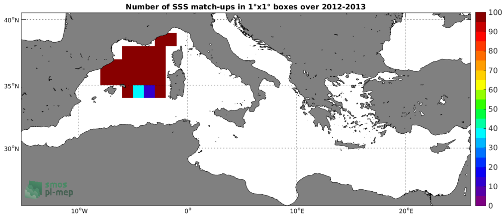
Figure 3: Number of SSS match-ups between Surface drifters SSS and the CCI L4 Merged-OI v1.8 - 30-day running (ESA) SSS product for the Mediterranean Sea Pi-MEP region over 1^\circ \times 1^\circ boxes and for the full satellite product period.
