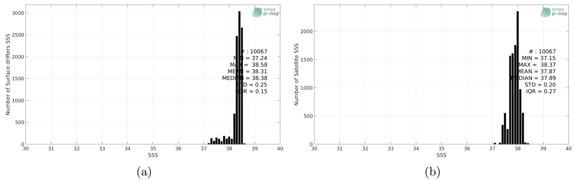
Figure 2: Histograms of SSS from Surface drifters (a) and CCI L4 Merged-OI v1.8 - 30-day running (ESA) (b) considering all match-up pairs per bins of 0.1 over the Mediterranean Sea Pi-MEP region and for the full satellite product period.
