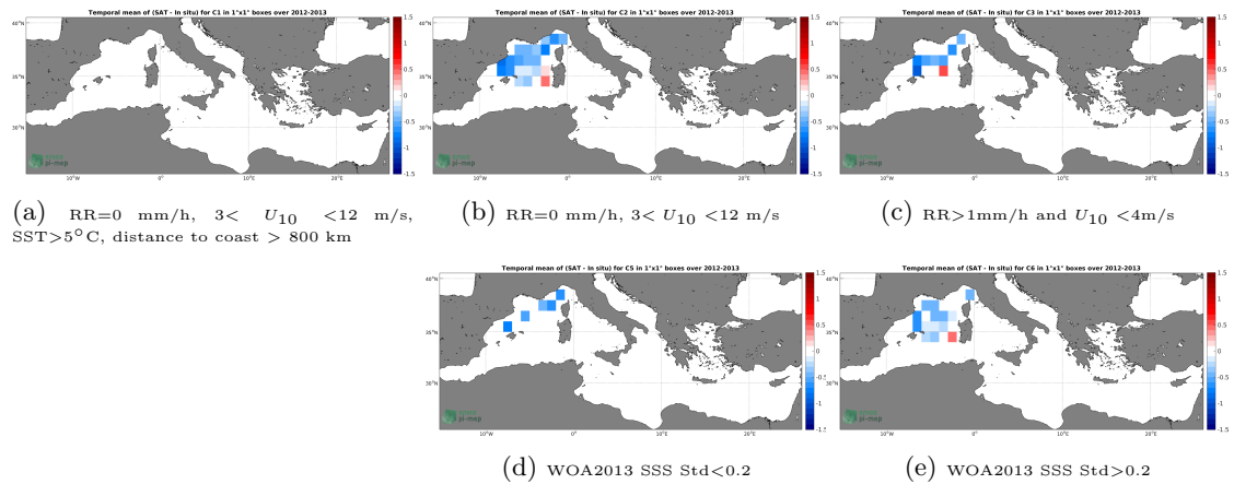
Figure 11: Temporal mean gridded over spatial boxes of size 1^\circ \times 1^\circ of \Delta SSS (CCI L4 Merged-OI v1.8 - 30-day running (ESA) - Surface drifters) for 5 different subdatasets corresponding to:RR=0 mm/h, 3 < U_{10} < 12 m/s, SST >5^\circ C, distance to coast > 800 km (a), RR=0 mm/h, 3 < U_{10} < 12 m/s (b), RR >1 mm/h and U_{10} < 4 m/s (c), WOA2013 SSS Std <0.2 (d), WOA2013 SSS Std >0.2 (e).
