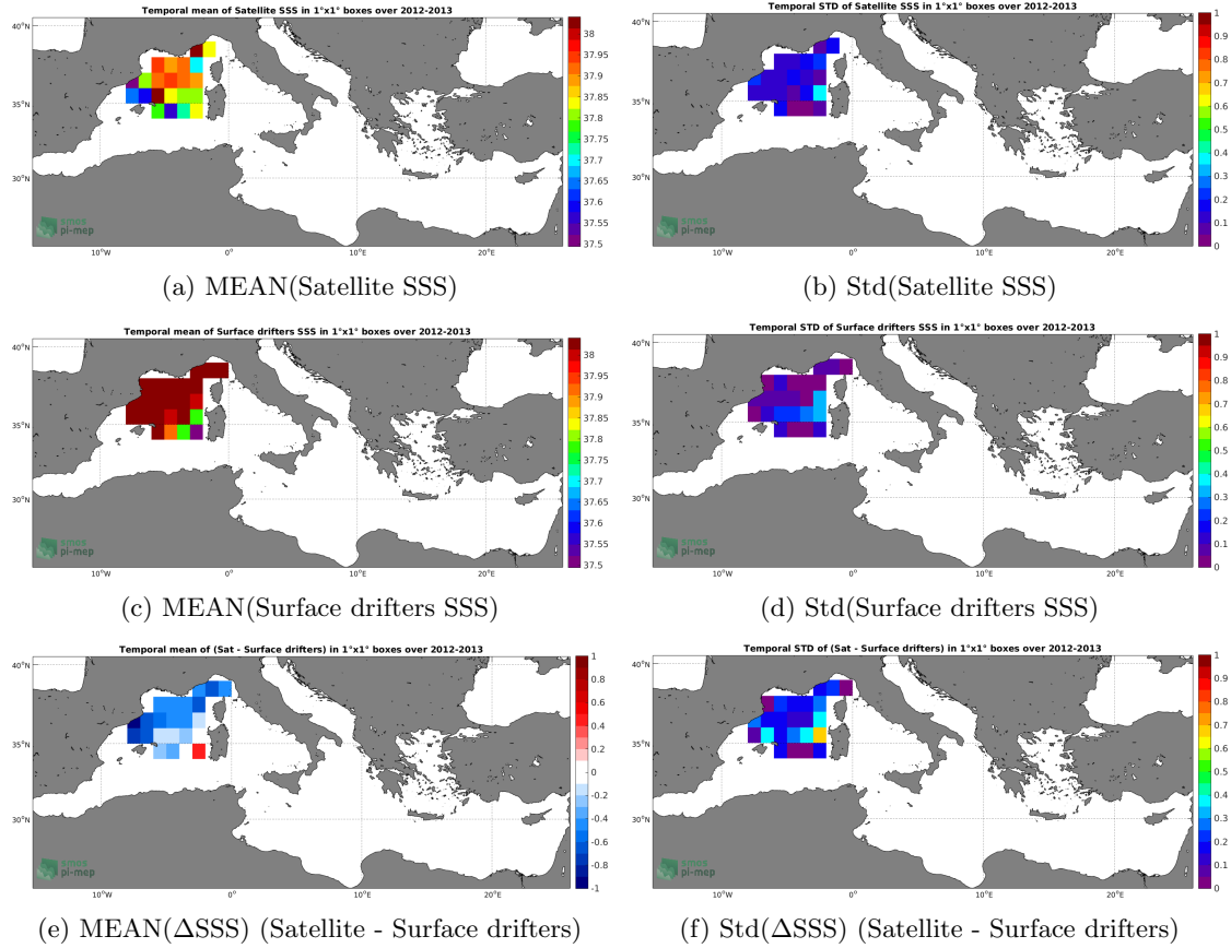
Figure 5: Temporal mean (left) and Std (right) of SSS from CCI L4 Merged-OI v1.8 - 30-day running (ESA) (top), Surface drifters (middle), and of \Delta SSS (Satellite - Surface drifters). Only match-up pairs are used to generate these maps.
