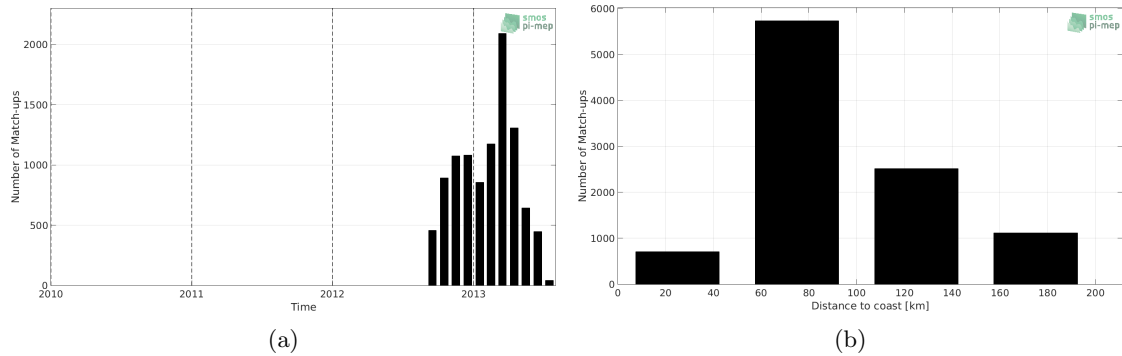
Figure 1: Number of match-ups between Surface drifters and CCI L4 Merged-OI v1.8 - 30-day running (ESA) SSS as a function of time (a) and as function of the distance to coast (b) over the Mediterranean Sea Pi-MEP region and for the full satellite product period.
