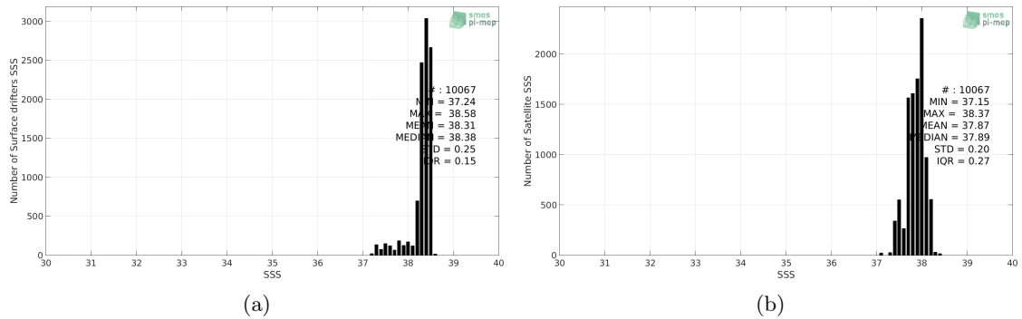
Figure 2: Histograms of SSS from Surface drifters (a) and CCI-L4-ESA-MERGED-OI-V1.8-30DAY-RUNNING (b) considering all match-up pairs per bins of 0.1 over the Mediterranean Sea Pi-MEP region and for the full satellite product period.
