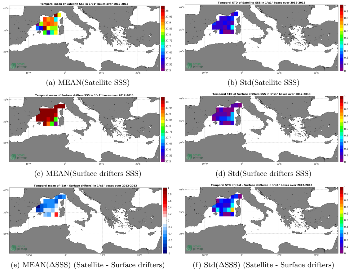
Figure 5: Temporal mean (left) and Std (right) of SSS from CCI-L4-ESA-MERGED-OI-V1.8-30DAY-RUNNING (top), Surface drifters (middle), and of \Delta SSS (Satellite - Surface drifters). Only match-up pairs are used to generate these maps.
