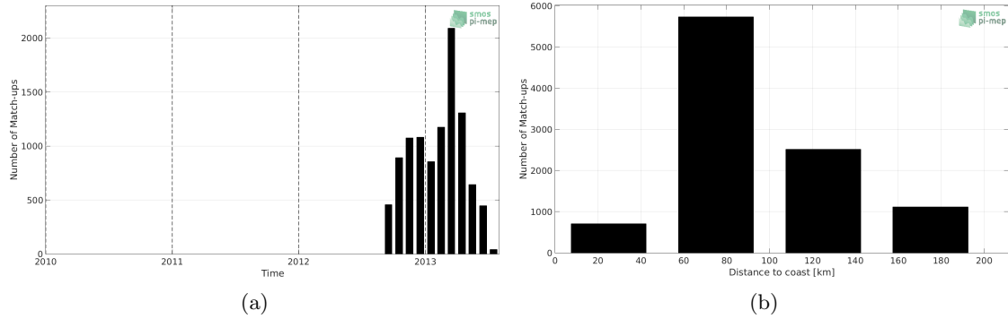
Figure 1: Number of match-ups between Surface drifters and CCI-L4-ESA-MERGED-OI-V1.8-30DAY-RUNNING SSS as a function of time (a) and as function of the distance to coast (b) over the Mediterranean Sea Pi-MEP region and for the full satellite product period.
