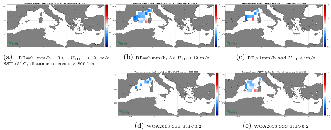
Figure 11: Temporal mean gridded over spatial boxes of size 1^\circ \times 1^\circ of \Delta SSS (CCI-L4-ESAMERGED-OI-V1.8-30DAY-RUNNING - Surface drifters) for 5 different subdatasets corresponding to:RR=0 mm/h, 3 < U_{10} < 12 m/s, SST >5^\circ\text{C} , distance to coast > 800 km (a), RR=0 mm/h, 3 < U_{10} < 12 m/s (b), RR >1 mm/h and U_{10} < 4 m/s (c), WOA2013 SSS Std <0.2 (d), WOA2013 SSS Std >0.2 (e).
