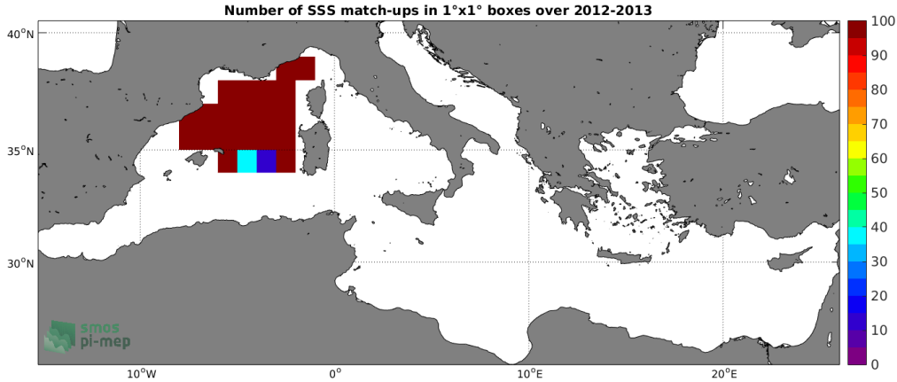
Figure 3: Number of SSS match-ups between Surface drifters SSS and the CCI-L4-ESA-MERGED-OI-V1.8-30DAY-RUNNING SSS product for the Mediterranean Sea Pi-MEP region over 1^\circ \times 1^\circ boxes and for the full satellite product period.
