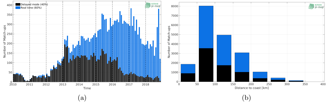
Figure 1: Number of match-ups between Argo and CCI L4 Merged-OI v1.8 - 30-day running (ESA) SSS as a function of time (a) and as function of the distance to coast (b) over the Mediterranean Sea Pi-MEP region and for the full satellite product period.
