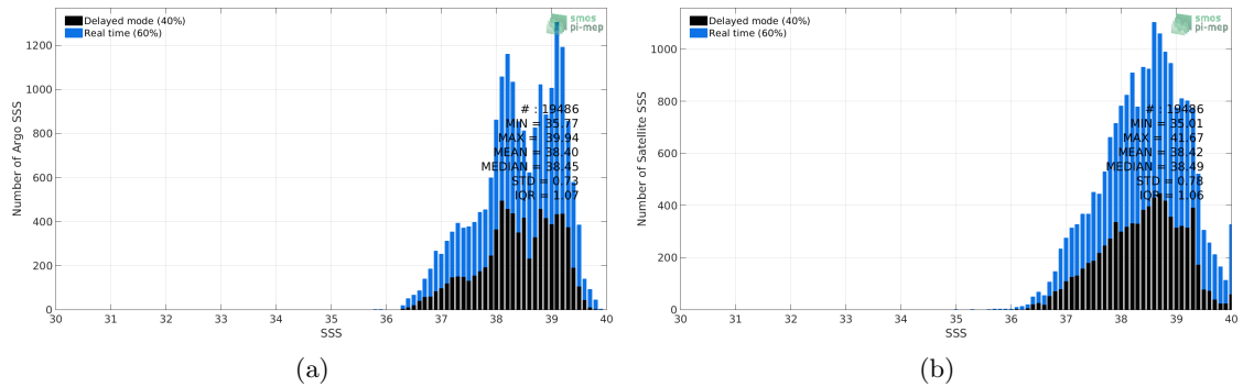
Figure 2: Histograms of SSS from Argo (a) and CCI L4 Merged-OI v1.8 - 30-day running (ESA) (b) considering all match-up pairs per bins of 0.1 over the Mediterranean Sea Pi-MEP region and for the full satellite product period.
