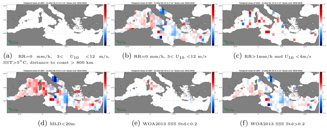
Figure 12: Temporal mean gridded over spatial boxes of size 1^\circ \times 1^\circ of \Delta SSS (CCI L4 Merged-OI v1.8 - 30-day running (ESA) - Argo) for 6 different subdatasets corresponding to:RR=0 mm/h, 3 < U_{10} < 12 m/s, SST >5^\circ C, distance to coast > 800 km (a), RR=0 mm/h, 3 < U_{10} < 12 m/s (b), RR >1 mm/h and U_{10} < 4 m/s (c),MLD <20 m (d),WOA2013 SSS Std <0.2 (e),WOA2013 SSS Std >0.2 (f).
