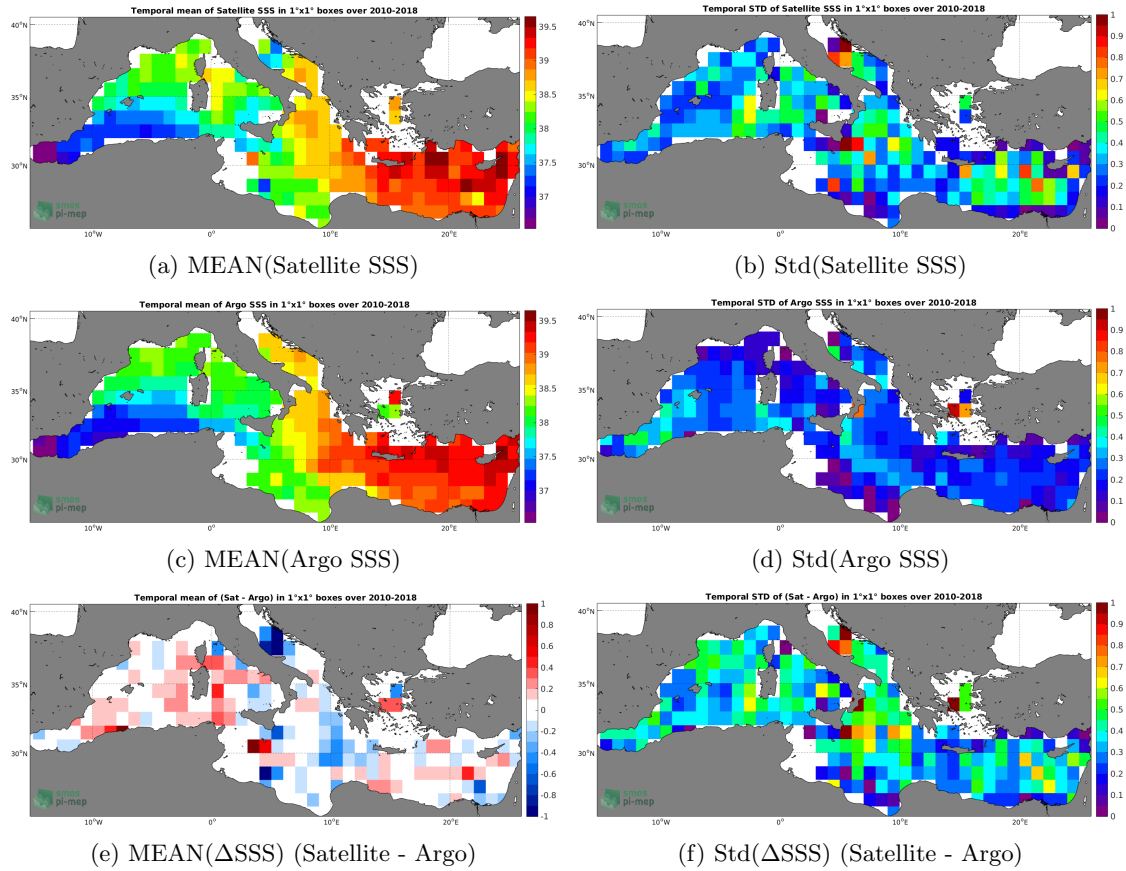
Figure 6: Temporal mean (left) and Std (right) of SSS from CCI L4 Merged-OI v1.8 - 30-day running (ESA) (top), Argo (middle), and of \Delta SSS (Satellite - Argo). Only match-up pairs are used to generate these maps.
