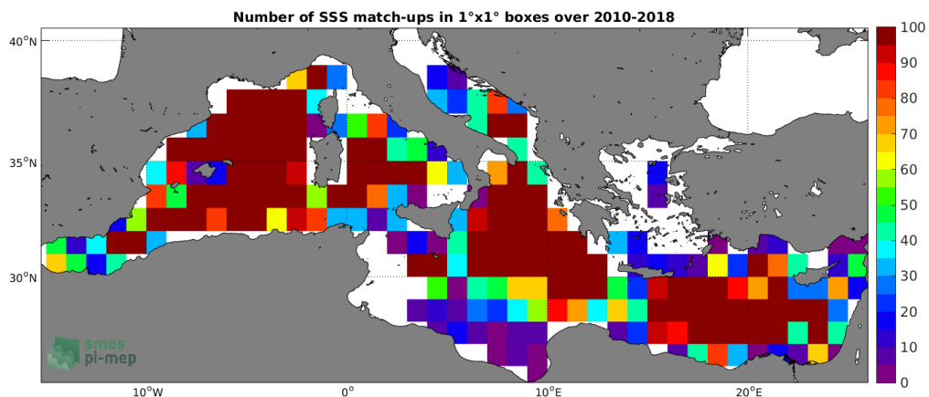
Figure 4: Number of SSS match-ups between Argo SSS and the CCI L4 Merged-OI v1.8 - 30-day running (ESA) SSS product for the Mediterranean Sea Pi-MEP region over 1^\circ \times 1^\circ boxes and for the full satellite product period.
