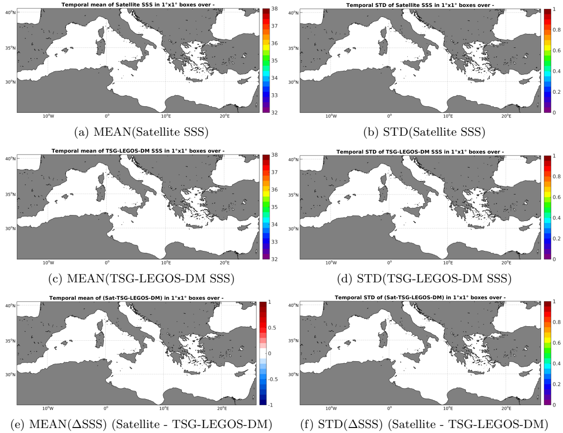
Figure 6: Temporal mean (left) and STD (right) of SSS from Aquarius-L4-IPRC-V4-WEEKLY (top), TSG-LEGOS-DM (middle), and of \Delta SSS (Satellite - TSG-LEGOS-DM). Only match-up pairs are used to generate these maps.
