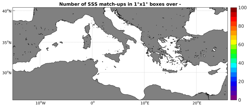
Figure 4: Number of SSS match-ups between TSG-LEGOS-DM SSS and the Aquarius-L4-IPRC-V4-WEEKLY SSS product for the Mediterranean Sea Pi-MEP region over 1^\circ \times 1^\circ boxes and for the full satellite product period.
