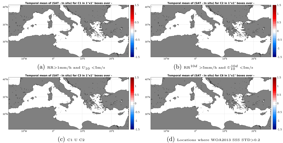
Figure 12: Temporal mean gridded over spatial boxes of size 1^\circ \times 1^\circ of \Delta SSS (Aquarius-L4-IPRC-V4-WEEKLY - TSG-LEGOS-DM) for 4 different subdatasets corresponding to:RR >1 mm/h and U_{10} < 5 m/s (a), RR ^{10d} > 5 mm/h and U_{10}^{10d} < 5 m/s (b), C1 U C2 (c),Locations where WOA2013 SSS STD >0.2 (d).
