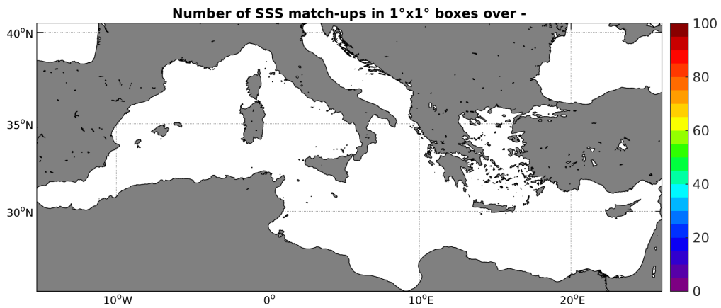
Figure 4: Number of SSS match-ups between TSG-GOSUD-Research-vessel SSS and the Aquarius-L4-IPRC-V4-WEEKLY SSS product for the Mediterranean Sea Pi-MEP region over 1^\circ \times 1^\circ boxes and for the full satellite product period.
