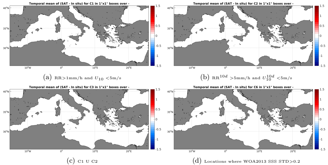
Figure 12: Temporal mean gridded over spatial boxes of size 1^\circ \times 1^\circ of \Delta SSS (Aquarius-L4-IPRC-V4-WEEKLY - TSG-GOSUD-Research-vessel) for 4 different subdatasets corresponding to: RR > 1\text{mm/h} and U_{10} < 5\text{m/s} (a), RR^{10d} > 5\text{mm/h} and U_{10}^{10d} < 5\text{m/s} (b), C1 U C2 (c), Locations where WOA2013 SSS STD > 0.2 (d).
