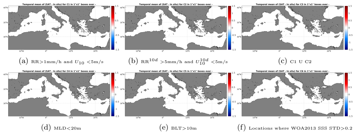
Figure 12: Temporal mean gridded over spatial boxes of size 1^\circ \times 1^\circ of \Delta SSS (Aquarius-L4-IPRC-V4-WEEKLY - Sea mammals) for 6 different subdatasets corresponding to: RR > 1\text{mm/h} and U_{10} < 5\text{m/s} (a), RR^{10d} > 5\text{mm/h} and U_{10}^{10d} < 5\text{m/s} (b), C1 U C2 (c), MLD < 20\text{m} (d), BLT > 10\text{m} (e), Locations where WOA2013 SSS STD > 0.2 (f).
