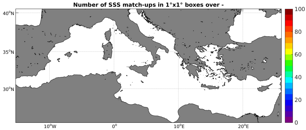
Figure 3: Number of SSS match-ups between Surface drifters SSS and the Aquarius-L4-IPRC-V4-WEEKLY SSS product for the Mediterranean Sea Pi-MEP region over 1^\circ \times 1^\circ boxes and for the full satellite product period.
