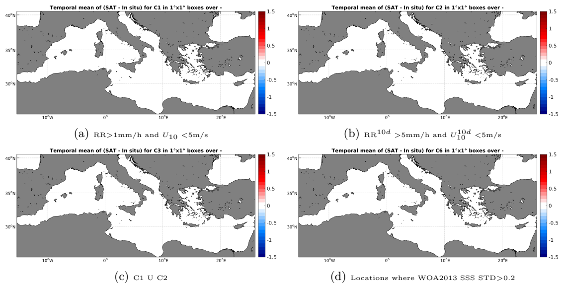
Figure 11: Temporal mean gridded over spatial boxes of size 1^\circ \times 1^\circ of \Delta SSS (Aquarius-L4-IPRC-V4-WEEKLY - Surface drifters) for 4 different subdatasets corresponding to:RR > 1 mm/h and U_{10} < 5 m/s (a), RR 10d > 5 mm/h and U_{10}^{10d} < 5 m/s (b), C1 U C2 (c),Locations where WOA2013 SSS STD > 0.2 (d).
