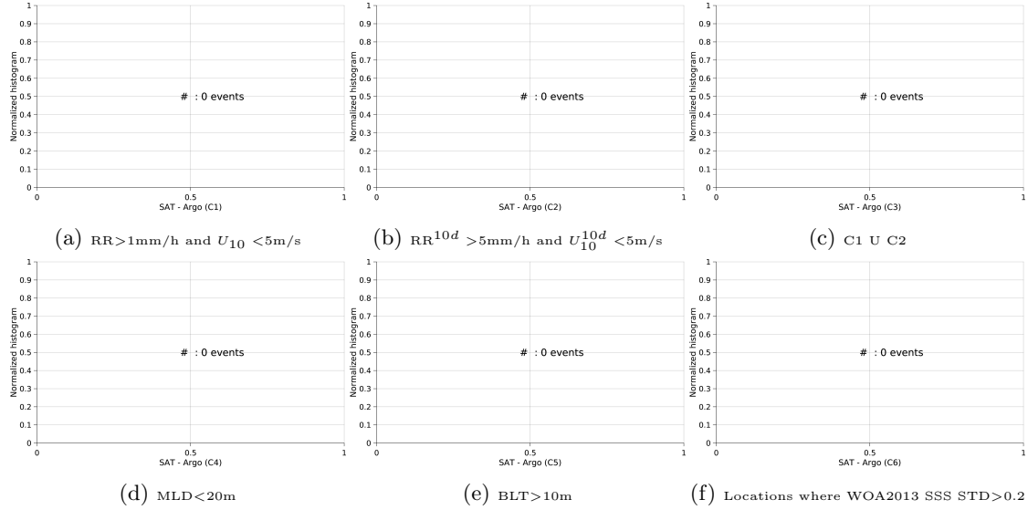
Figure 13: Normalized histogram of \Delta\text{SSS} (Aquarius-L4-IPRC-V4-WEEKLY - Argo) for 6 different subdatasets corresponding to: RR > 1\text{mm/h} and U_{10} < 5\text{m/s} (a), RR^{10d} > 5\text{mm/h} and U_{10}^{10d} < 5\text{m/s} (b), C1 U C2 (c), MLD < 20\text{m} (d), BLT > 10\text{m} (e), Locations where WOA2013 SSS STD > 0.2 (f).
