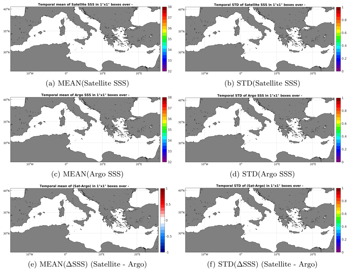
Figure 6: Temporal mean (left) and STD (right) of SSS from Aquarius-L4-IPRC-V4-WEEKLY (top), Argo (middle), and of \Delta SSS (Satellite - Argo). Only match-up pairs are used to generate these maps.
