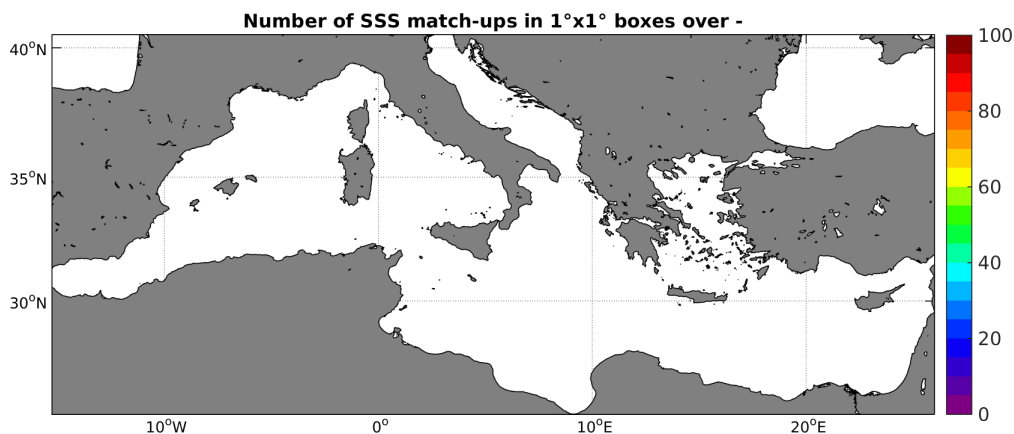
Figure 4: Number of SSS match-ups between Argo SSS and the Aquarius-L4-IPRC-V4-WEEKLY SSS product for the Mediterranean Sea Pi-MEP region over 1^\circ \times 1^\circ boxes and for the full satellite product period.
