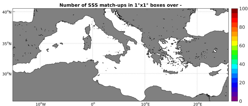
Figure 4: Number of SSS match-ups between TSG-SAMOS SSS and the Aquarius-L3-JPL-V4-7DAY-RUNNING SSS product for the Mediterranean Sea Pi-MEP region over 1^\circ \times 1^\circ boxes and for the full satellite product period.
