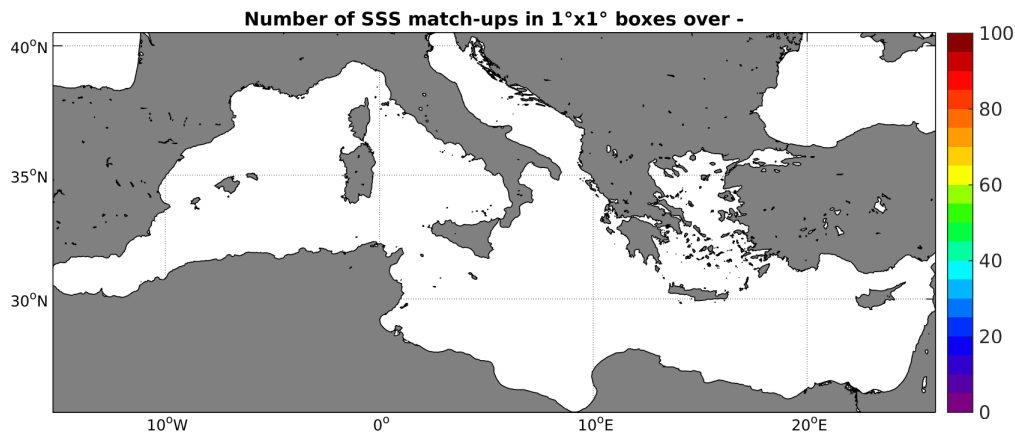
Figure 4: Number of SSS match-ups between TSG-LEGOS-DM SSS and the Aquarius-L3-JPL-V4-7DAY-RUNNING SSS product for the Mediterranean Sea Pi-MEP region over 1^\circ \times 1^\circ boxes and for the full satellite product period.
