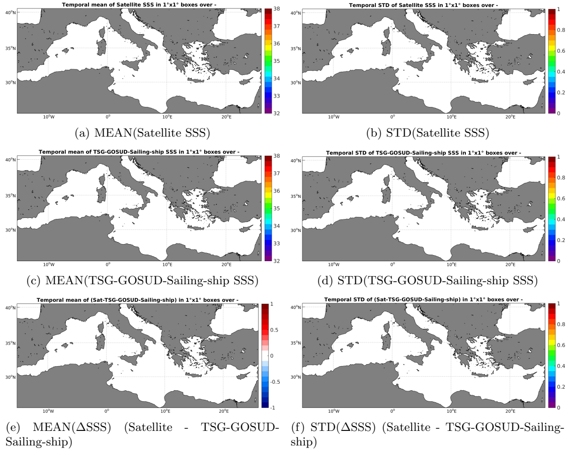
Figure 6: Temporal mean (left) and STD (right) of SSS from Aquarius-L3-JPL-V4-7DAY-RUNNING (top), TSG-GOSUD-Sailing-ship (middle), and of \Delta SSS (Satellite - TSG-GOSUD-Sailing-ship). Only match-up pairs are used to generate these maps.
