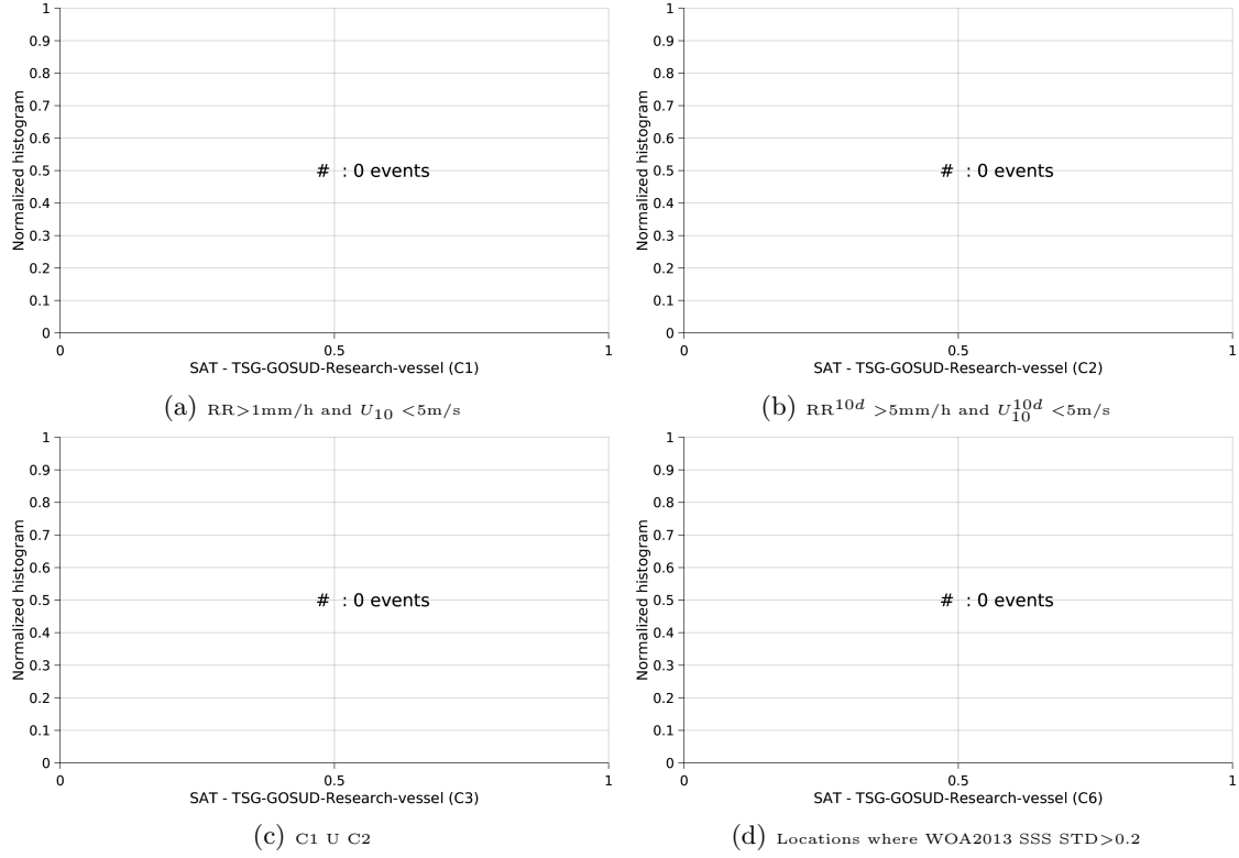
Figure 13: Normalized histogram of \Delta\text{SSS} (Aquarius-L3-JPL-V4-7DAY-RUNNING - TSG-GOSUD-Research-vessel) for 6 different subdatasets corresponding to: RR > 1\text{mm/h} and U_{10} < 5\text{m/s} (a), RR^{10d} > 5\text{mm/h} and U_{10}^{10d} < 5\text{m/s} (b), C1 \cup C2 (c), Locations where WOA2013 SSS STD > 0.2 (d).
