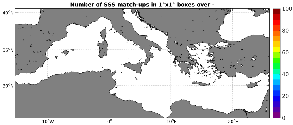
Figure 4: Number of SSS match-ups between Argo SSS and the Aquarius-L3-JPL-V4-7DAY-RUNNING SSS product for the Mediterranean Sea Pi-MEP region over 1^\circ \times 1^\circ boxes and for the full satellite product period.
