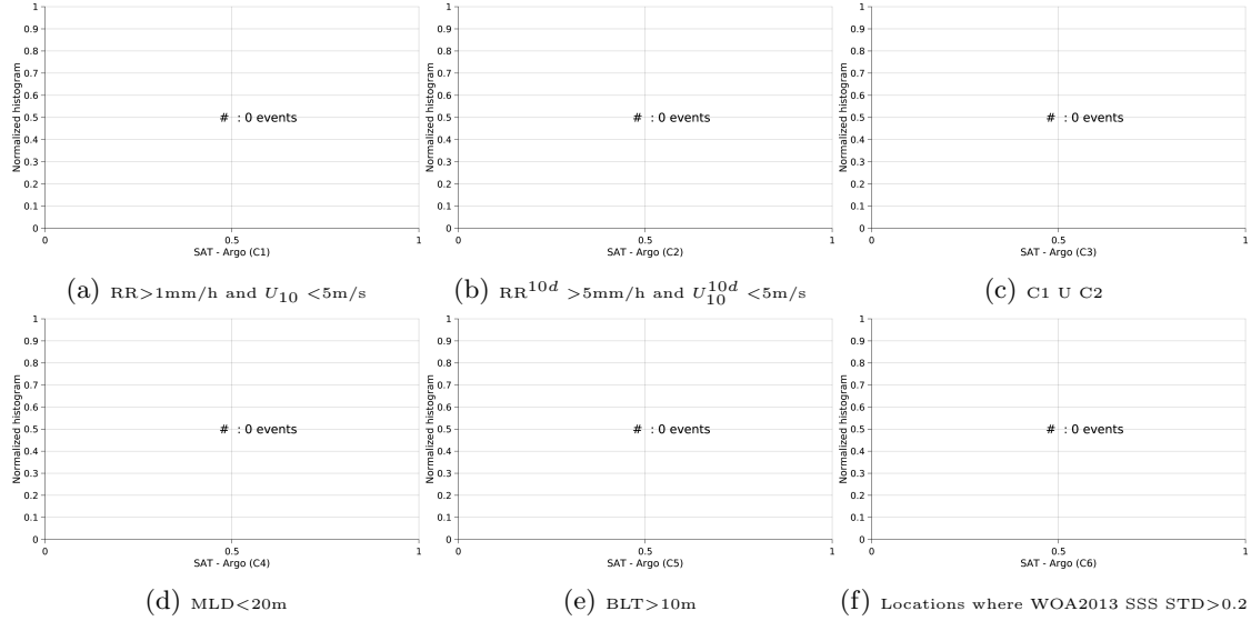
Figure 13: Normalized histogram of \Delta\text{SSS} (Aquarius-L3-JPL-V4-7DAY-RUNNING - Argo) for 6 different subdatasets corresponding to: RR > 1\text{mm/h} and U_{10} < 5\text{m/s} (a), RR^{10d} > 5\text{mm/h} and U_{10}^{10d} < 5\text{m/s} (b), C1 U C2 (c), MLD < 20\text{m} (d), BLT > 10\text{m} (e), Locations where WOA2013 SSS STD > 0.2 (f).
