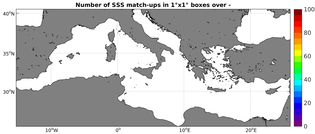
Figure 4: Number of SSS match-ups between Sea mammals SSS and the AQUARIUS-L2-JPL-V4 SSS product for the Mediterranean Sea Pi-MEP region over 1^\circ \times 1^\circ boxes and for the full satellite product period.
