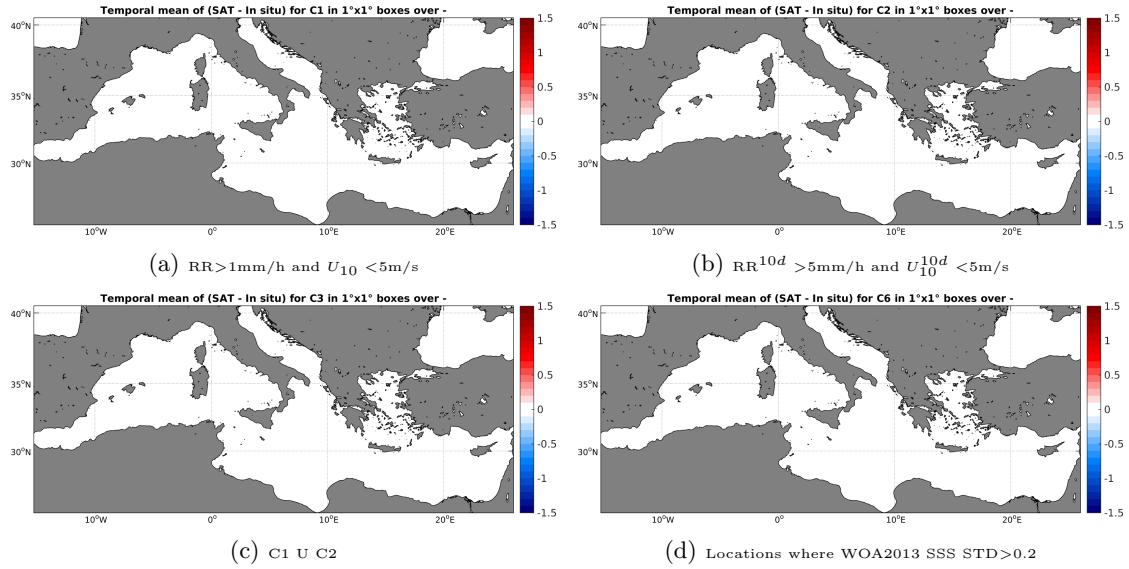
Figure 11: Temporal mean gridded over spatial boxes of size 1^\circ \times 1^\circ of \Delta SSS (AQUARIUS-L2-JPL-V4 - Surface drifters) for 4 different subdatasets corresponding to: RR > 1\text{mm/h} and U_{10} < 5\text{m/s} (a), RR^{10d} > 5\text{mm/h} and U_{10}^{10d} < 5\text{m/s} (b), C1 U C2 (c), Locations where WOA2013 SSS STD > 0.2 (d).
