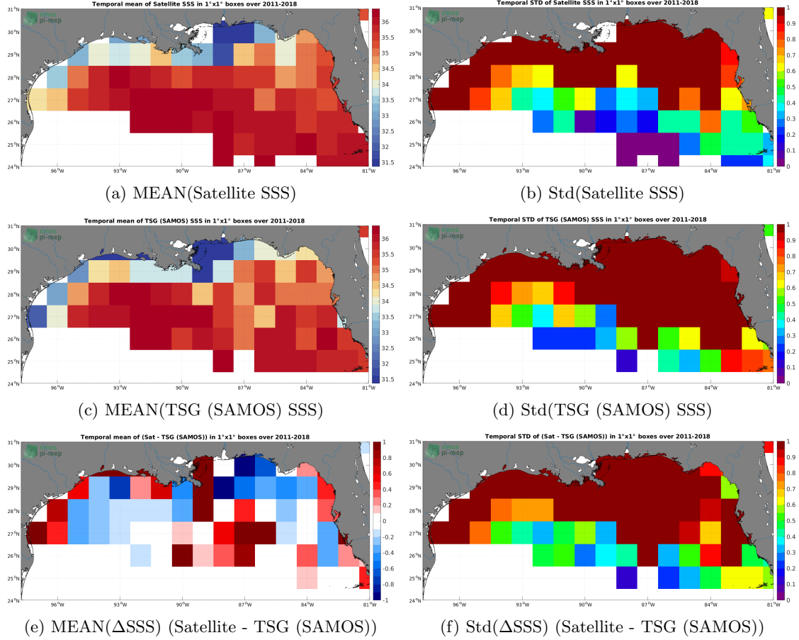
Figure 6: Temporal mean (left) and Std (right) of SSS from SMOS and SMAP SSS L4 OI v1 - 7 Days (LOPS) (top), TSG (SAMOS) (middle), and of \Delta\text{SSS} (Satellite - TSG (SAMOS)). Only match-up pairs are used to generate these maps.
