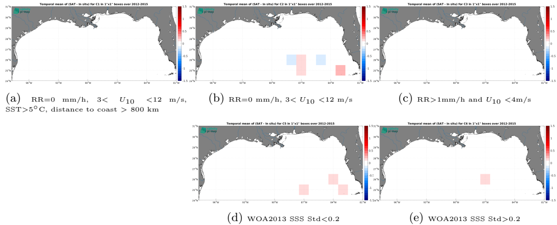
Figure 12: Temporal mean gridded over spatial boxes of size 1^{\circ}\times 1^{\circ} of \Delta SSS (SMOS and SMAP SSS L4 OI v1 - 7 Days (LOPS) - TSG (GOSUD-Sailing-ship)) for 5 different subdatasets corresponding to:RR=0 mm/h, 3 < U_{10} < 12 m/s, SST > 5^{\circ}\text{C} , distance to coast > 800 km (a), RR=0 mm/h, 3 < U_{10} < 12 m/s (b), RR > 1 mm/h and U_{10} < 4 m/s (c), WOA2013 SSS Std < 0.2 (d), WOA2013 SSS Std > 0.2 (e).
