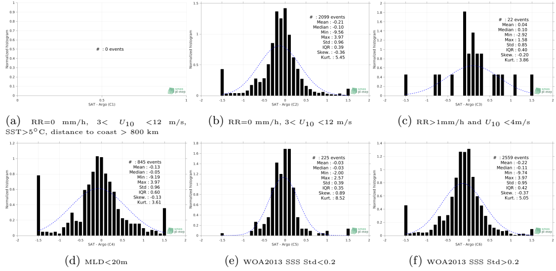
Figure 13: Normalized histogram of \Delta\text{SSS} (SMOS and SMAP SSS L4 OI v1 - 7 Days (LOPS) - Argo) for 6 different subdatasets corresponding to: \text{RR}=0 mm/h, 3 < U_{10} < 12 m/s, \text{SST} > 5^\circ\text{C} , distance to coast > 800 km (a), \text{RR}=0 mm/h, 3 < U_{10} < 12 m/s (b), \text{RR} > 1 mm/h and U_{10} < 4 m/s (c), \text{MLD} < 20 m (d), \text{WOA2013 SSS Std} < 0.2 (e), \text{WOA2013 SSS Std} > 0.2 (f).
