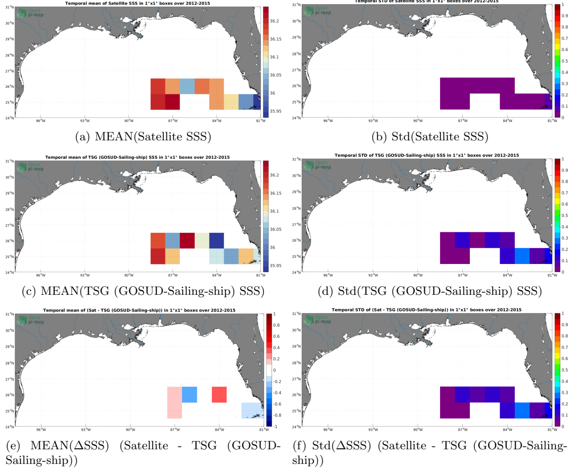
Figure 6: Temporal mean (left) and Std (right) of SSS from SMOS SSS L4 v1 - Weekly (CMEMS-CNR) (top), TSG (GOSUD-Sailing-ship) (middle), and of \Delta SSS (Satellite - TSG (GOSUD-Sailing-ship)). Only match-up pairs are used to generate these maps.
