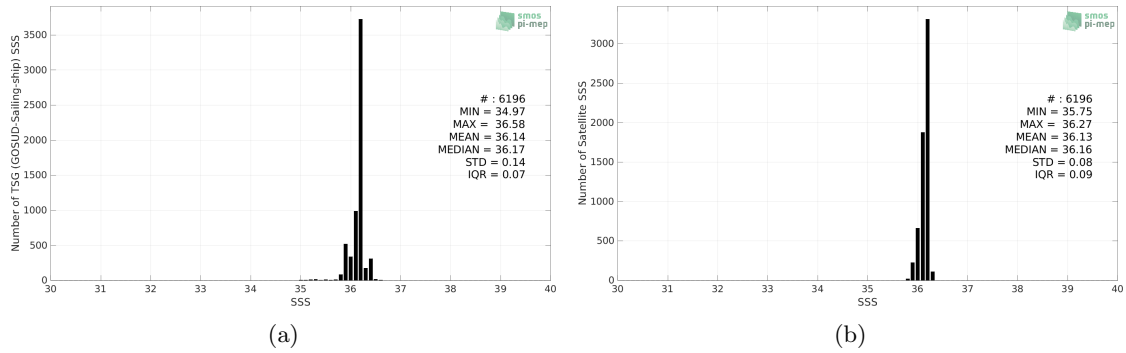
Figure 2: Histograms of SSS from TSG (GOSUD-Sailing-ship) (a) and SMOS SSS L4 v1 - Weekly (CMEMS-CNR) (b) considering all match-up pairs per bins of 0.1 over the Mississippi river plume Pi-MEP region and for the full satellite product period.
