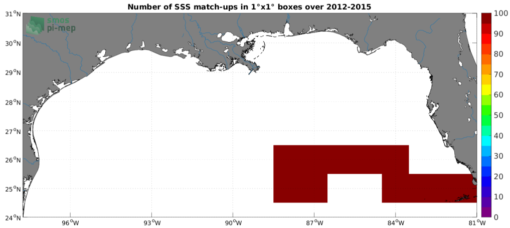
Figure 4: Number of SSS match-ups between TSG (GOSUD-Sailing-ship) SSS and the SMOS SSS L4 v1 - Weekly (CMEMS-CNR) SSS product for the Mississippi river plume Pi-MEP region over 1^\circ \times 1^\circ boxes and for the full satellite product period.
