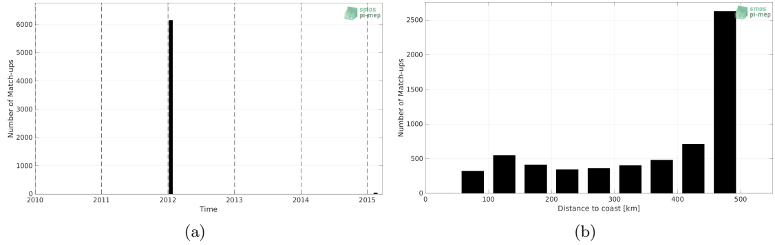
Figure 1: Number of match-ups between TSG (GOSUD-Sailing-ship) and SMOS SSS L4 v1 - Weekly (CMEMS-CNR) SSS as a function of time (a) and as function of the distance to coast (b) over the Mississippi river plume Pi-MEP region and for the full satellite product period.
