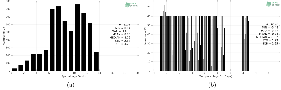
Figure 5: Histograms of the spatial (a) and temporal (b) lags between the location/time of the TSG (GOSUD-Sailing-ship) measurement and the date of the corresponding SMOS SSS L4 v1 - Weekly (CMEMS-CNR) SSS pixel.
