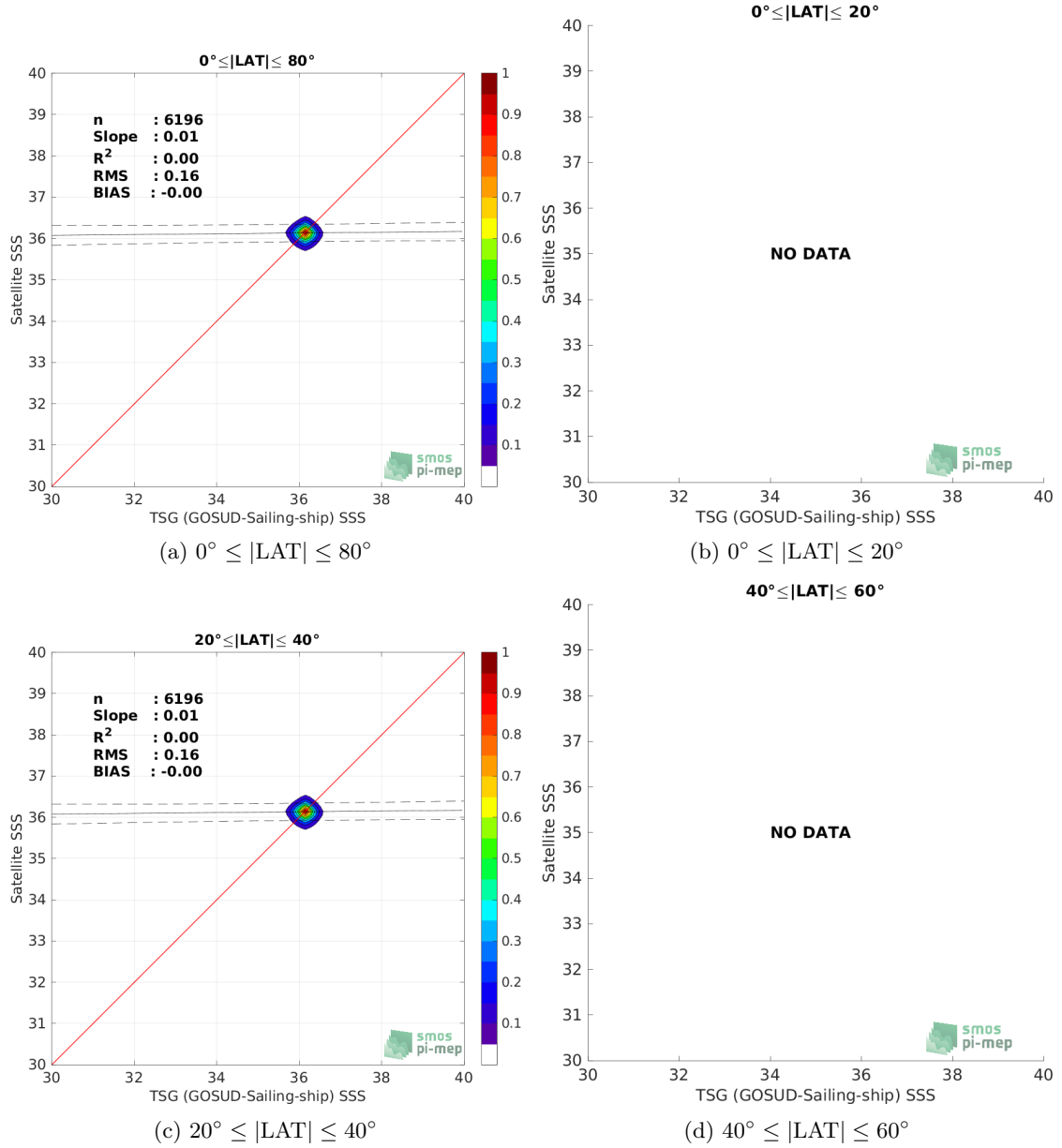
Figure 9: Contour maps of the concentration of SMOS SSS L4 v1 - Weekly (CMEMS-CNR) SSS (y-axis) versus TSG (GOSUD-Sailing-ship) SSS (x-axis) at match-up pairs for different latitude bands. For each plot, the red line shows x=y . The black thin and dashed lines indicate a linear fit through the data cloud and the \pm 95\% confidence levels, respectively. The number match-up pairs n , the slope and R^2 coefficient of the linear fit, the root mean square (RMS) and the mean bias between satellite and in situ data are indicated for each latitude band in each plots.
