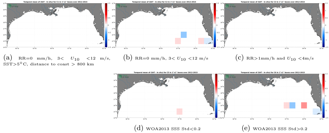
Figure 12: Temporal mean gridded over spatial boxes of size 1^{\circ} \times 1^{\circ} of \Delta SSS (SMOS SSS L4 v1 - Weekly (CMEMS-CNR) - TSG (GOSUD-Sailing-ship)) for 5 different subdatasets corresponding to:RR=0 mm/h, 3 < U_{10} < 12 m/s, SST >5^{\circ}\text{C} , distance to coast > 800 km (a), RR=0 mm/h, 3 < U_{10} < 12 m/s (b), RR >1 mm/h and U_{10} < 4 m/s (c), WOA2013 SSS Std <0.2 (d), WOA2013 SSS Std >0.2 (e).
