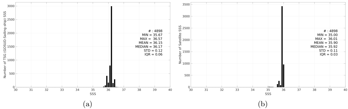
Figure 3: Histograms of SSS from TSG (GOSUD-Sailing-ship) (a) and SMOS SSS L4 v1 - Monthly (CMEMS-CNR) (b) considering all match-up pairs per bins of 0.1 over the Mississippi river plume Pi-MEP region and for the full satellite product period.
