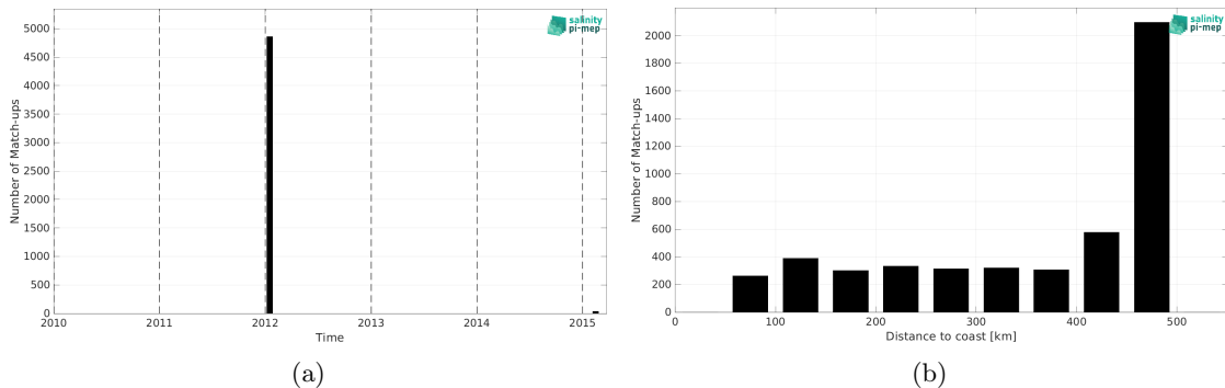
Figure 2: Number of match-ups between TSG (GOSUD-Sailing-ship) and SMOS SSS L4 v1 - Monthly (CMEMS-CNR) SSS as a function of time (a) and as function of the distance to coast (b) over the Mississippi river plume Pi-MEP region and for the full satellite product period.
