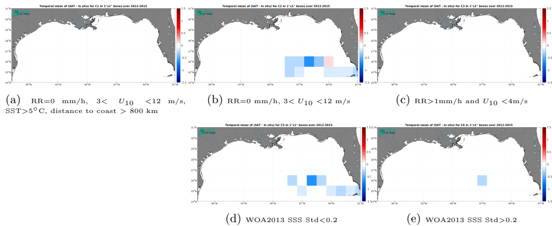
Figure 14: Temporal mean gridded over spatial boxes of size 1^\circ \times 1^\circ of \Delta SSS (SMOS SSS L4 v1 - Monthly (CMEMS-CNR) - TSG (GOSUD-Sailing-ship)) for 5 different subdatasets corresponding to: RR=0 mm/h, 3 < U_{10} < 12 m/s, SST > 5°C, distance to coast > 800 km (a), RR=0 mm/h, 3 < U_{10} < 12 m/s (b), RR > 1mm/h and U_{10} < 4 m/s (c), WOA2013 SSS Std < 0.2 (d), WOA2013 SSS Std > 0.2 (e).
