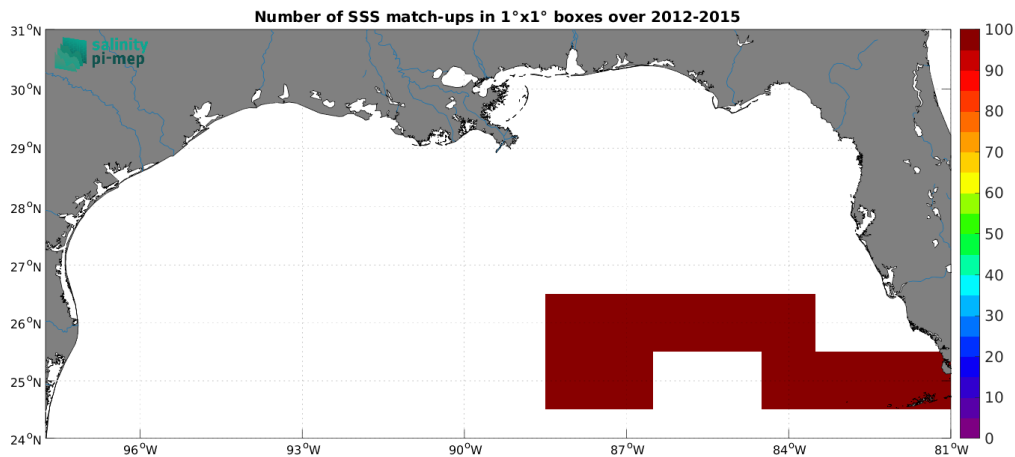
Figure 5: Number of SSS match-ups between TSG (GOSUD-Sailing-ship) SSS and the SMOS SSS L4 v1 - Monthly (CMEMS-CNR) SSS product for the Mississippi river plume Pi-MEP region over 1^\circ \times 1^\circ boxes and for the full satellite product period.
