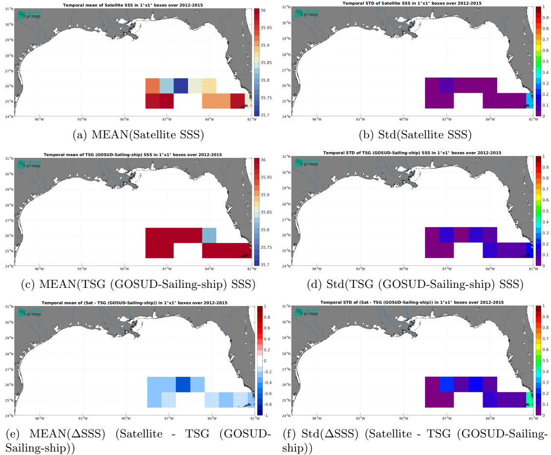
Figure 7: Temporal mean (left) and Std (right) of SSS from SMOS SSS L4 v1 - Monthly (CMEMS-CNR) (top), TSG (GOSUD-Sailing-ship) (middle), and of \Delta\text{SSS} (Satellite - TSG (GOSUD-Sailing-ship)). Only match-up pairs are used to generate these maps.
