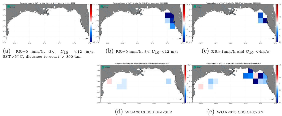
Figure 14: Temporal mean gridded over spatial boxes of size 1^\circ \times 1^\circ of \Delta SSS (SMOS SSS L4 v1 - Monthly (CMEMS-CNR) - Saildrone) for 5 different subdatasets corresponding to: RR=0 mm/h, 3 < U_{10} < 12 m/s, SST > 5°C, distance to coast > 800 km (a), RR=0 mm/h, 3 < U_{10} < 12 m/s (b), RR > 1mm/h and U_{10} < 4 m/s (c), WOA2013 SSS Std < 0.2 (d), WOA2013 SSS Std > 0.2 (e).
