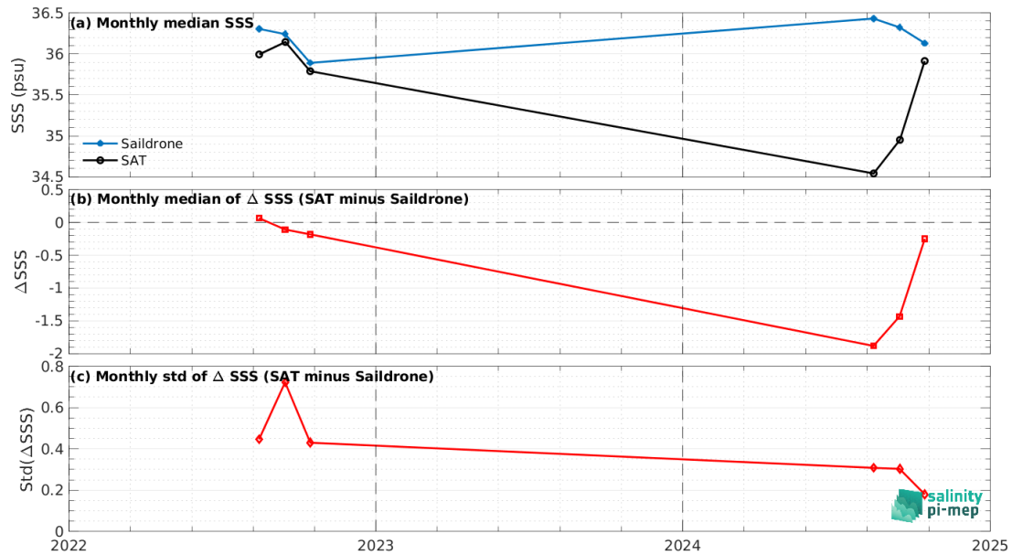
Figure 8: Time series of the monthly median SSS (top), median of \Delta SSS (Satellite - Ssaldrone) and Std of \Delta SSS (Satellite - Ssaldrone) over the Mississippi river plume Pi-MEP region considering all match-ups collected by the Pi-MEP.
