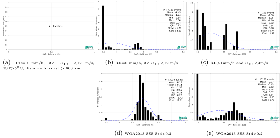
Figure 15: Normalized histogram of \Delta\text{SSS} (SMOS SSS L4 v1 - Monthly (CMEMS-CNR) - Saildrone) for 5 different subdatasets corresponding to: RR=0 mm/h, 3 < U_{10} < 12 m/s, SST > 5^\circ\text{C} , distance to coast > 800 km (a), RR=0 mm/h, 3 < U_{10} < 12 m/s (b), RR > 1\text{mm/h} and U_{10} < 4\text{m/s} (c), WOA2013 SSS Std < 0.2 (d), WOA2013 SSS Std > 0.2 (e).
