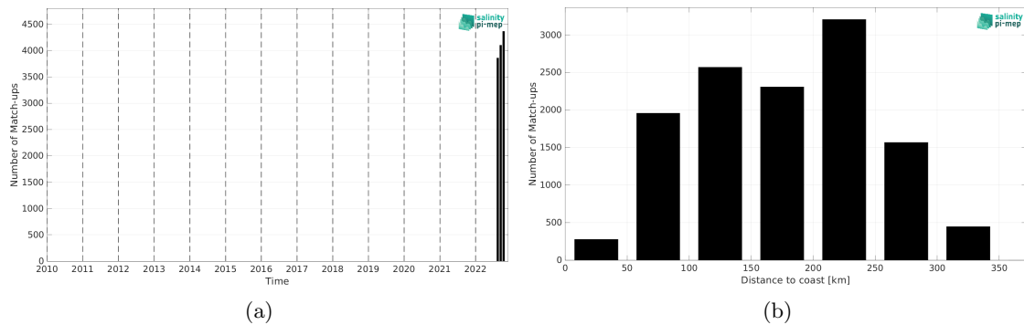
Figure 2: Number of match-ups between Saildrone and SMOS SSS L4 v1 - Monthly (CMEMS-CNR) SSS as a function of time (a) and as function of the distance to coast (b) over the Mississippi river plume Pi-MEP region and for the full satellite product period.
