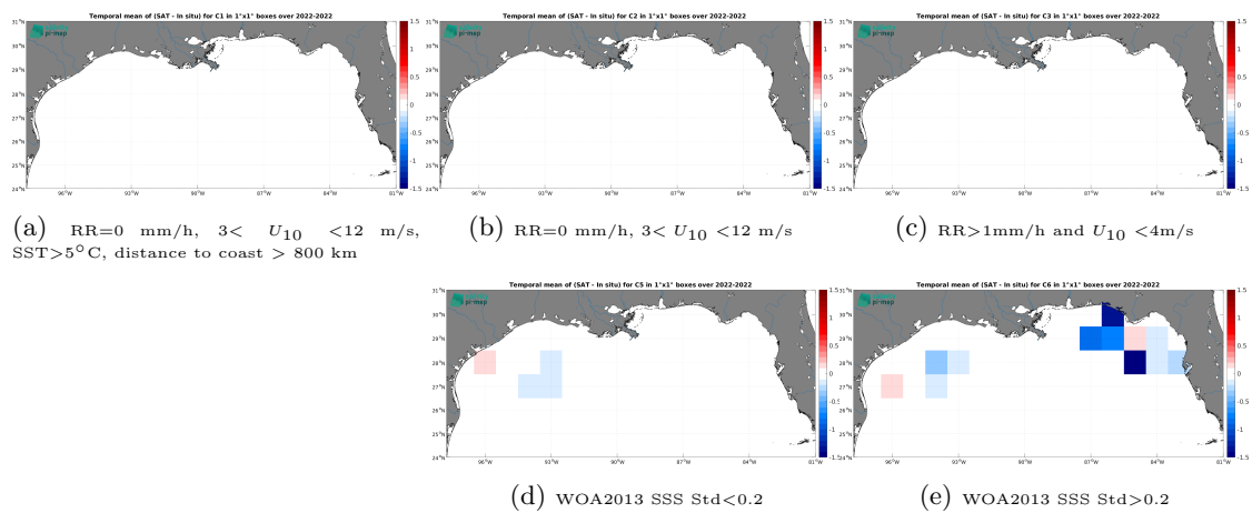
Figure 14: Temporal mean gridded over spatial boxes of size 1^\circ \times 1^\circ of \Delta\text{SSS} (SMOS SSS L4 v1 - Monthly (CMEMS-CNR) - Saildrone) for 5 different subdatasets corresponding to:RR=0 mm/h, 3 < U_{10} < 12 m/s, SST >5^\circ\text{C} , distance to coast > 800 km (a), RR=0 mm/h, 3 < U_{10} < 12 m/s (b), RR >1 mm/h and U_{10} < 4 m/s (c), WOA2013 SSS Std <0.2 (d), WOA2013 SSS Std >0.2 (e).
