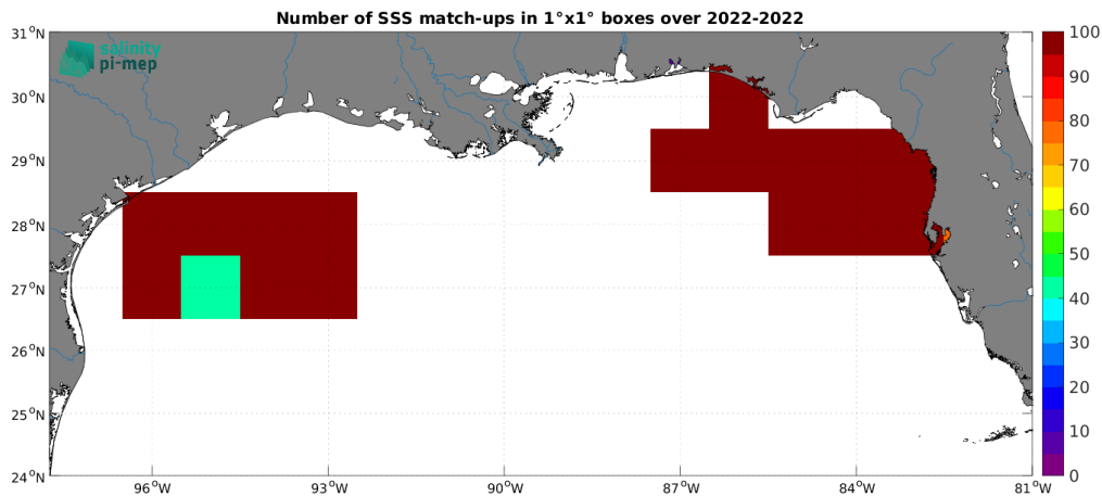
Figure 5: Number of SSS match-ups between Saildrone SSS and the SMOS SSS L4 v1 - Monthly (CMEMS-CNR) SSS product for the Mississippi river plume Pi-MEP region over 1^\circ \times 1^\circ boxes and for the full satellite product period.
