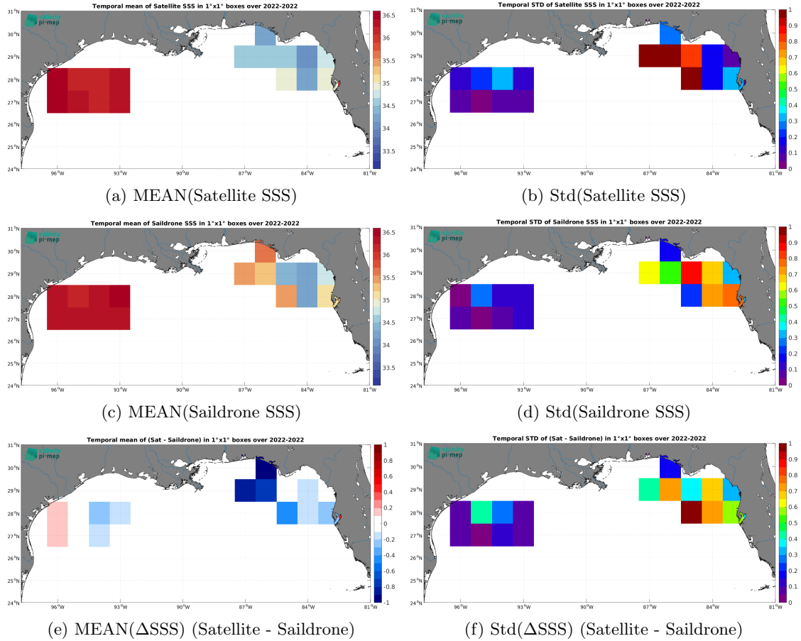
Figure 7: Temporal mean (left) and Std (right) of SSS from SMOS SSS L4 v1 - Monthly (CMEMS-CNR) (top), Sairdrone (middle), and of \Delta SSS (Satellite - Sairdrone). Only match-up pairs are used to generate these maps.
