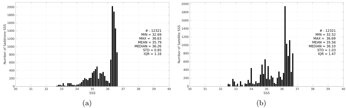
Figure 3: Histograms of SSS from Saildrone (a) and SMOS SSS L4 v1 - Monthly (CMEMS-CNR) (b) considering all match-up pairs per bins of 0.1 over the Mississippi river plume Pi-MEP region and for the full satellite product period.
