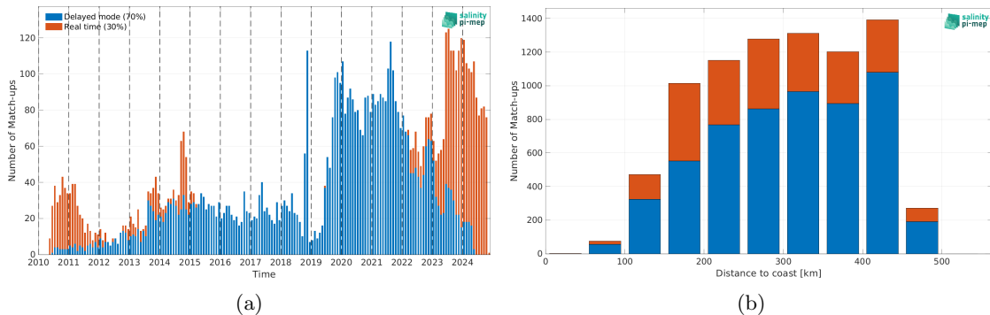
Figure 2: Number of match-ups between Argo and SMOS SSS L4 v1 - Monthly (CMEMS-CNR) SSS as a function of time (a) and as function of the distance to coast (b) over the Mississippi river plume Pi-MEP region and for the full satellite product period.
