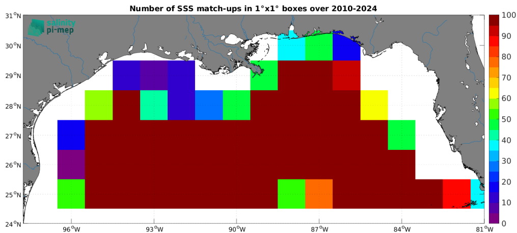
Figure 5: Number of SSS match-ups between Argo SSS and the SMOS SSS L4 v1 - Monthly (CMEMS-CNR) SSS product for the Mississippi river plume Pi-MEP region over 1^\circ \times 1^\circ boxes and for the full satellite product period.
