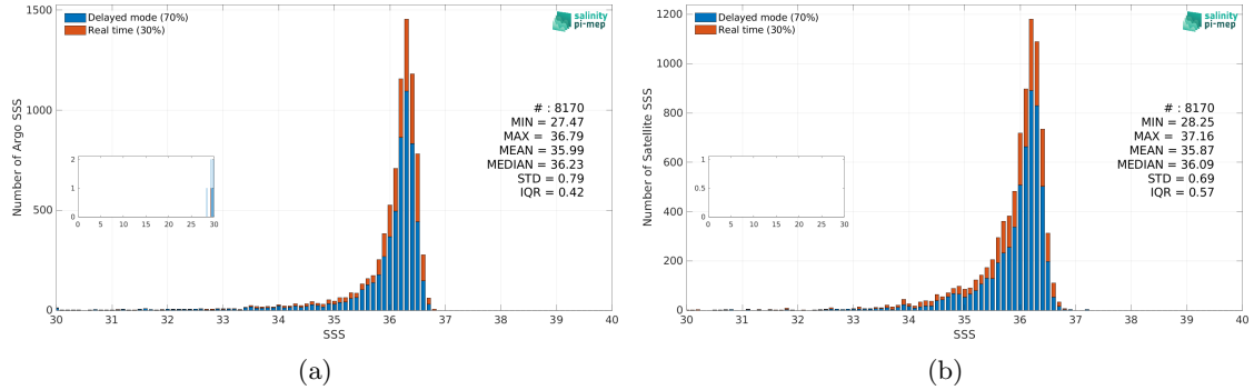
Figure 3: Histograms of SSS from Argo (a) and SMOS SSS L4 v1 - Monthly (CMEMS-CNR) (b) considering all match-up pairs per bins of 0.1 over the Mississippi river plume Pi-MEP region and for the full satellite product period.
