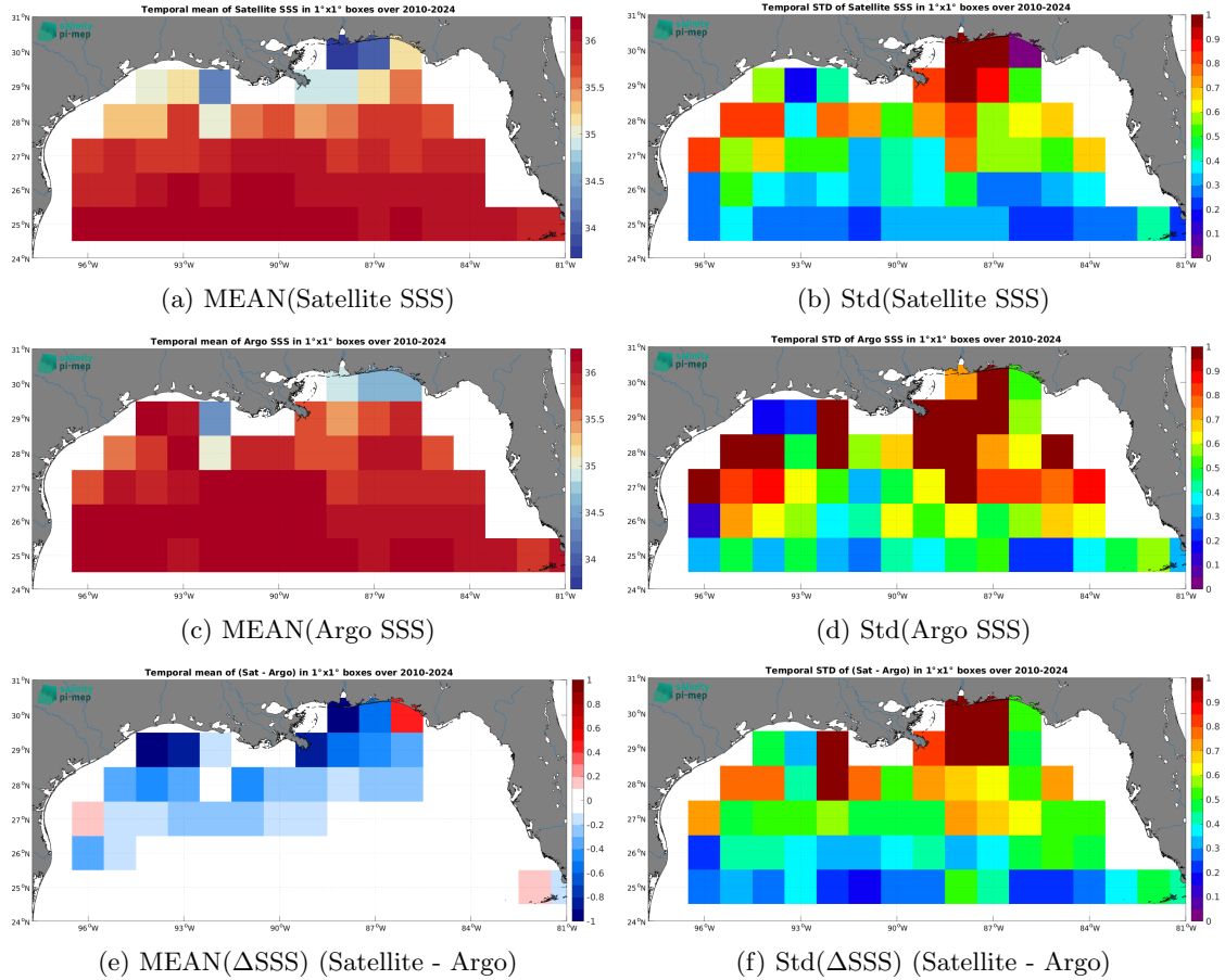
Figure 7: Temporal mean (left) and Std (right) of SSS from SMOS SSS L4 v1 - Monthly (CMEMS-CNR) (top), Argo (middle), and of \Delta\text{SSS} (Satellite - Argo). Only match-up pairs are used to generate these maps.
