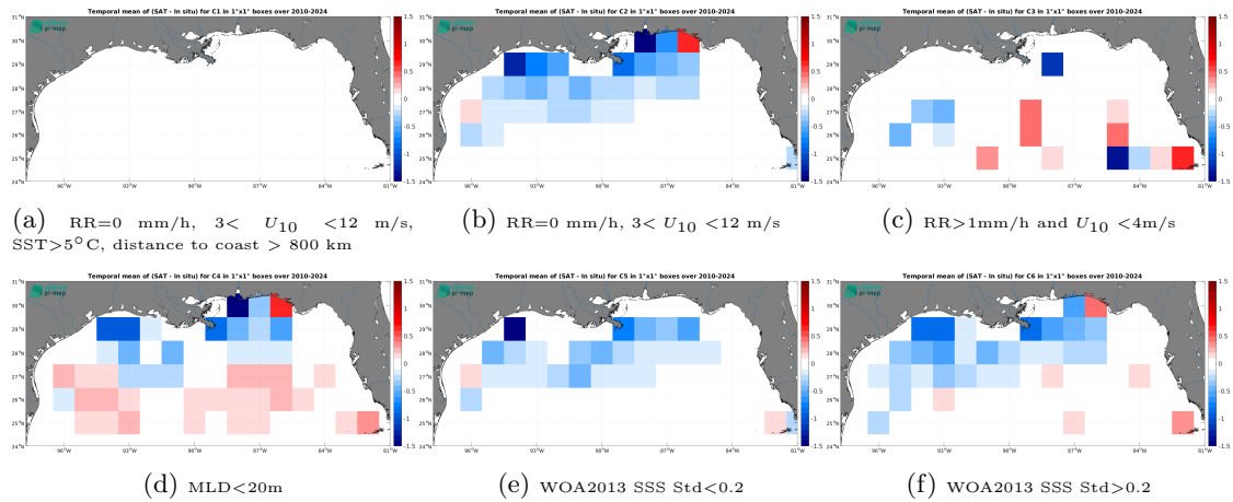
Figure 14: Temporal mean gridded over spatial boxes of size 1^\circ \times 1^\circ of \Delta SSS (SMOS SSS L4 v1 - Monthly (CMEMS-CNR) - Argo) for 6 different subdatasets corresponding to:RR=0 mm/h, 3 < U_{10} < 12 m/s, SST >5^\circ C, distance to coast > 800 km (a), RR=0 mm/h, 3 < U_{10} < 12 m/s (b), RR >1 mm/h and U_{10} < 4 m/s (c),MLD <20 m (d),WOA2013 SSS Std <0.2 (e),WOA2013 SSS Std >0.2 (f).
