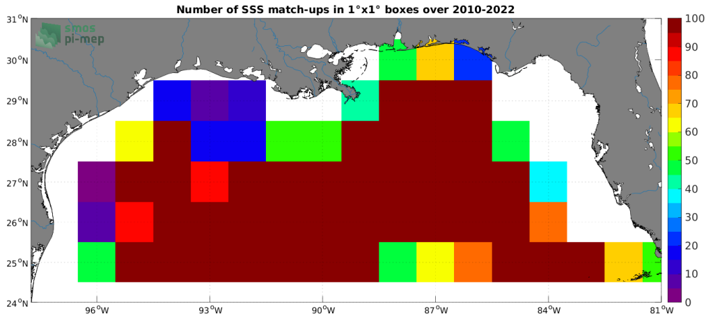
Figure 4: Number of SSS match-ups between Argo SSS and the SMOS SSS L4 v1 - Monthly (CMEMS-CNR) SSS product for the Mississippi river plume Pi-MEP region over 1^{\circ} \times 1^{\circ} boxes and for the full satellite product period.
