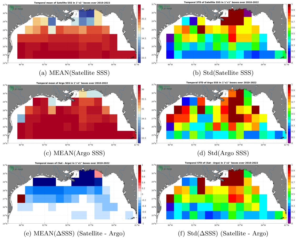
Figure 6: Temporal mean (left) and Std (right) of SSS from SMOS SSS L4 v1 - Monthly (CMEMS-CNR) (top), Argo (middle), and of \Delta SSS (Satellite - Argo). Only match-up pairs are used to generate these maps.
