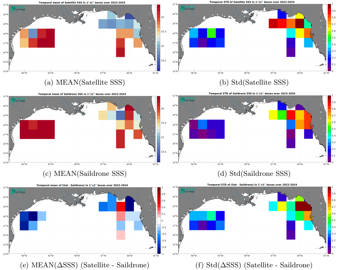
Figure 7: Temporal mean (left) and Std (right) of SSS from SMOS SSS L4 v1 - Daily (CMEMS-CNR) (top), Saildrone (middle), and of \Delta\text{SSS} (Satellite - Saildrone). Only match-up pairs are used to generate these maps.
