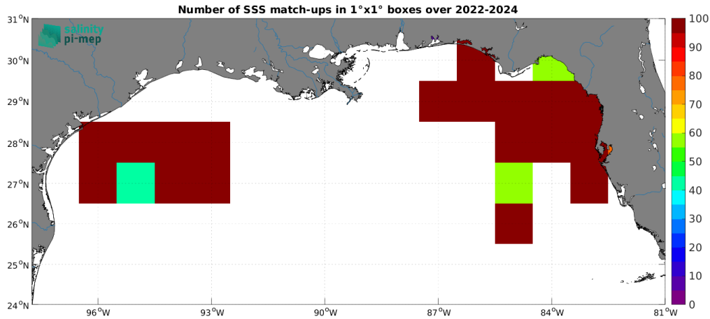
Figure 5: Number of SSS match-ups between Saildrone SSS and the SMOS SSS L4 v1 - Daily (CMEMS-CNR) SSS product for the Mississippi river plume Pi-MEP region over 1^\circ \times 1^\circ boxes and for the full satellite product period.
