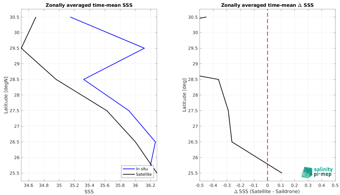
Figure 9: Left panel: Zonal mean SSS from SMOS SSS L4 v1 - Daily (CMEMS-CNR) satellite product (black) and from Sairdrone (blue). Right panel: Zonal mean of \Delta SSS (Satellite - Sairdrone) for all the collected Pi-MEP match-up pairs estimated over the full satellite product period.
