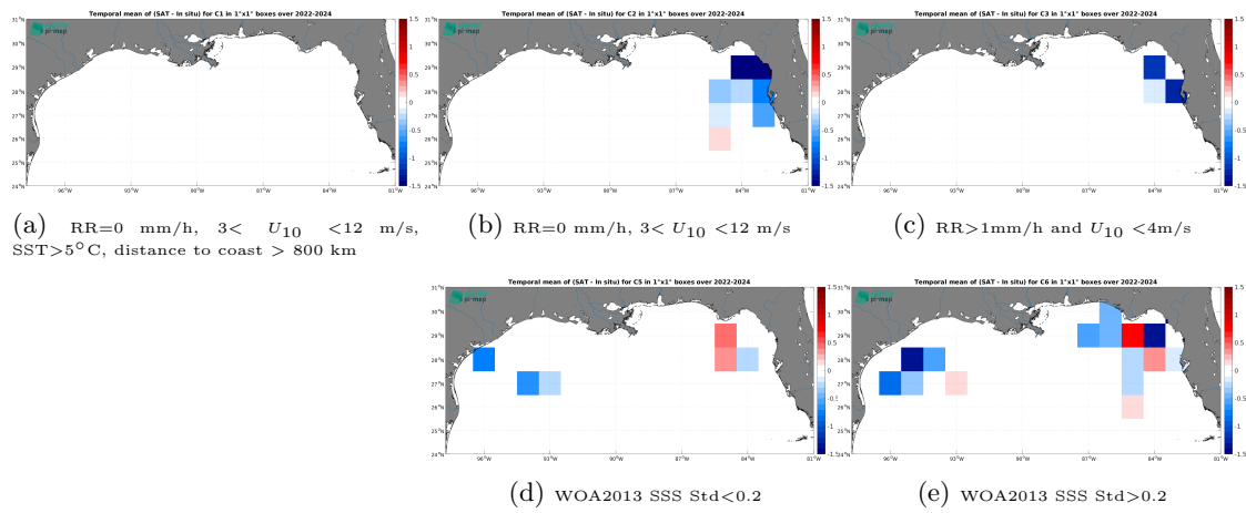
Figure 14: Temporal mean gridded over spatial boxes of size 1^\circ \times 1^\circ of \Delta SSS (SMOS SSS L4 v1 - Daily (CMEMS-CNR) - Saildrone) for 5 different subdatasets corresponding to:RR=0 mm/h, 3 < U_{10} < 12 m/s, SST > 5°C, distance to coast > 800 km (a), RR=0 mm/h, 3 < U_{10} < 12 m/s (b), RR > 1mm/h and U_{10} < 4 m/s (c), WOA2013 SSS Std < 0.2 (d), WOA2013 SSS Std > 0.2 (e).
