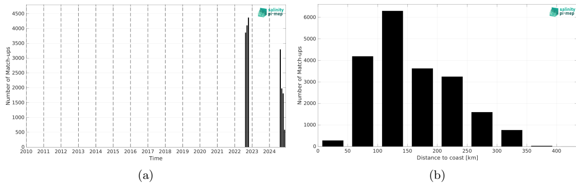
Figure 2: Number of match-ups between Saildrone and SMOS SSS L4 v1 - Daily (CMEMS-CNR) SSS as a function of time (a) and as function of the distance to coast (b) over the Mississippi river plume Pi-MEP region and for the full satellite product period.
