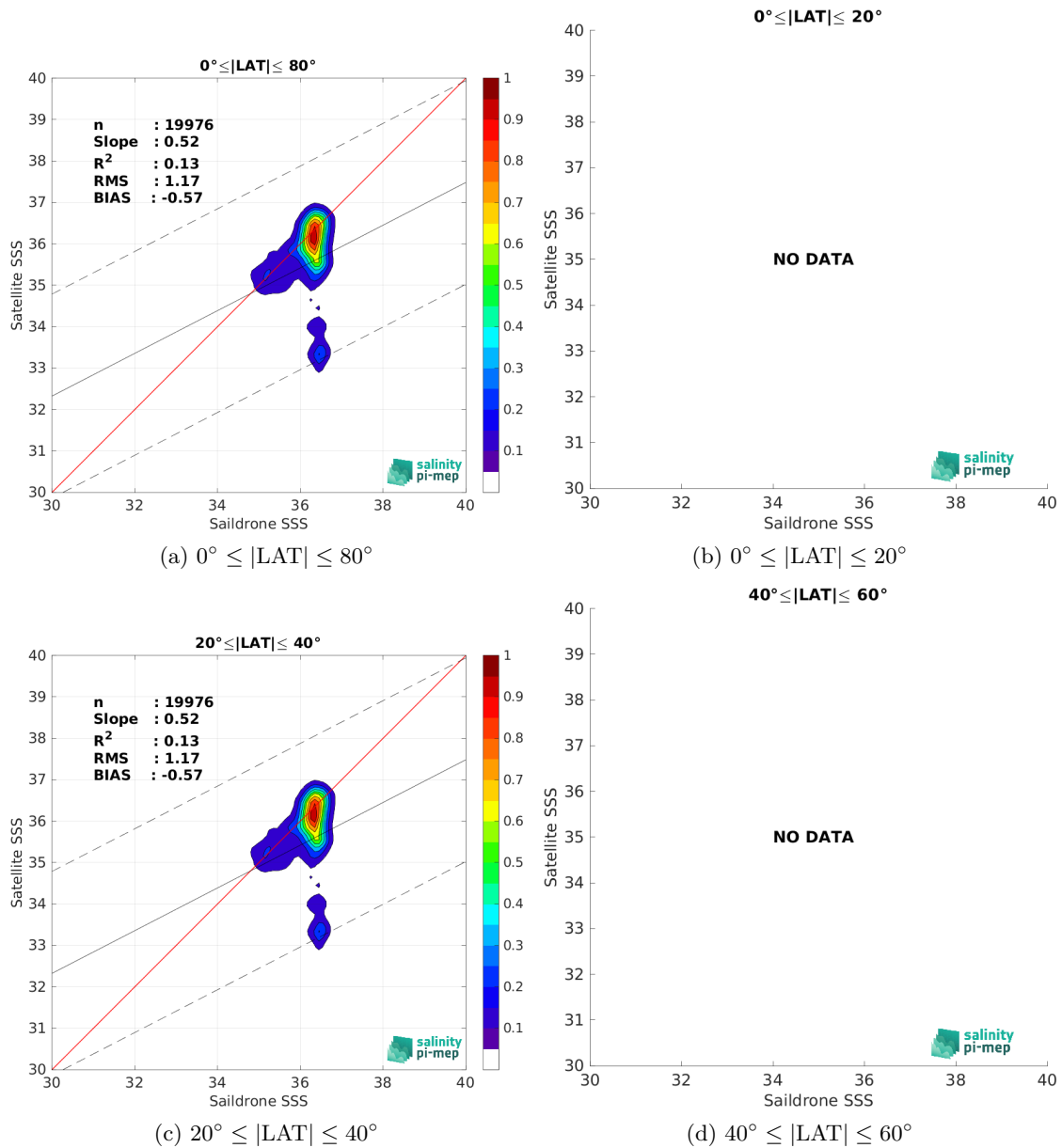
Figure 10: Contour maps of the concentration of SMOS SSS L4 v1 - Daily (CMEMS-CNR) SSS (y-axis) versus Saildrone SSS (x-axis) at match-up pairs for different latitude bands. For each plot, the red line shows x=y . The black thin and dashed lines indicate a linear fit through the data cloud and the \pm 95\% confidence levels, respectively. The number match-up pairs n , the slope and R^2 coefficient of the linear fit, the root mean square (RMS) and the mean bias between satellite and in situ data are indicated for each latitude band in each plots.
