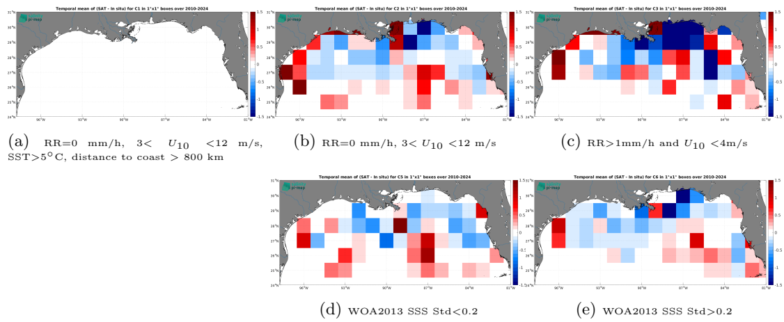
Figure 14: Temporal mean gridded over spatial boxes of size 1^\circ \times 1^\circ of \Delta SSS (SMOS SSS L4 OI v346 - Weekly (CMEMS-CATDS-LOPS) - TSG (SAMOS)) for 5 different subdatasets corresponding to:RR=0 mm/h, 3 < U_{10} < 12 m/s, SST > 5°C, distance to coast > 800 km (a), RR=0 mm/h, 3 < U_{10} < 12 m/s (b), RR > 1mm/h and U_{10} < 4 m/s (c), WOA2013 SSS Std < 0.2 (d), WOA2013 SSS Std > 0.2 (e).
