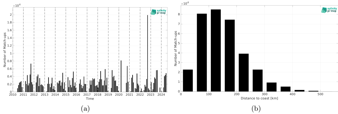
Figure 2: Number of match-ups between TSG (SAMOS) and SMOS SSS L4 OI v346 - Weekly (CMEMS-CATDS-LOPS) SSS as a function of time (a) and as function of the distance to coast (b) over the Mississippi river plume Pi-MEP region and for the full satellite product period.
