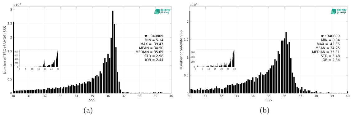
Figure 3: Histograms of SSS from TSG (SAMOS) (a) and SMOS SSS L4 OI v346 - Weekly (CMEMS-CATDS-LOPS) (b) considering all match-up pairs per bins of 0.1 over the Mississippi river plume Pi-MEP region and for the full satellite product period.
