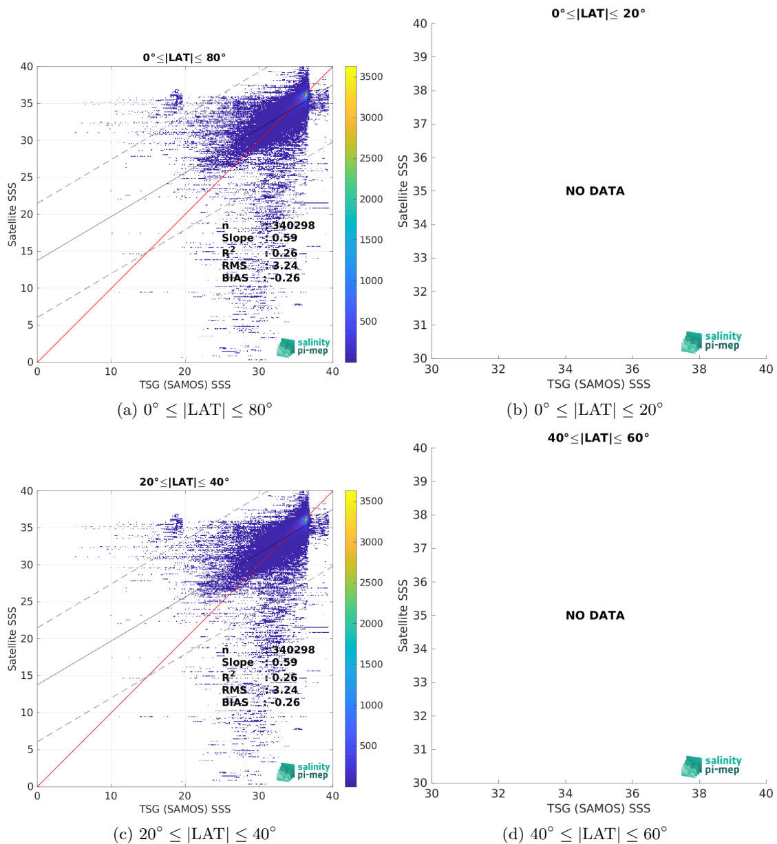
Figure 10: Contour maps of the concentration of SMOS SSS L4 OI v346 - Weekly (CMEMS-CATDS-LOPS) SSS (y-axis) versus TSG (SAMOS) SSS (x-axis) at match-up pairs for different latitude bands. For each plot, the red line shows x=y . The black thin and dashed lines indicate a linear fit through the data cloud and the \pm 95\% confidence levels, respectively. The number match-up pairs n , the slope and R^2 coefficient of the linear fit, the root mean square (RMS) and the mean bias between satellite and in situ data are indicated for each latitude band in each plots.
