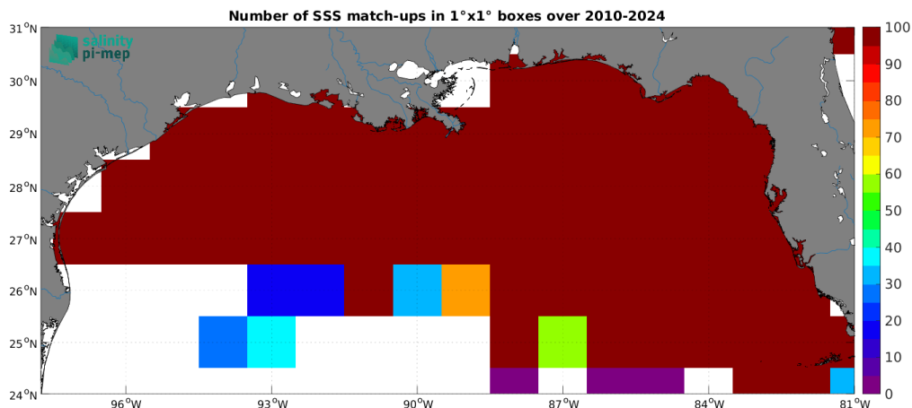
Figure 5: Number of SSS match-ups between TSG (SAMOS) SSS and the SMOS SSS L4 OI v346 - Weekly (CMEMS-CATDS-LOPS) SSS product for the Mississippi river plume Pi-MEP region over 1^\circ \times 1^\circ boxes and for the full satellite product period.
