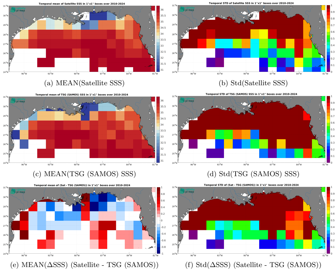
Figure 7: Temporal mean (left) and Std (right) of SSS from SMOS SSS L4 OI v346 - Weekly (CMEMS-CATDS-LOPS) (top), TSG (SAMOS) (middle), and of \Delta SSS (Satellite - TSG (SAMOS)). Only match-up pairs are used to generate these maps.
