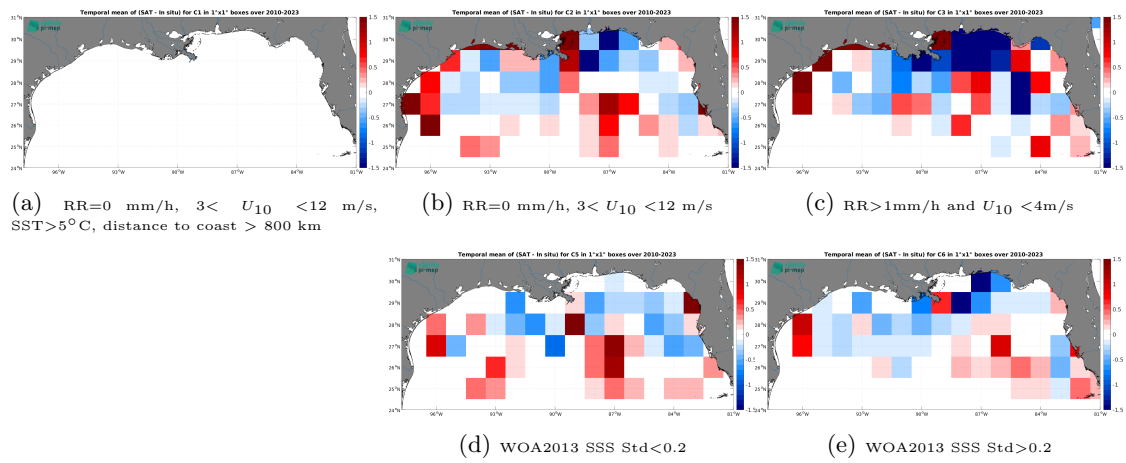
Figure 14: Temporal mean gridded over spatial boxes of size 1^\circ \times 1^\circ of \Delta\text{SSS} (SMOS SSS L4 OI v346 - Weekly (CMEMS-CATDS-LOPS) - TSG (SAMOS)) for 5 different subdatasets corresponding to: RR=0 mm/h, 3 < U_{10} < 12 m/s, SST > 5°C, distance to coast > 800 km (a), RR=0 mm/h, 3 < U_{10} < 12 m/s (b), RR > 1 mm/h and U_{10} < 4 m/s (c), WOA2013 SSS Std < 0.2 (d), WOA2013 SSS Std > 0.2 (e).
