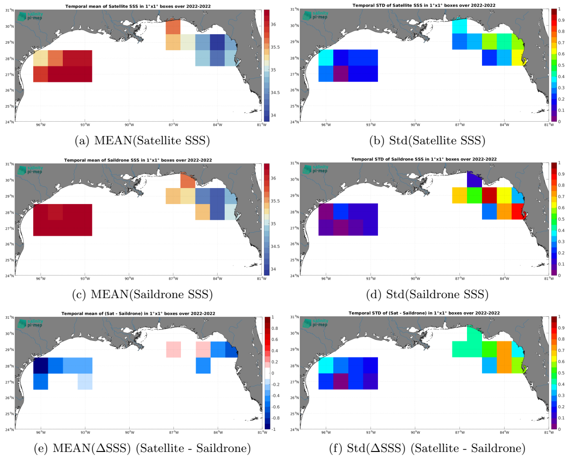
Figure 7: Temporal mean (left) and Std (right) of SSS from SMOS SSS L4 OI v346 - Weekly (CMEMS-CATDS-LOPS) (top), Saildrone (middle), and of \Delta SSS (Satellite - Saildrone). Only match-up pairs are used to generate these maps.
