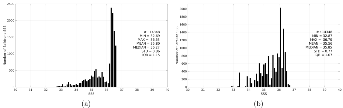
Figure 3: Histograms of SSS from Sailldrone (a) and SMOS SSS L4 OI v346 - Weekly (CMEMS-CATDS-LOPS) (b) considering all match-up pairs per bins of 0.1 over the Mississippi river plume Pi-MEP region and for the full satellite product period.
