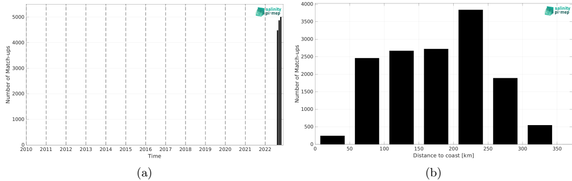
Figure 2: Number of match-ups between Sailldrone and SMOS SSS L4 OI v346 - Weekly (CMEMS-CATDS-LOPS) SSS as a function of time (a) and as function of the distance to coast (b) over the Mississippi river plume Pi-MEP region and for the full satellite product period.
