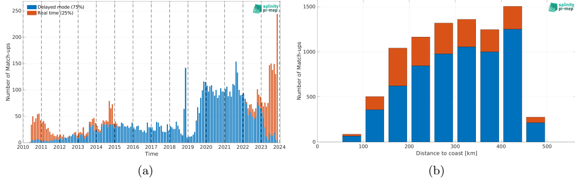
Figure 2: Number of match-ups between Argo and SMOS SSS L4 OI v346 - Weekly (CMEMS-CATDS-LOPS) SSS as a function of time (a) and as function of the distance to coast (b) over the Mississippi river plume Pi-MEP region and for the full satellite product period.
