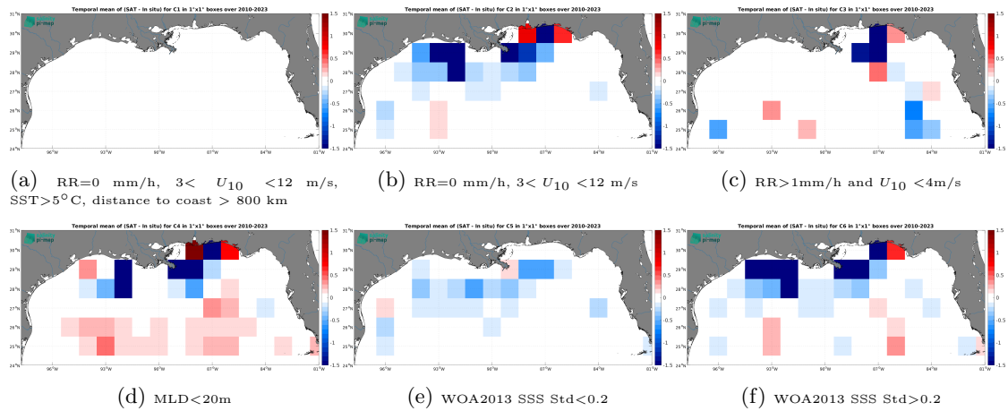
Figure 14: Temporal mean gridded over spatial boxes of size 1^\circ \times 1^\circ of \Delta SSS (SMOS SSS L4 OI v346 - Weekly (CMEMS-CATDS-LOPS) - Argo) for 6 different subdatasets corresponding to:RR=0 mm/h, 3 < U_{10} < 12 m/s, SST >5^\circ C, distance to coast > 800 km (a), RR=0 mm/h, 3 < U_{10} < 12 m/s (b), RR >1 mm/h and U_{10} < 4 m/s (c),MLD <20 m (d),WOA2013 SSS Std <0.2 (e),WOA2013 SSS Std >0.2 (f).
