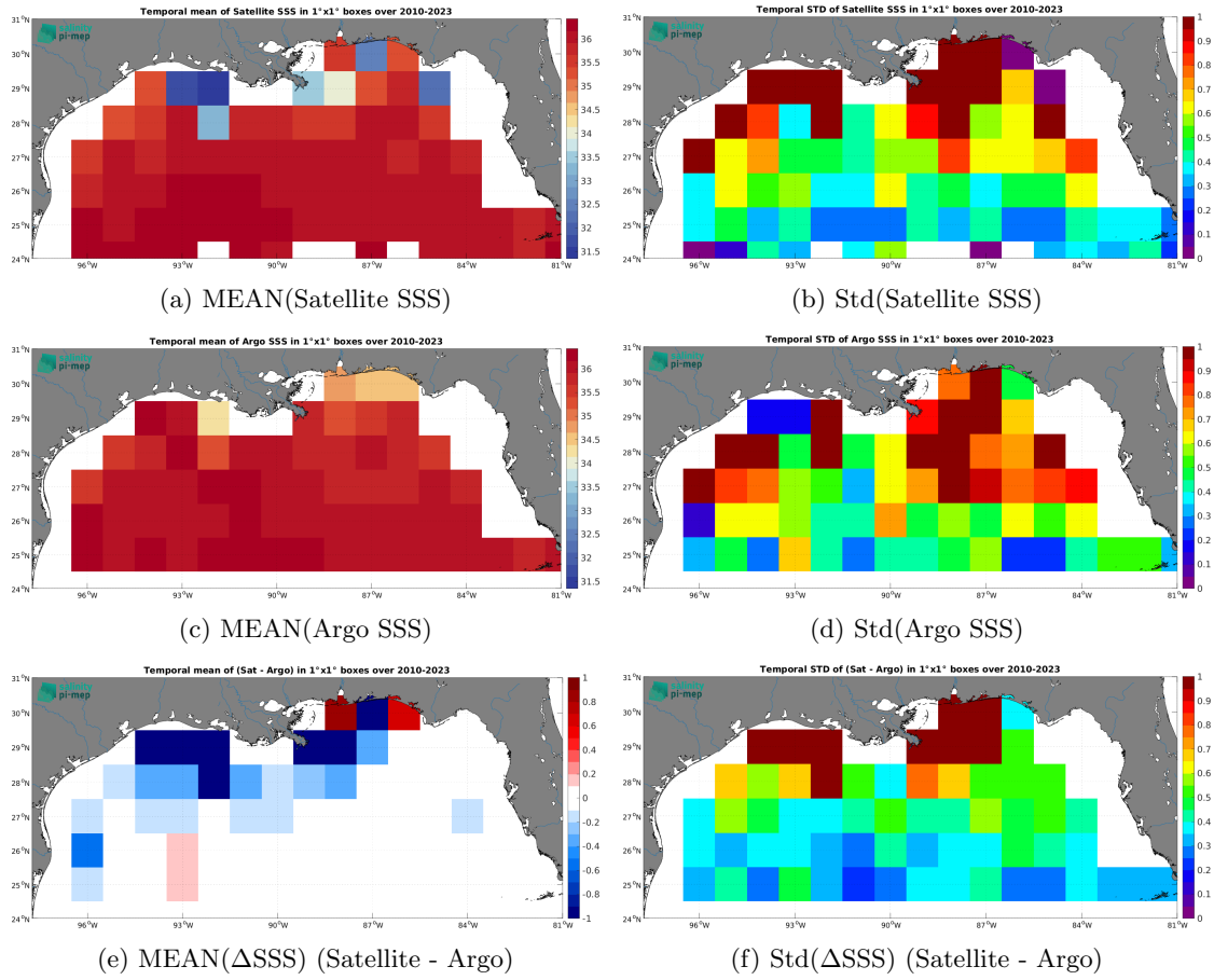
Figure 7: Temporal mean (left) and Std (right) of SSS from SMOS SSS L4 OI v346 - Weekly (CMEMS-CATDS-LOPS) (top), Argo (middle), and of \Delta SSS (Satellite - Argo). Only match-up pairs are used to generate these maps.
