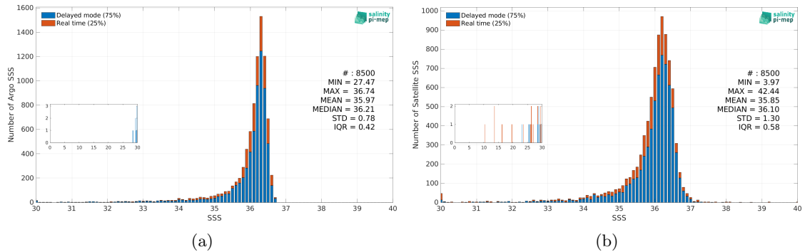
Figure 3: Histograms of SSS from Argo (a) and SMOS SSS L4 OI v346 - Weekly (CMEMS-CATDS-LOPS) (b) considering all match-up pairs per bins of 0.1 over the Mississippi river plume Pi-MEP region and for the full satellite product period.
