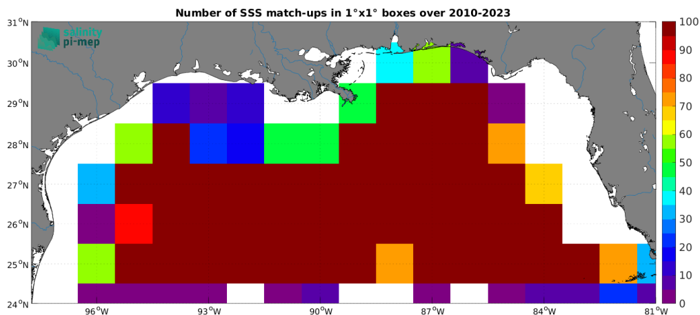
Figure 5: Number of SSS match-ups between Argo SSS and the SMOS SSS L4 OI v346 - Weekly (CMEMS-CATDS-LOPS) SSS product for the Mississippi river plume Pi-MEP region over 1^\circ \times 1^\circ boxes and for the full satellite product period.
